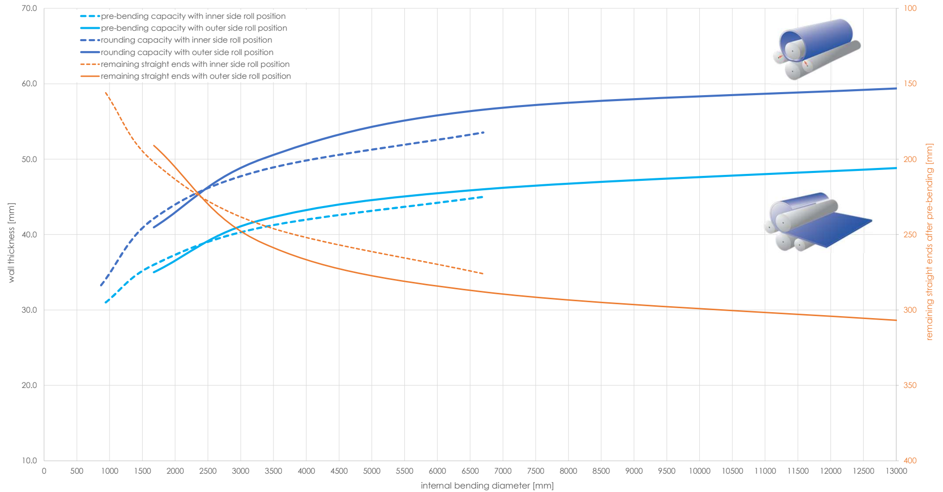
Capacity graph EVO 41513 - Yield point 690 N/mm 2 (calculated plate width 4'000 mm)
