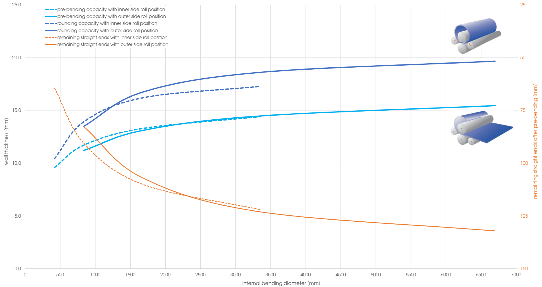
Capacity graph EVO 26071 - Yield point 690 N/mm 2 (calculated plate width 2'500 mm)
