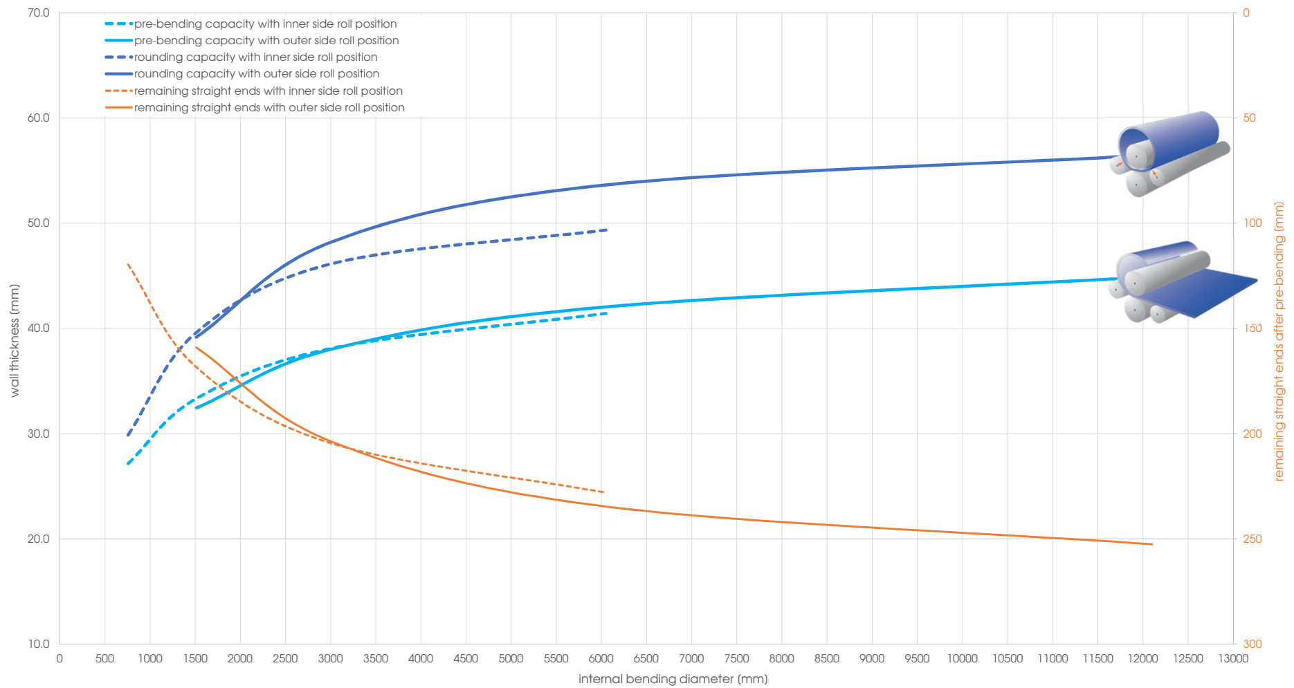
Capacity graph EVO 31385 - Yield point 690 N/mm 2 (calculated plate width 3'000 mm)
