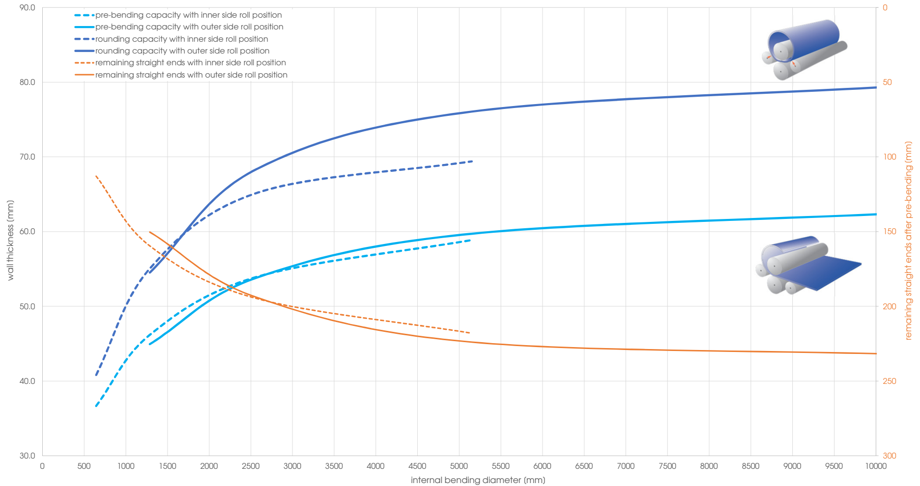
Capacity graph EVO 26283 - Yield point 260 N/mm 2 (calculated plate width 2'500 mm)
