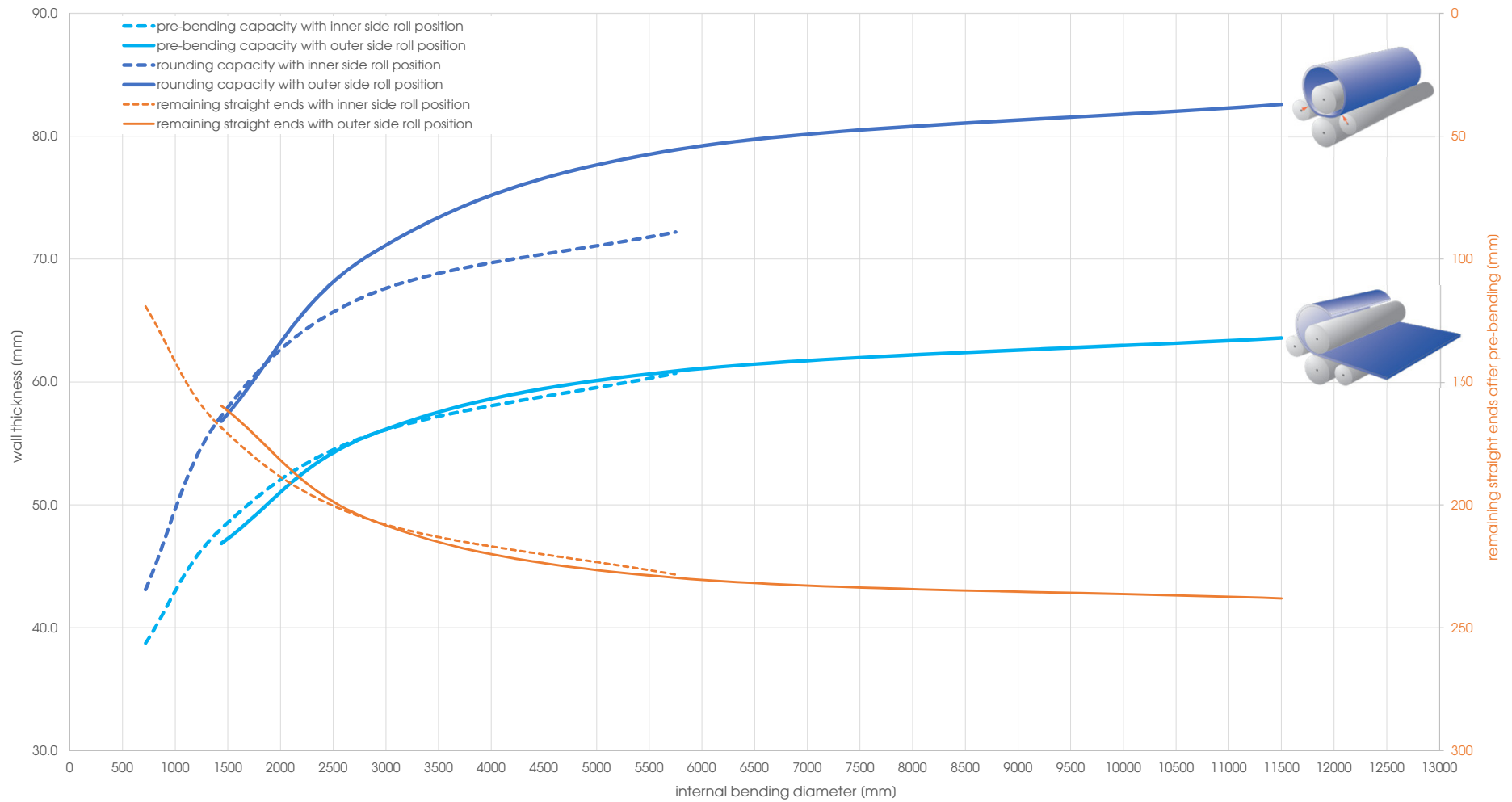
Capacity graph EVO 26385 - Yield point 360 N/mm 2 (calculated plate width 2'500 mm)
