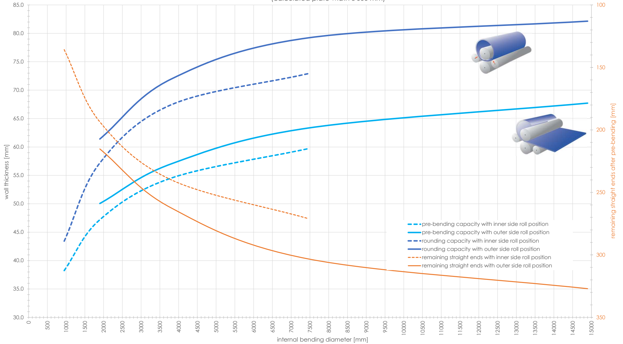
Capacity graph EVO 31680 - Yield point 690 N/mm 2 (calculated plate width 3'000 mm)
