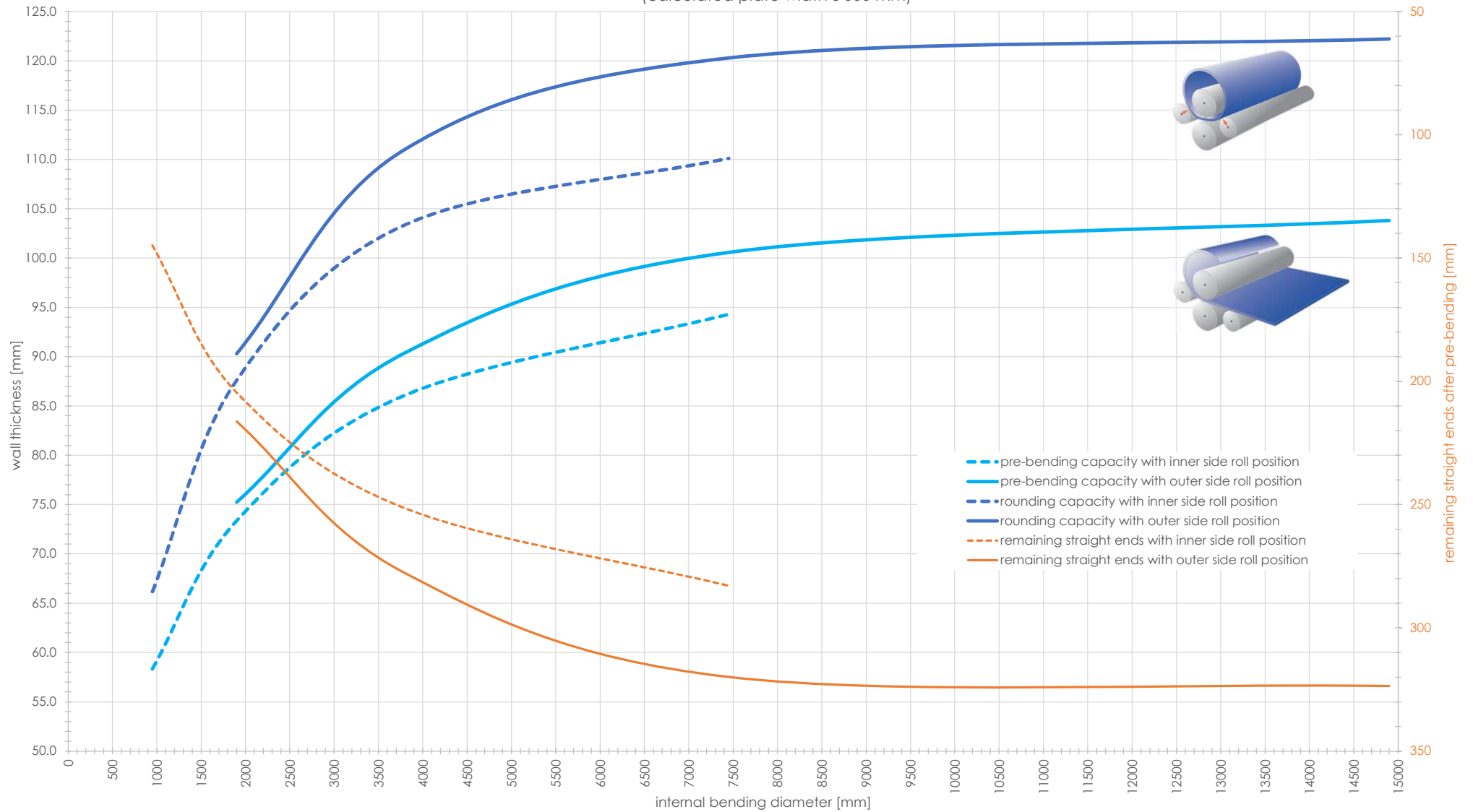
Capacity graph EVO 31680 - Yield point 260 N/mm 2 (calculated plate width 3'000 mm)
