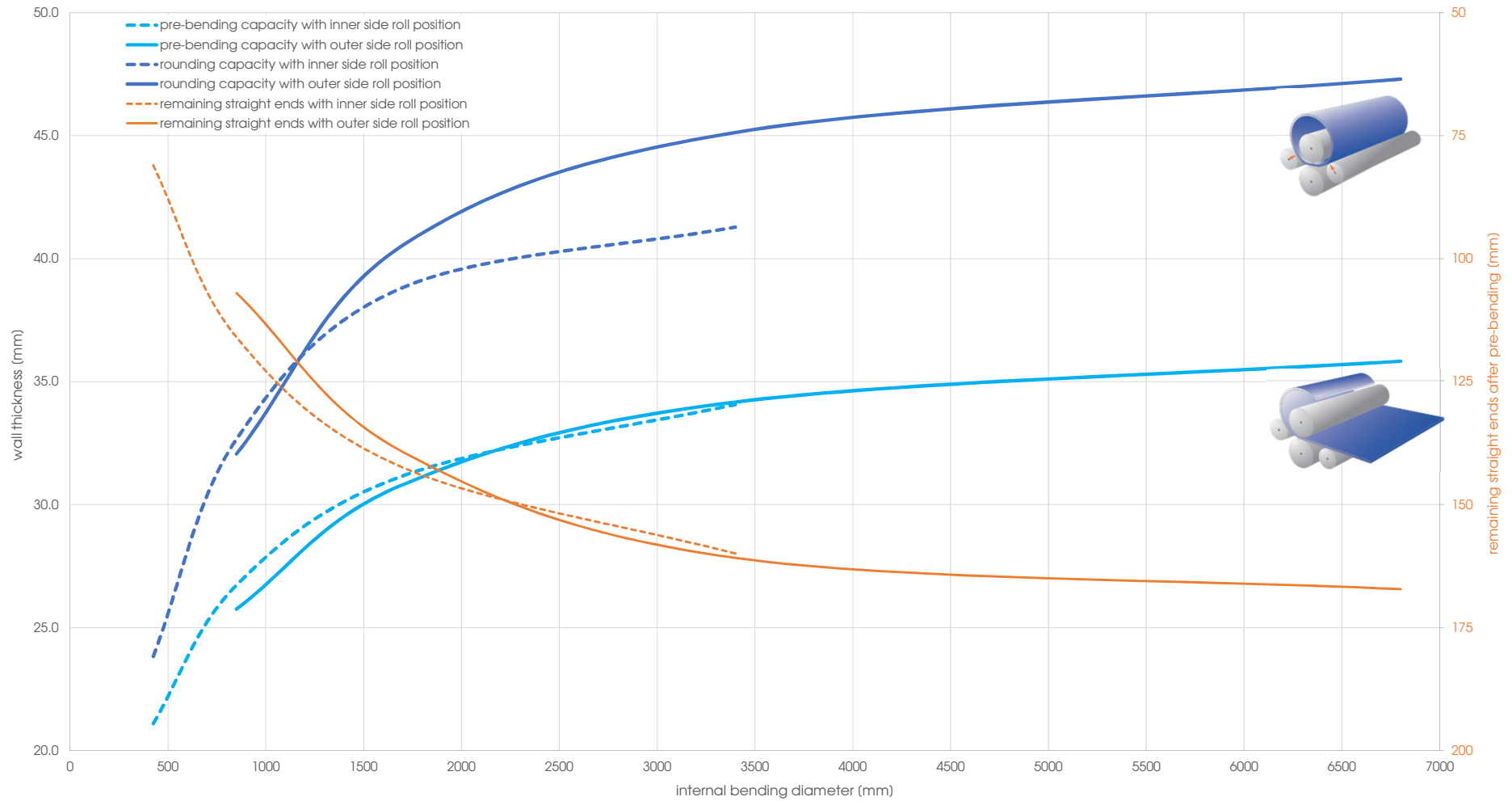
Capacity graph EVO 21102 - Yield point 260 N/mm 2 (calculated plate width 2'000 mm)
