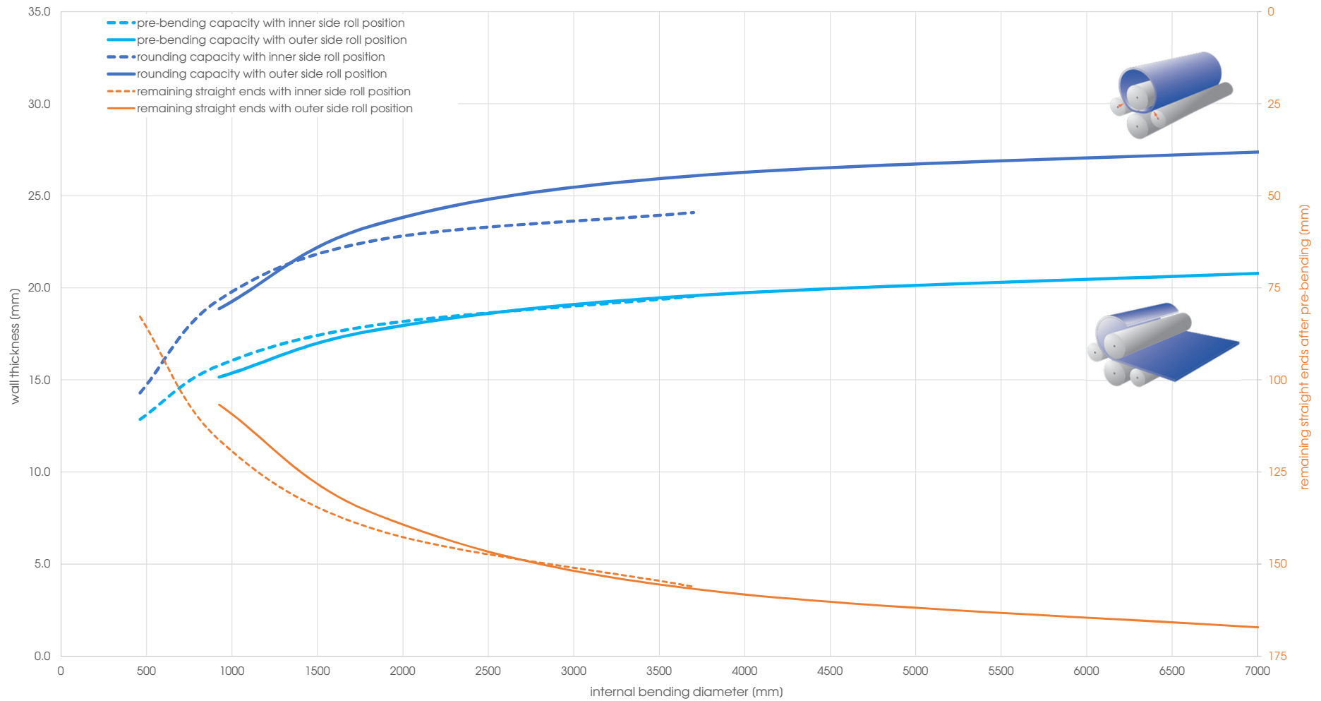
Capacity graph EVO 26102 - Yield point 690 N/mm 2 (calculated plate width 2'500 mm)
