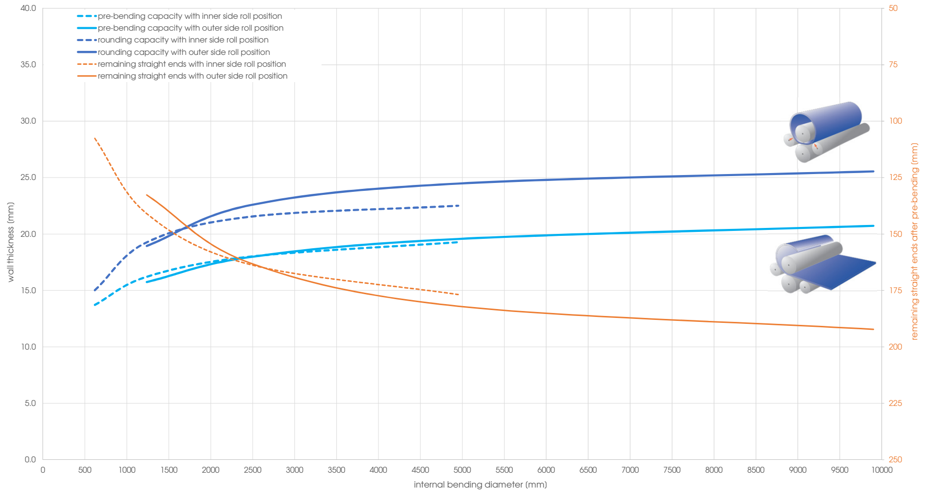
Capacity graph EVO 41139 - Yield point 690 N/mm 2 (calculated plate width 4'000 mm)
