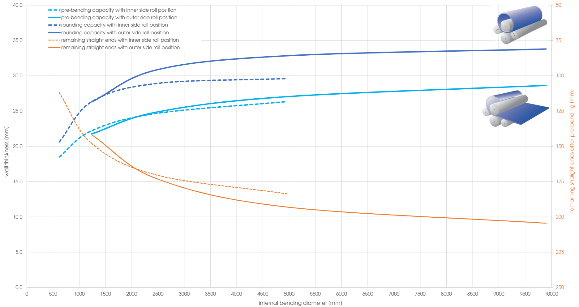
Capacity graph EVO 41139 - Yield point 360 N/mm 2 (calculated plate width 4'000 mm)
