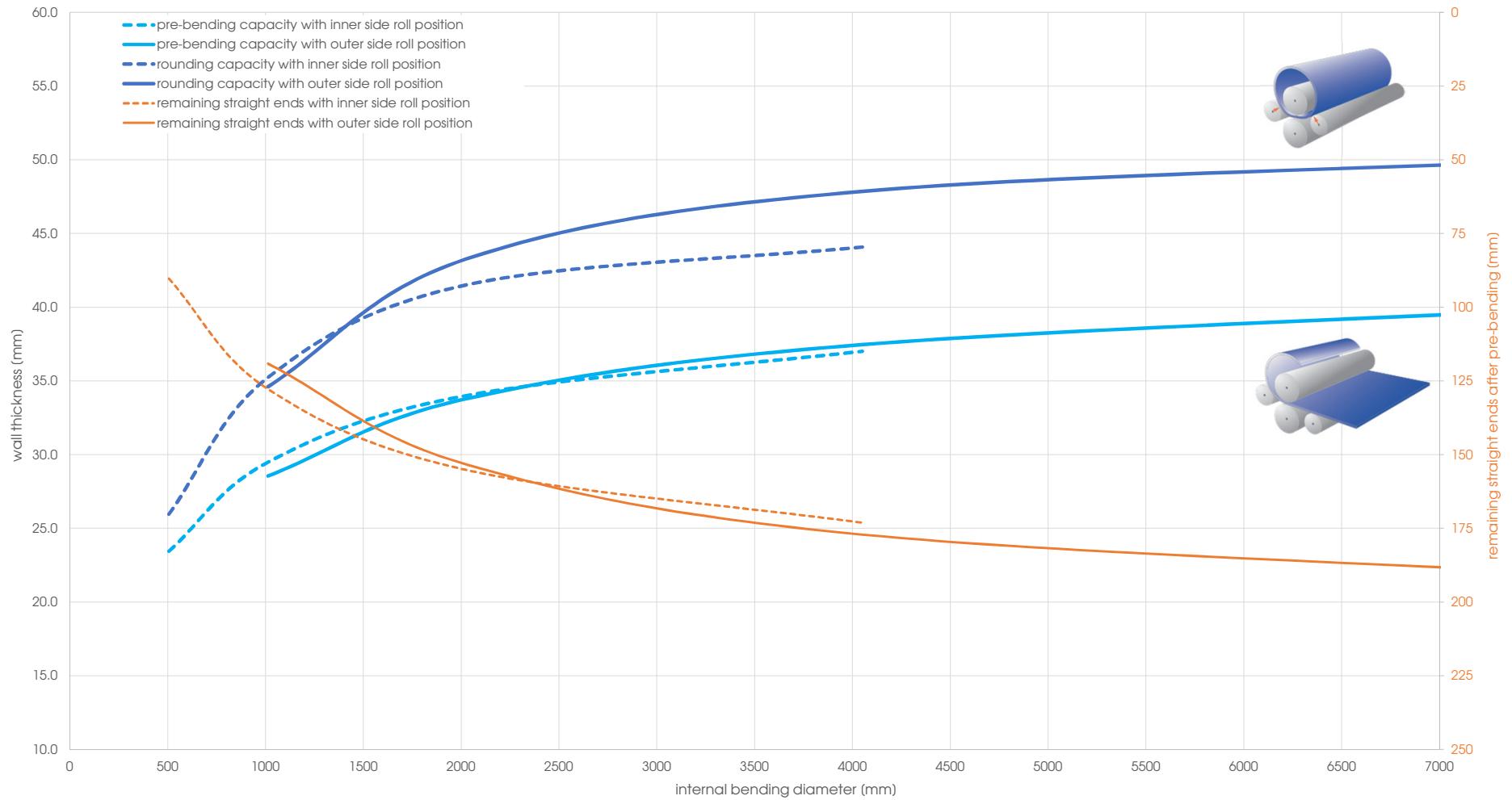
Capacity graph EVO 26139 - Yield point 260 N/mm 2 (calculated plate width 2'500 mm)
