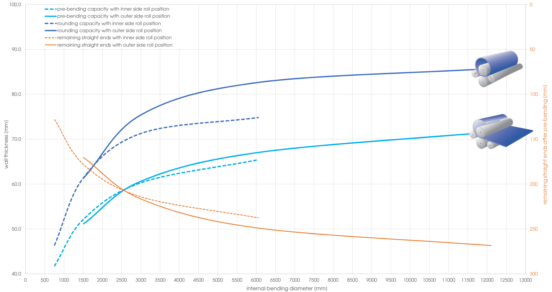
Capacity graph EVO 31385 - Yield point 260 N/mm 2 (calculated plate width 3'000 mm)
