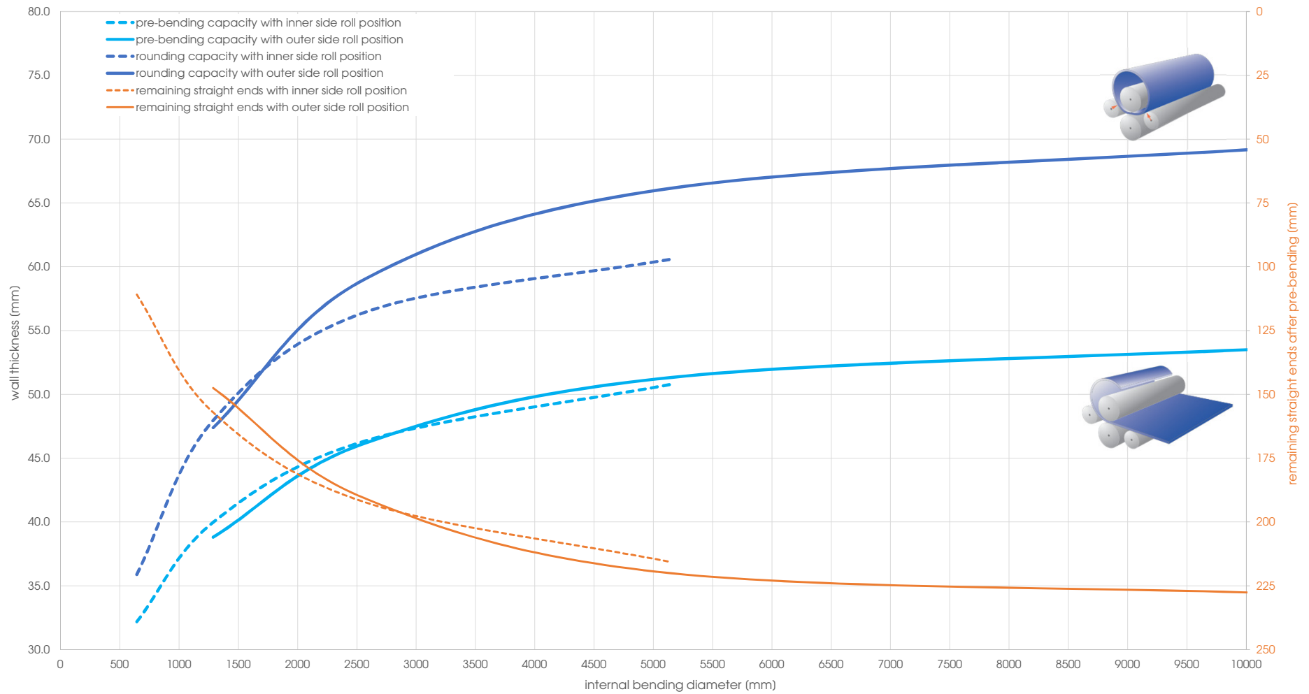
Capacity graph EVO 26283 - Yield point 360 N/mm 2 (calculated plate width 2'500 mm)
