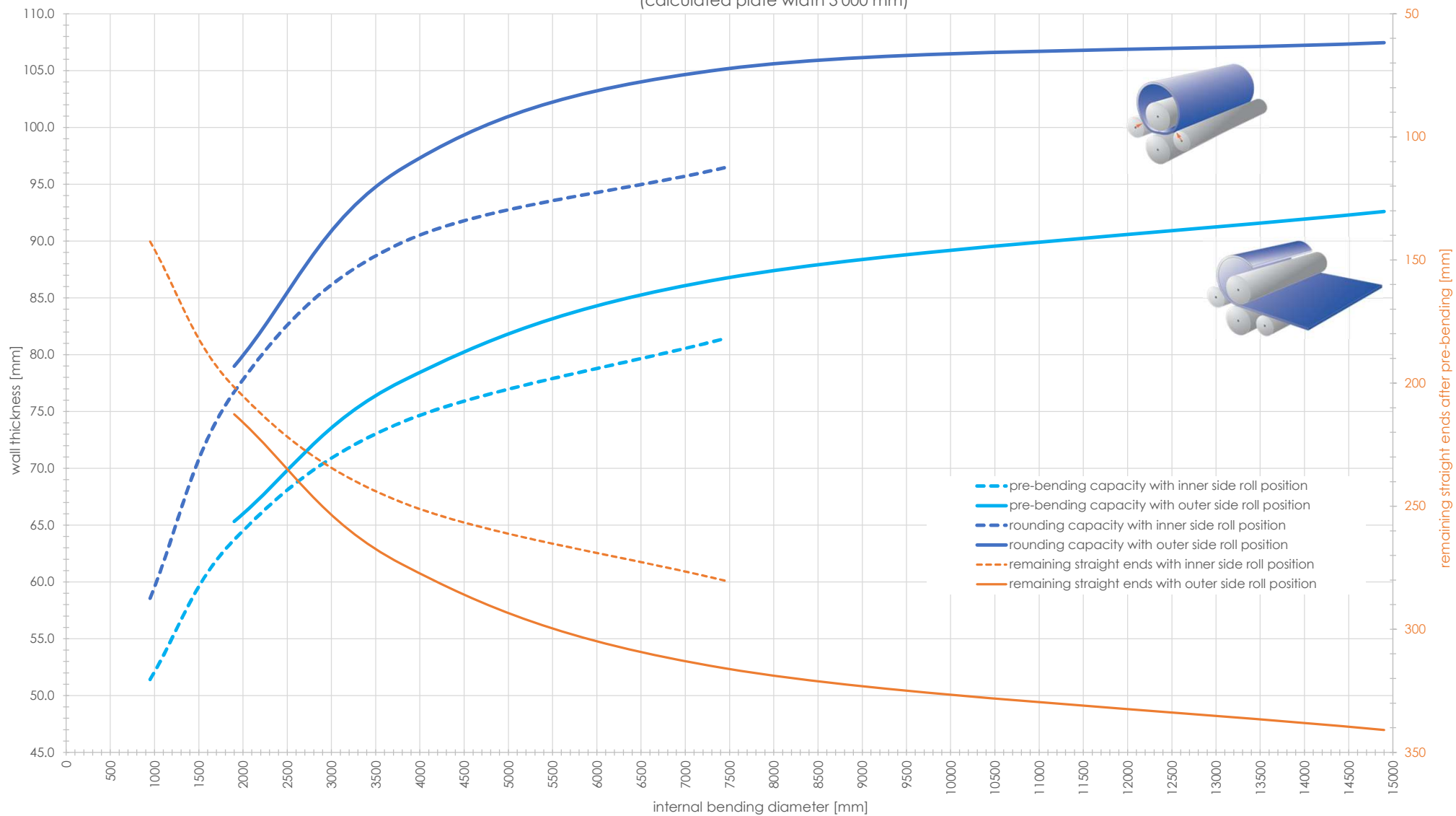
Capacity graph EVO 31680 - Yield point 360 N/mm 2 (calculated plate width 3'000 mm)
