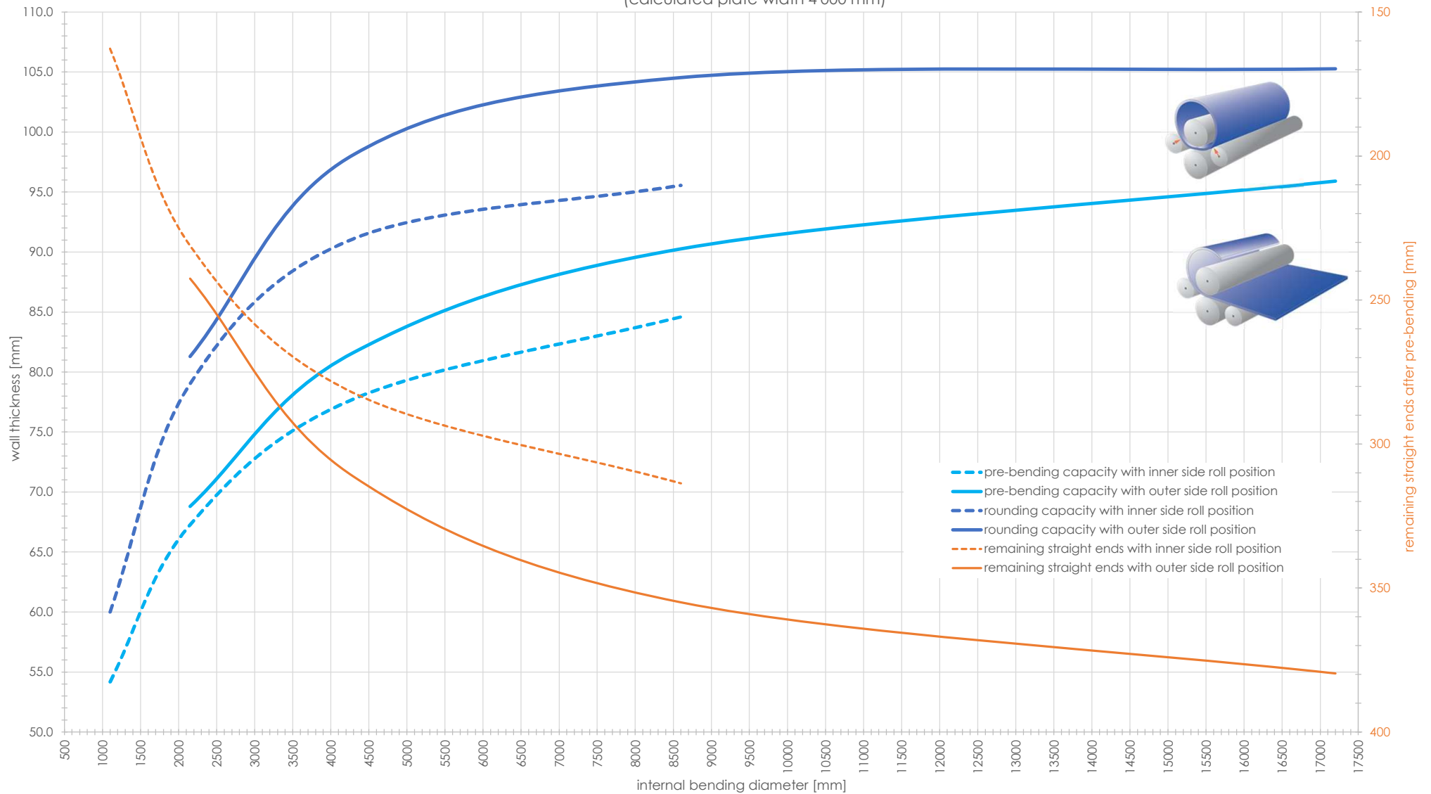
Capacity graph EVO 41871 - Yield point 360 N/mm 2 (calculated plate width 4'000 mm)
