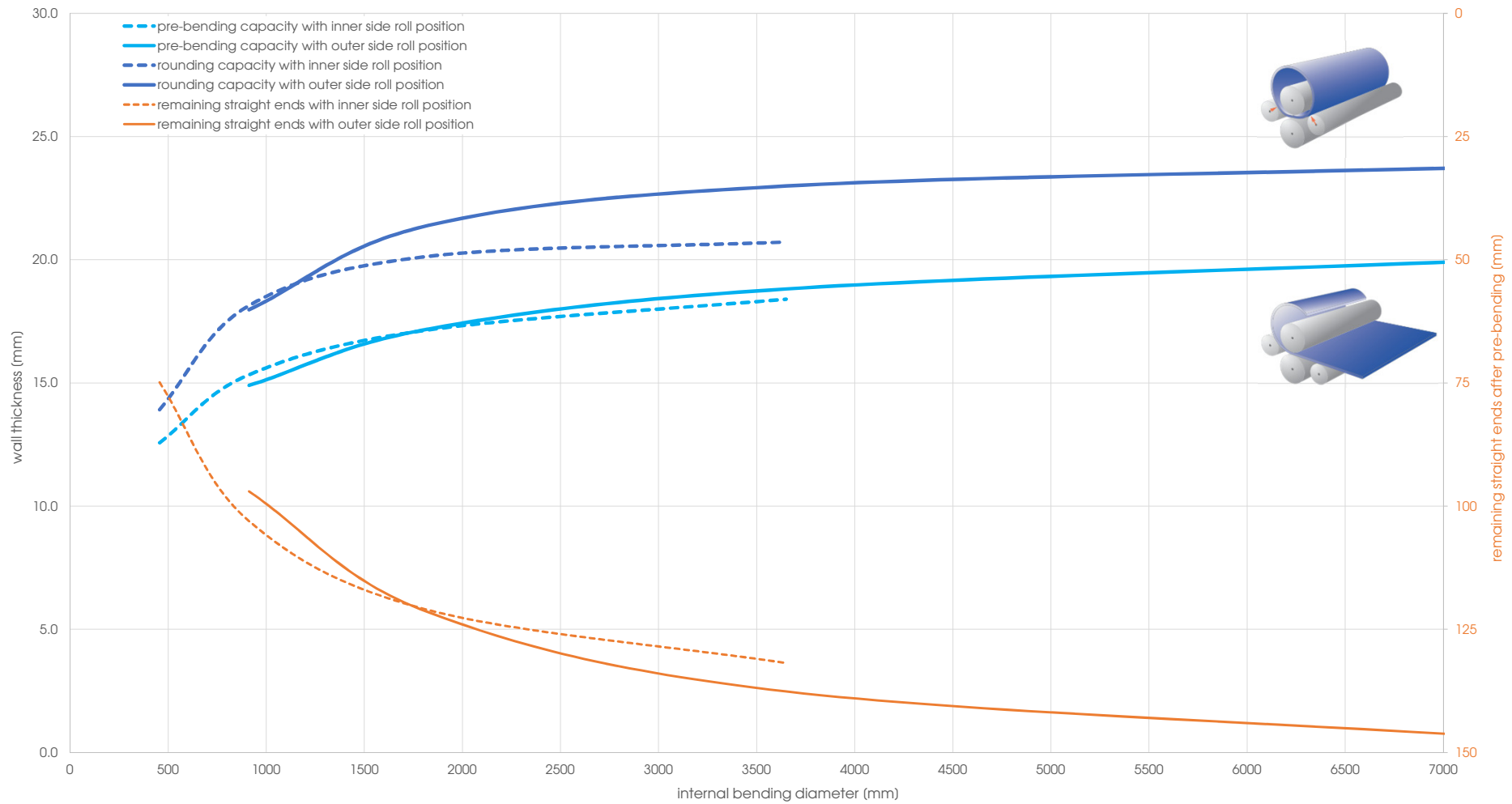
Capacity graph EVO 31071 - Yield point 360 N/mm 2 (calculated plate width 3'000 mm)
