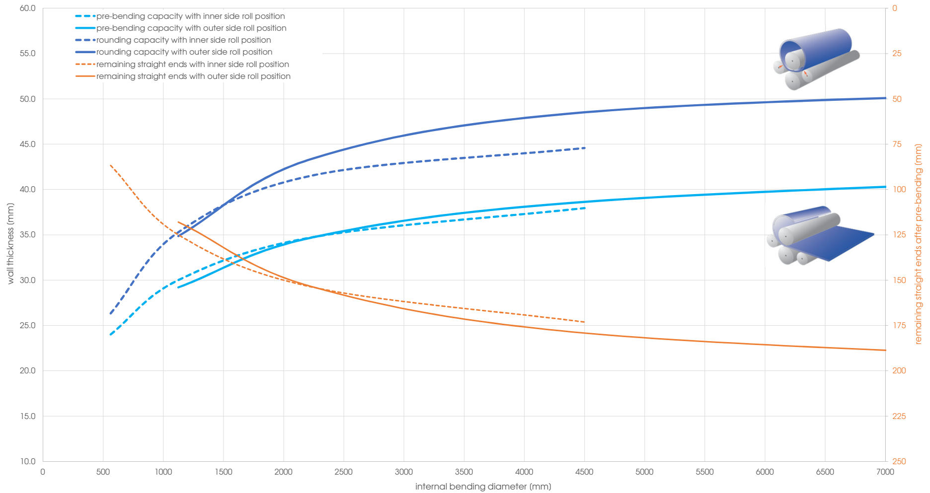
Capacity graph EVO 26196 - Yield point 360 N/mm 2 (calculated plate width 2'500 mm)
