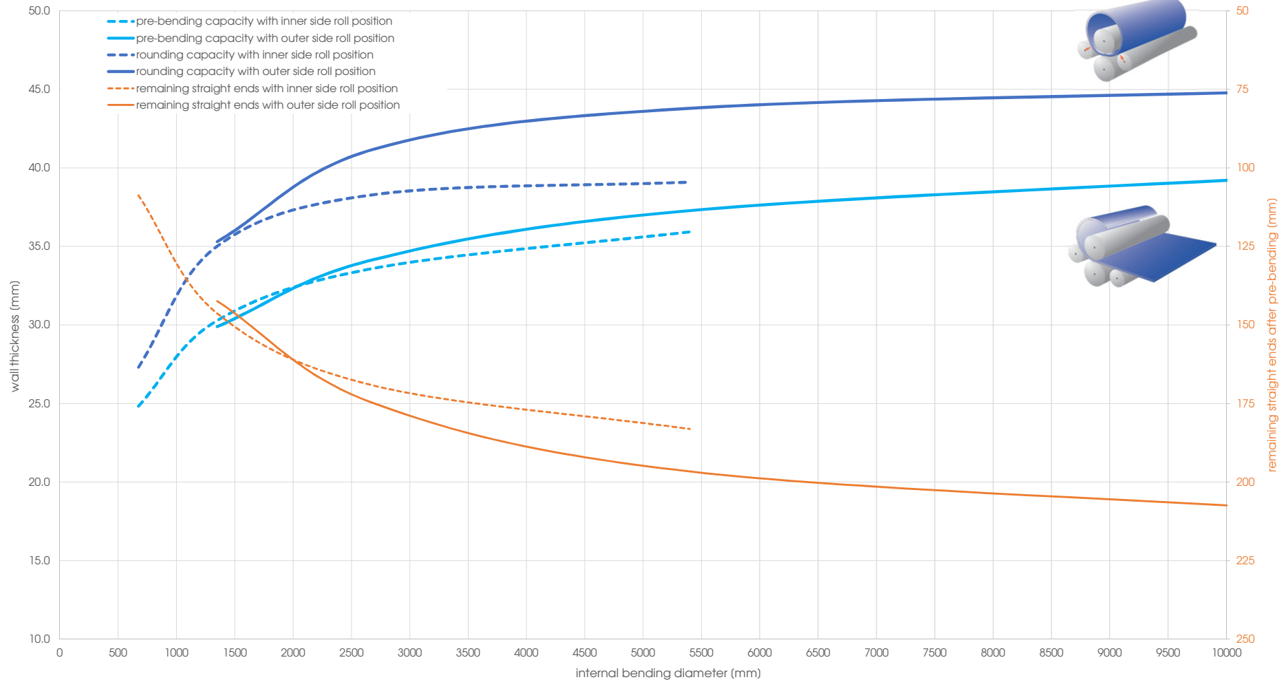
Capacity graph EVO 41196 - Yield point 260 N/mm 2 (calculated plate width 4'000 mm)
