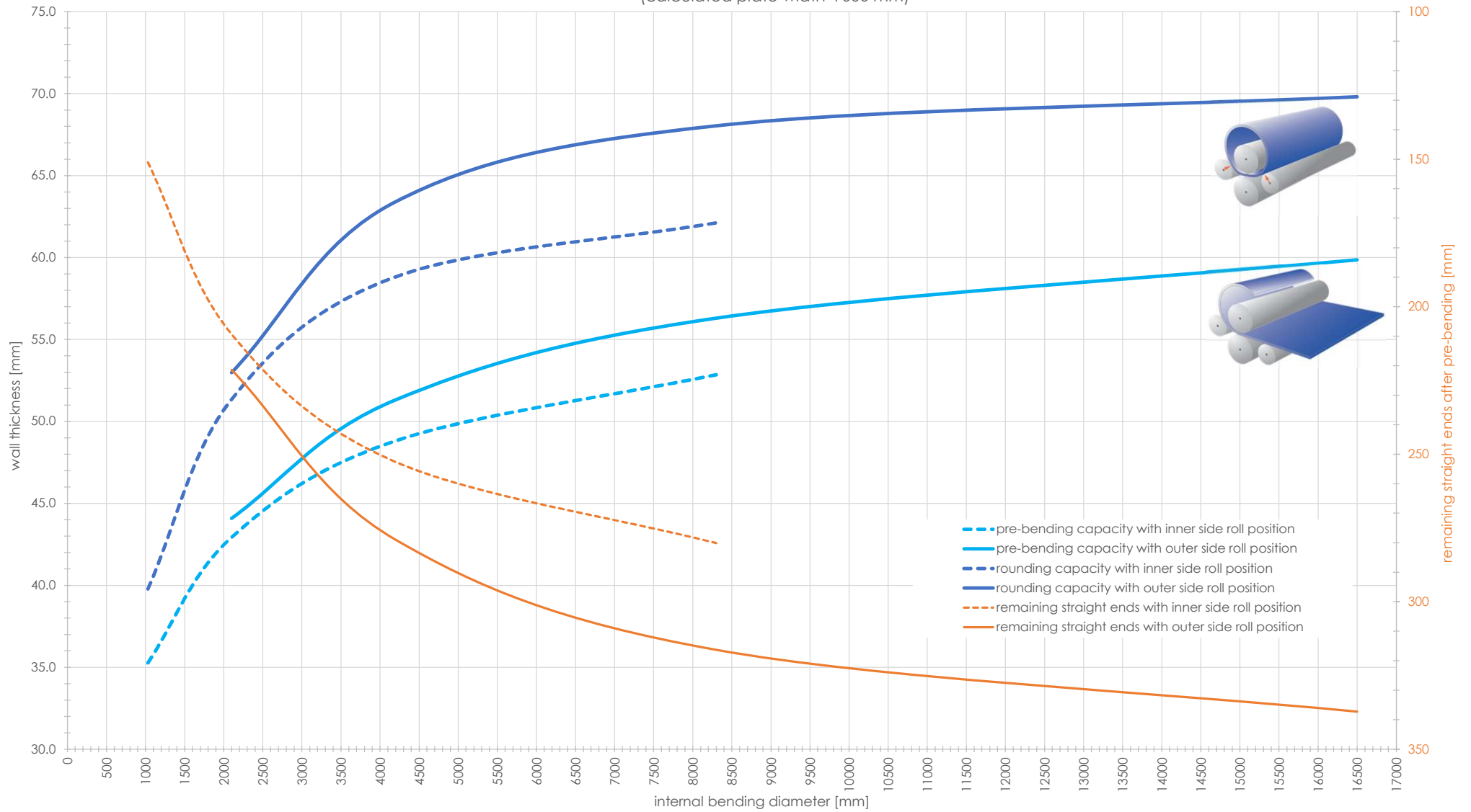
Capacity graph EVO 41680 - Yield point 690 N/mm 2 (calculated plate width 4'000 mm)
