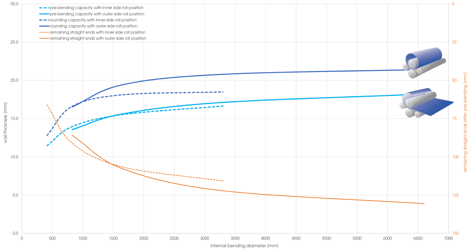
Capacity graph EVO 31049 - Yield point 260 N/mm 2 (calculated plate width 3'000 mm)
