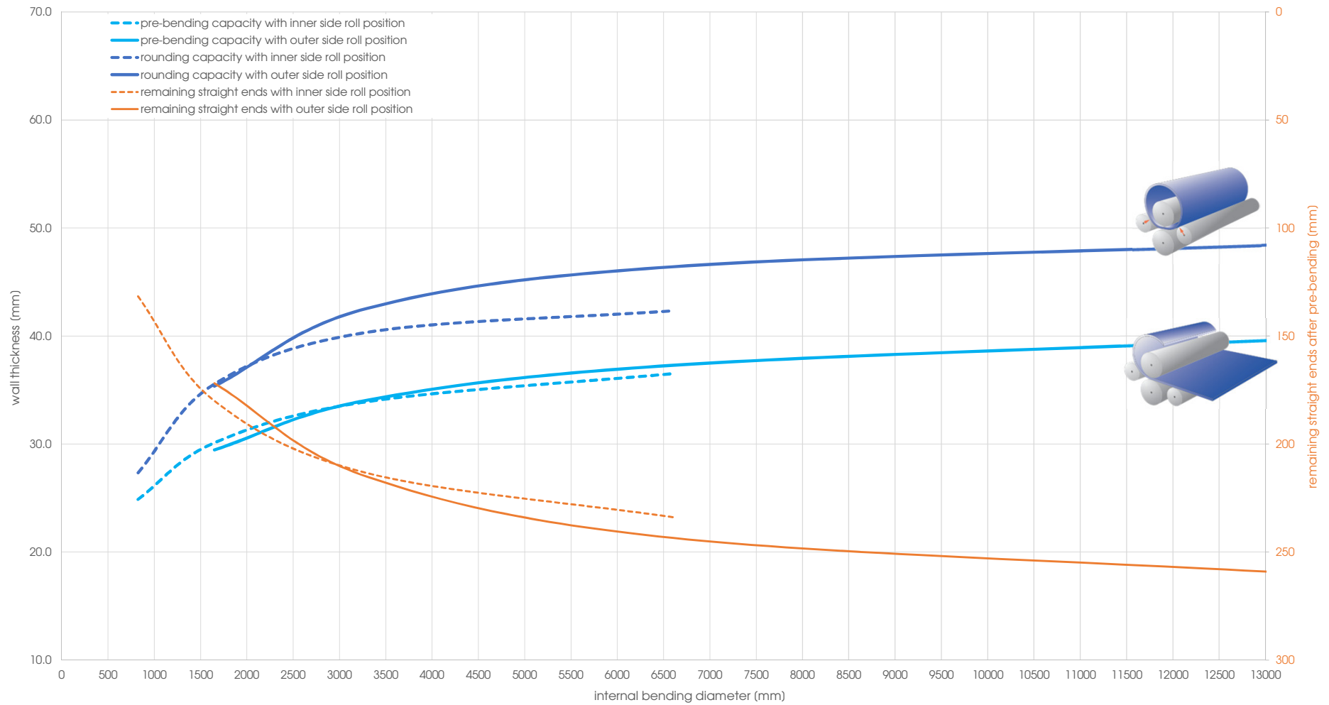
Capacity graph EVO 41385 - Yield point 690 N/mm 2 (calculated plate width 4'000 mm)
