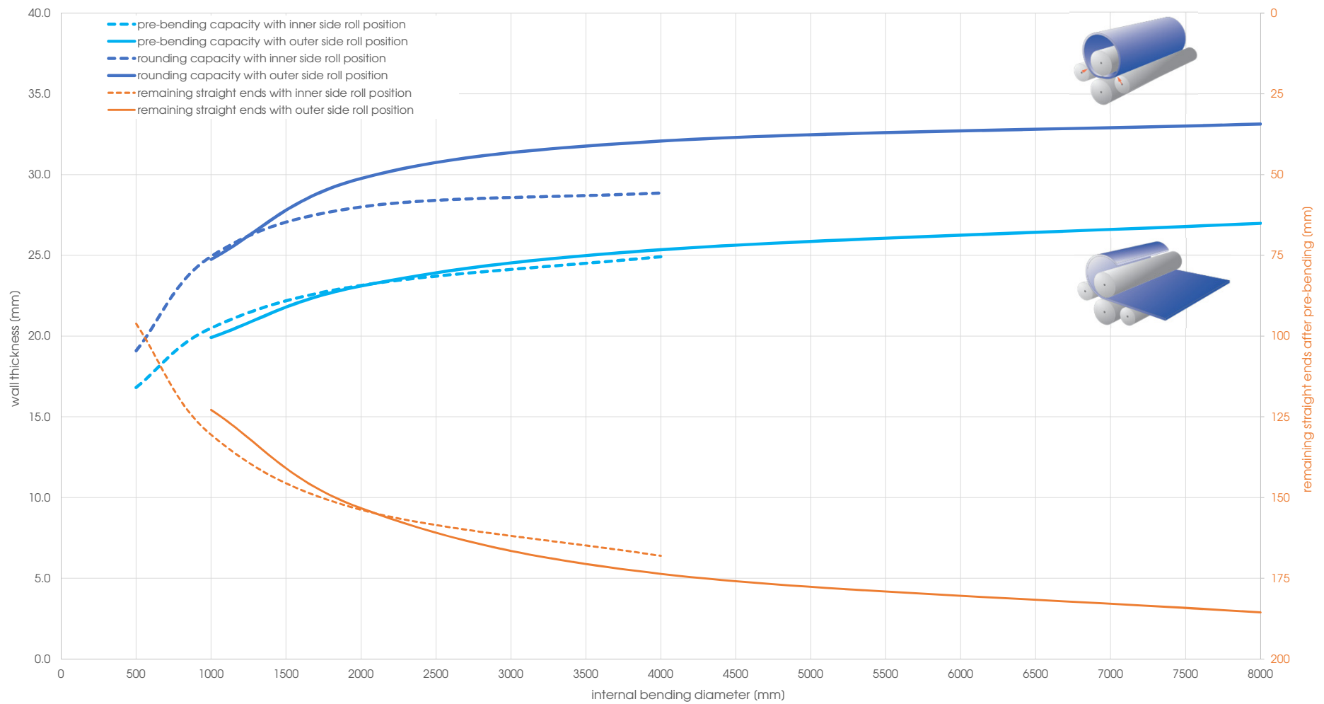
Capacity graph EVO 31102 - Yield point 360 N/mm 2 (calculated plate width 3'000 mm)
