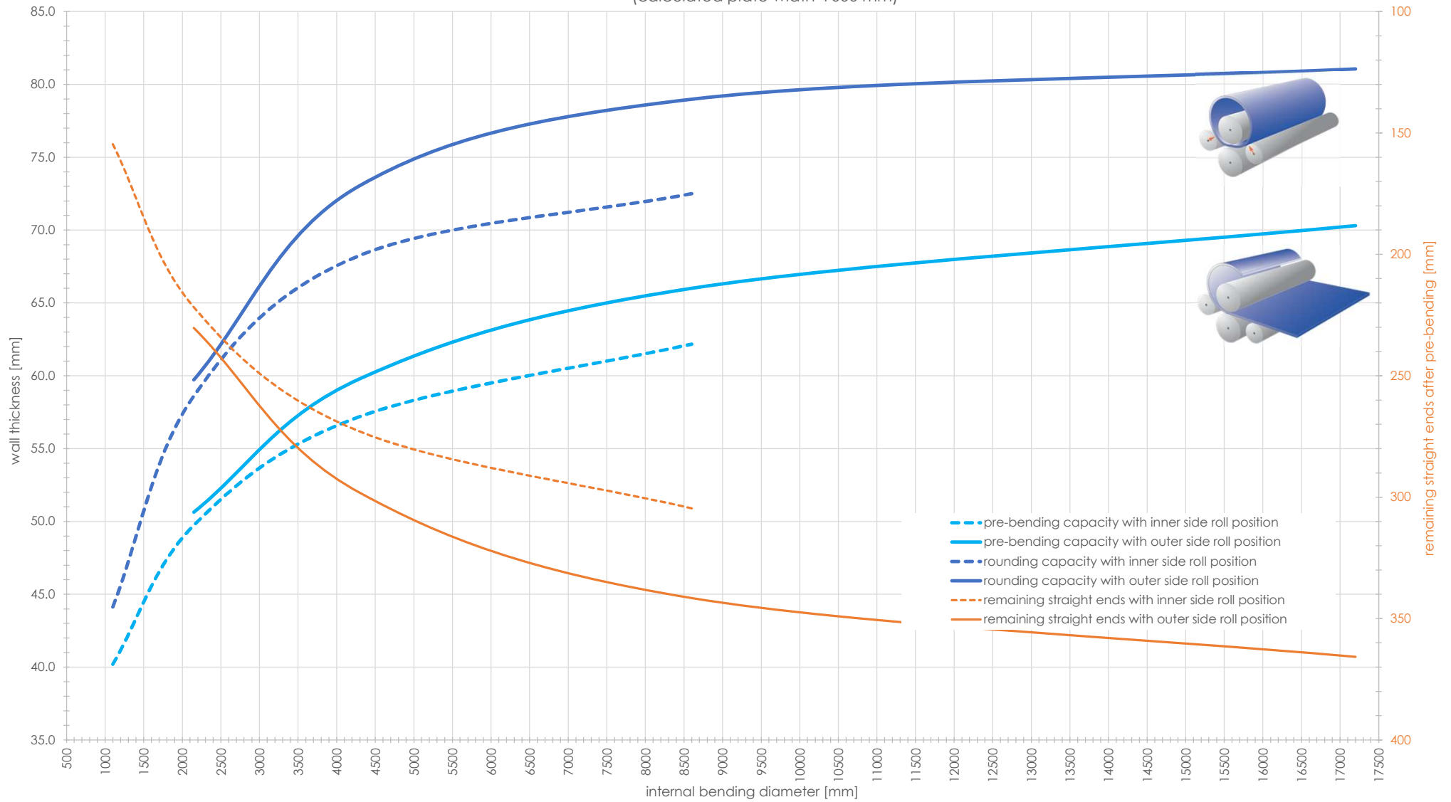
Capacity graph EVO 41871 - Yield point 690 N/mm 2 (calculated plate width 4'000 mm)
