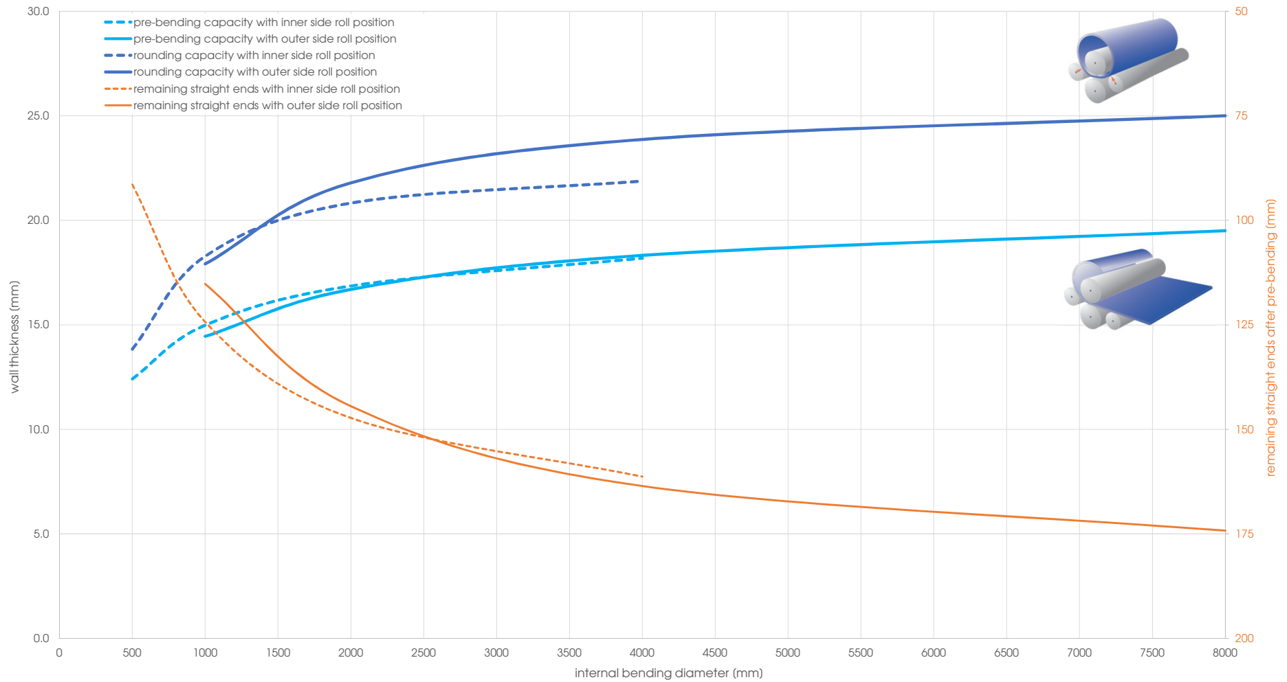
Capacity graph EVO 31102 - Yield point 690 N/mm 2 (calculated plate width 3'000 mm)
