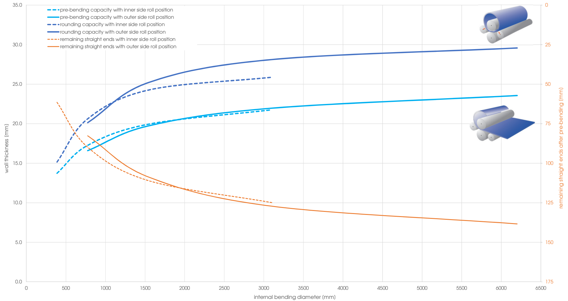
Capacity graph EVO 21071 - Yield point 360 N/mm 2 (calculated plate width 2'000 mm)
