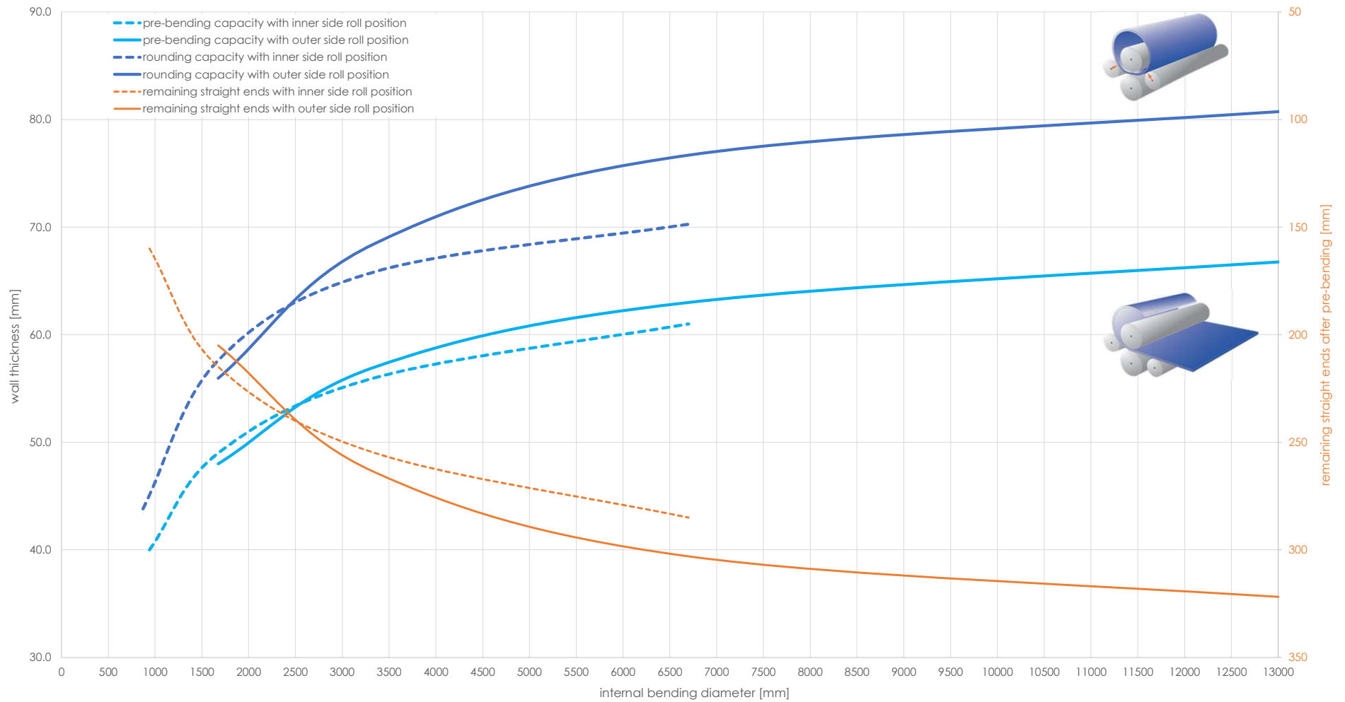
Capacity graph EVO 41513 - Yield point 360 N/mm 2 (calculated plate width 4'000 mm)
