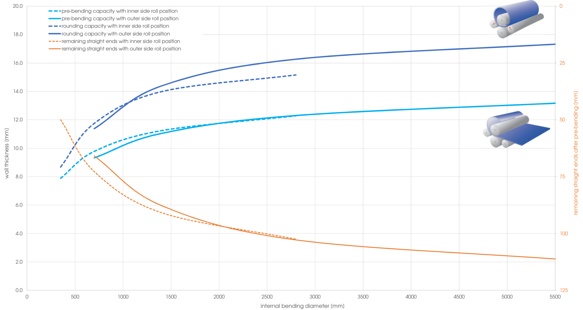
Capacity graph EVO 21049 - Yield point 690 N/mm 2 (calculated plate width 2'000 mm)
