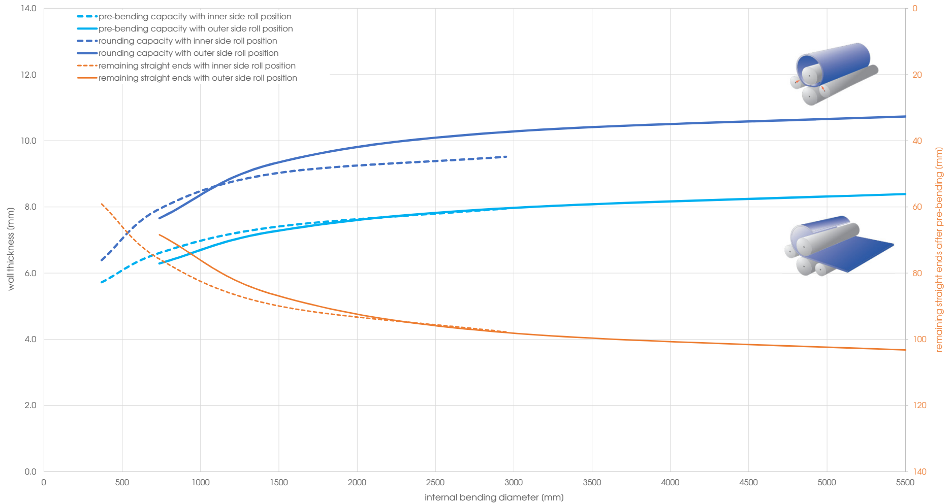
Capacity graph EVO 31031 - Yield point 690 N/mm 2 (calculated plate width 3'000 mm)
