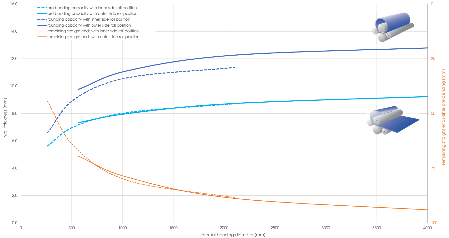
Capacity graph EVO 21015 - Yield point 360 N/mm 2 (calculated plate width 2'000 mm)
