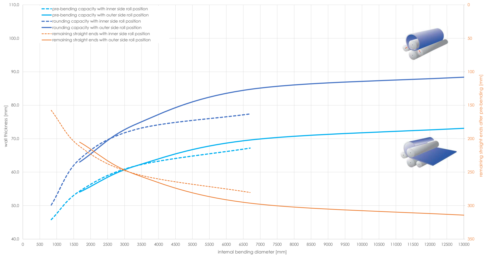
Capacity graph EVO 31513 - Yield point 360 N/mm 2 (calculated plate width 3'000 mm)
