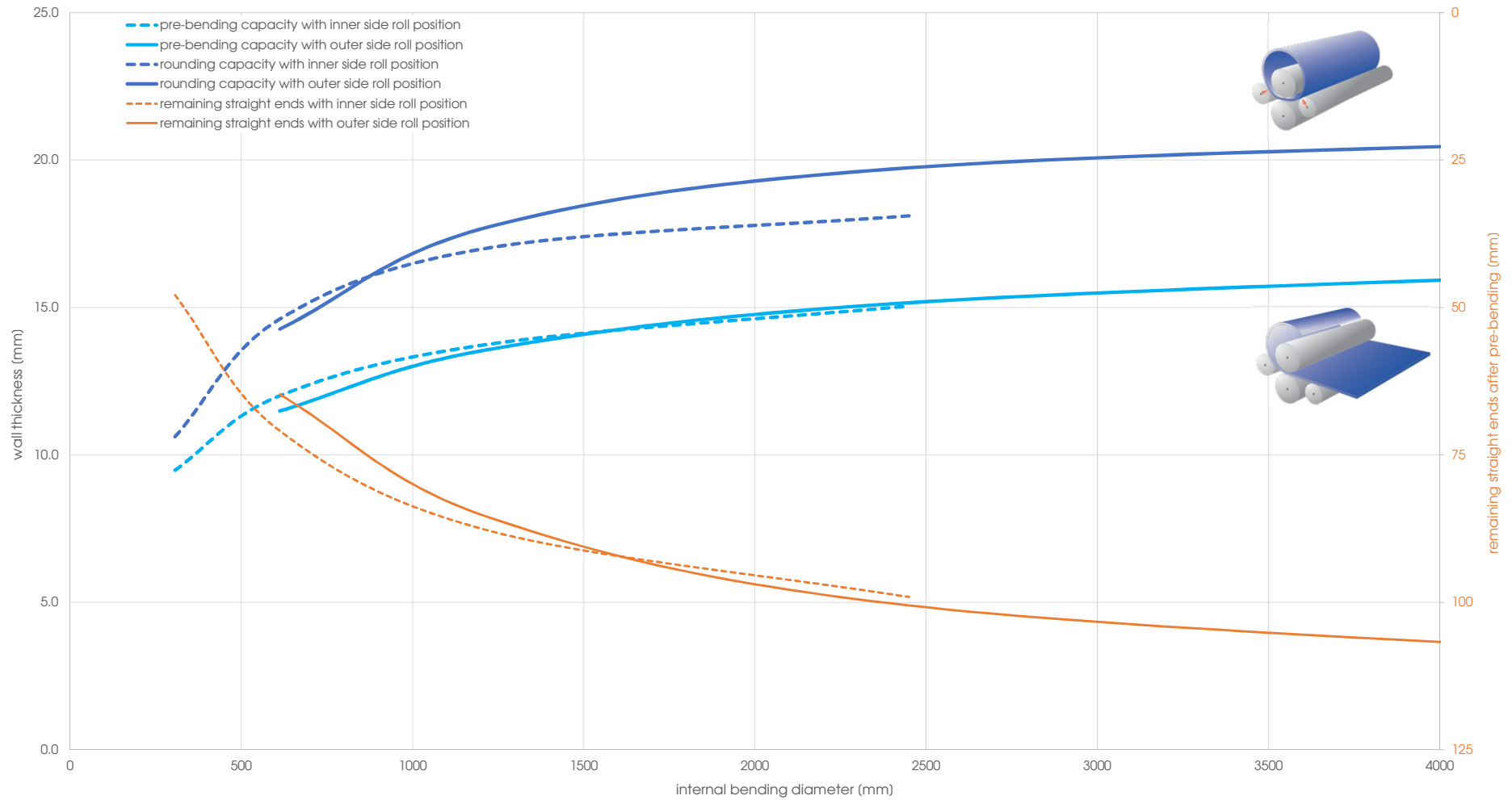
Capacity graph EVO 21031 - Yield point 260 N/mm 2 (calculated plate width 2'000 mm)
