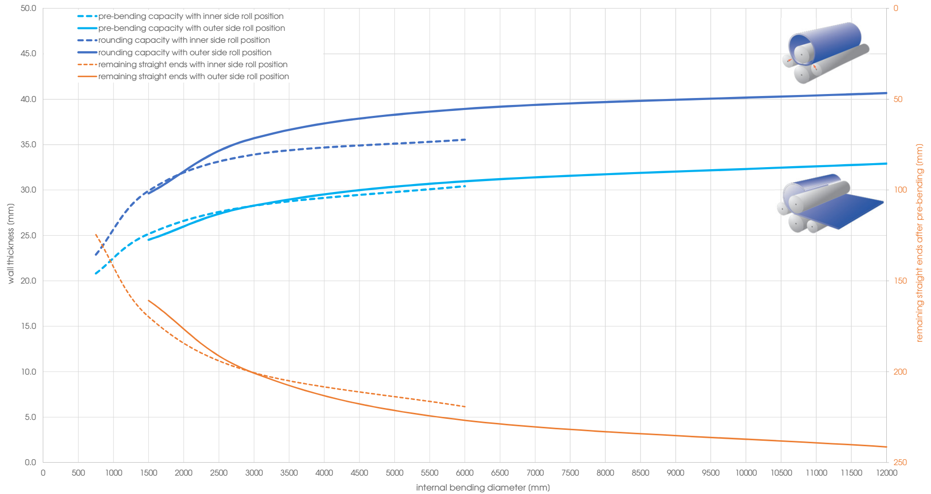
Capacity graph EVO 41283 - Yield point 690 N/mm 2 (calculated plate width 4'000 mm)
