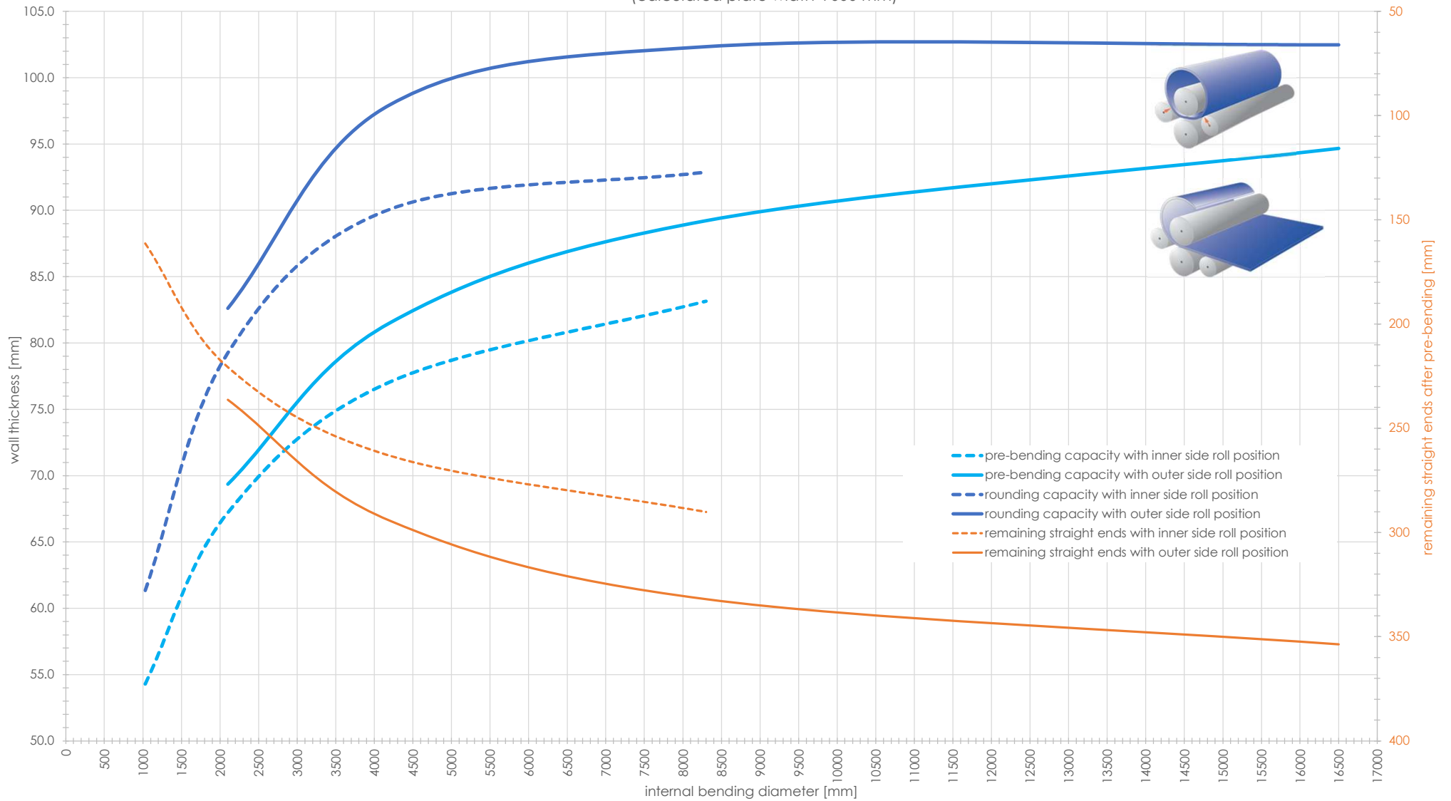
Capacity graph EVO 41680 - Yield point 260 N/mm 2 (calculated plate width 4'000 mm)
