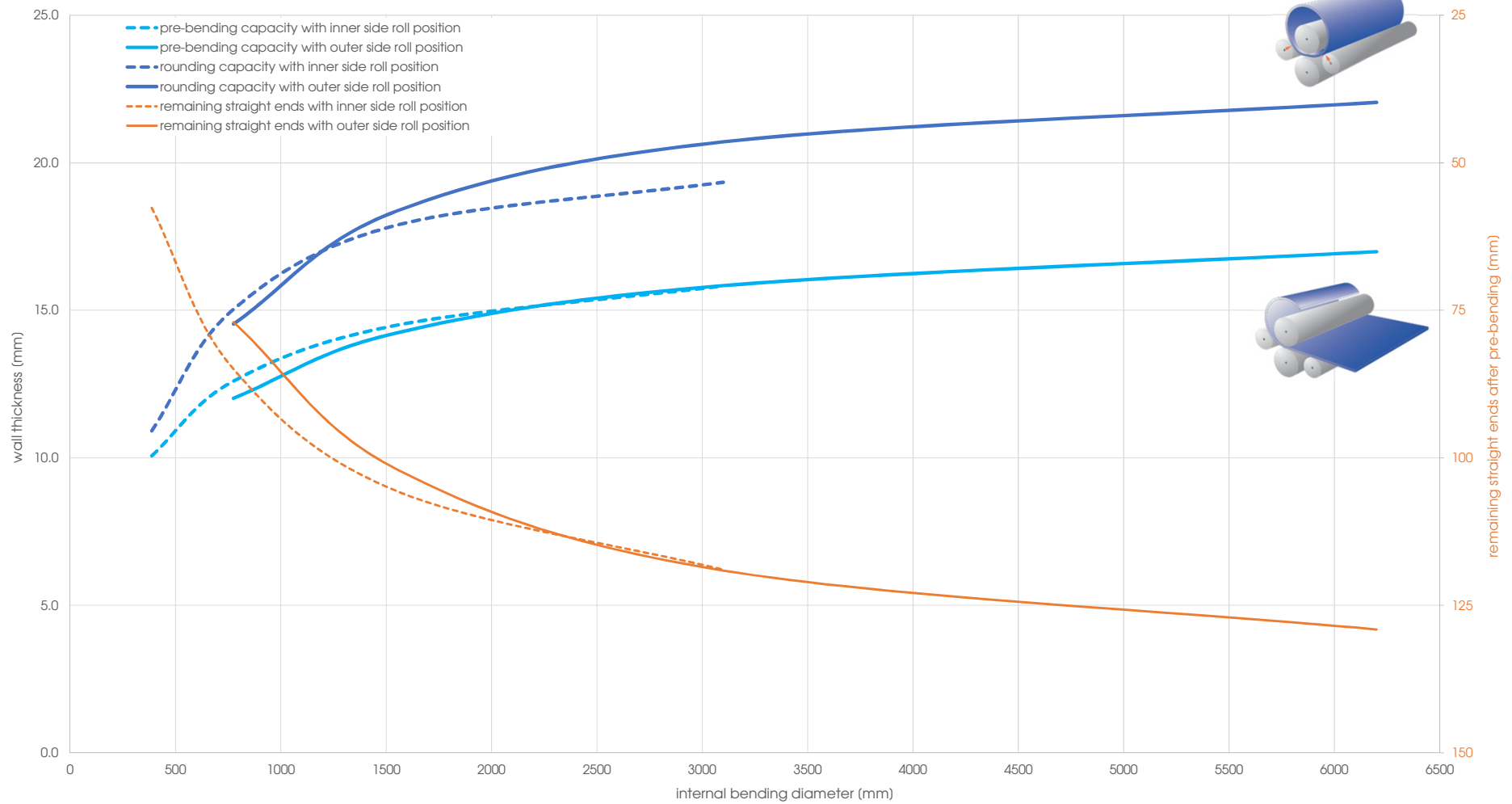
Capacity graph EVO 21071 - Yield point 690 N/mm 2 (calculated plate width 2'000 mm)
