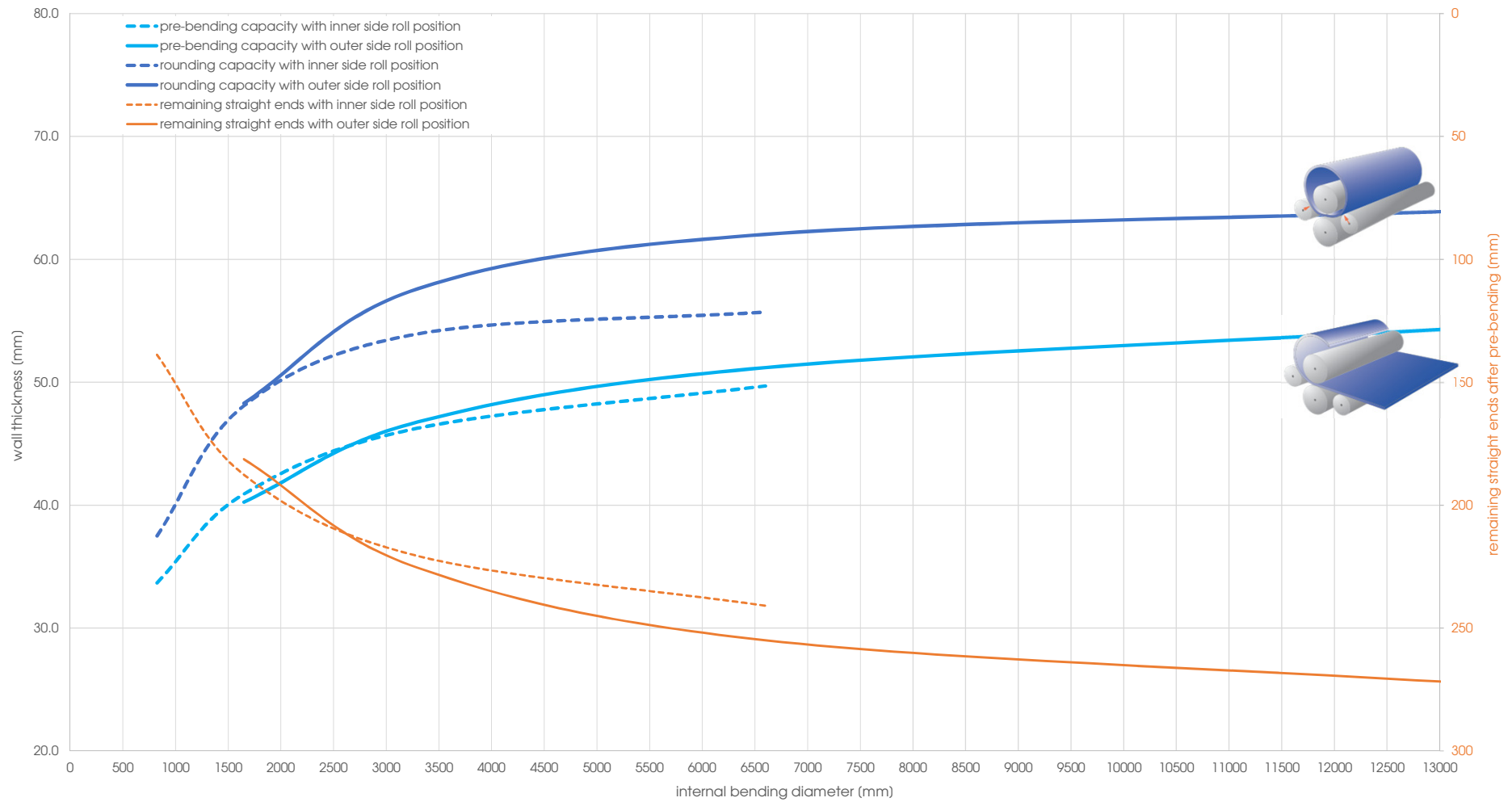
Capacity graph EVO 41385 - Yield point 360 N/mm 2 (calculated plate width 4'000 mm)
