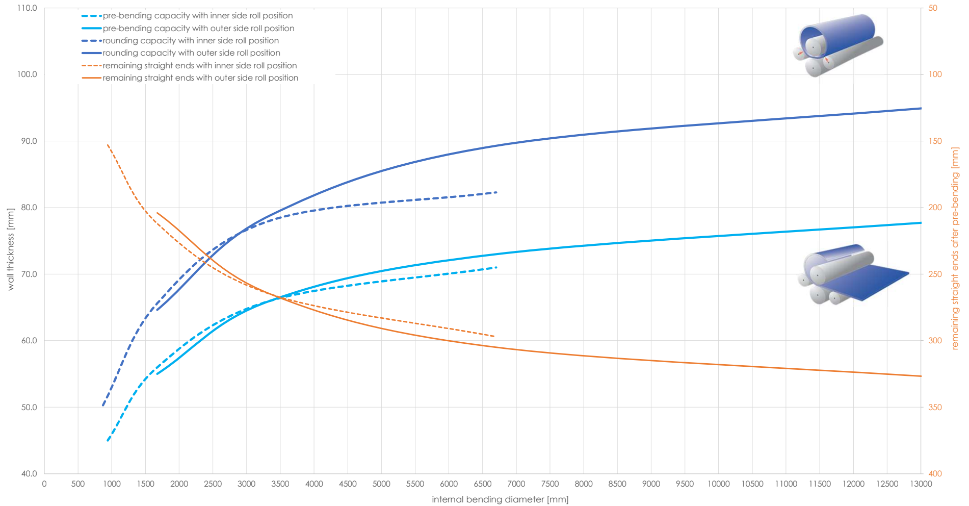
Capacity graph EVO 41513 - Yield point 260 N/mm 2 (calculated plate width 4'000 mm)
