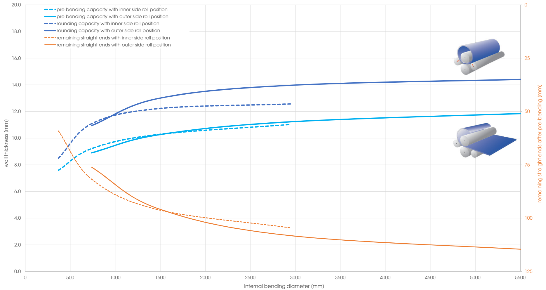
Capacity graph EVO 31031 - Yield point 360 N/mm 2 (calculated plate width 3'000 mm)
