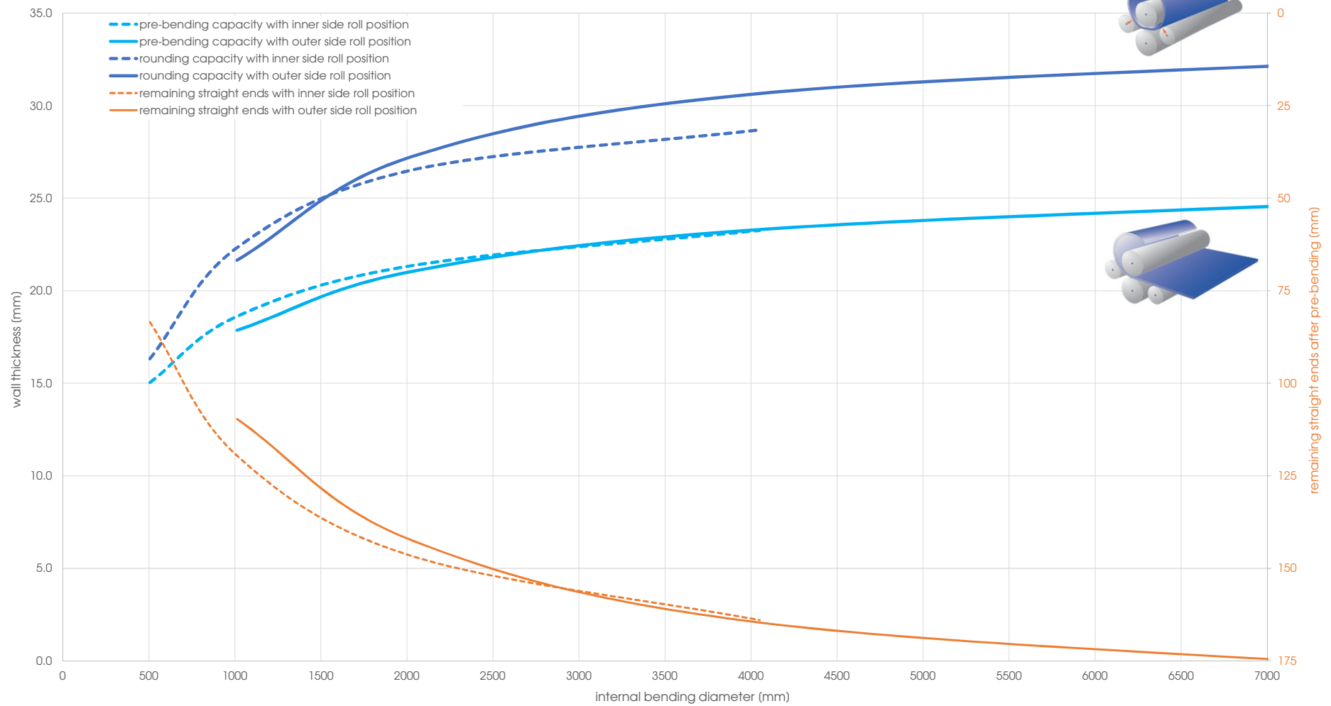
Capacity graph EVO 26139 - Yield point 690 N/mm 2 (calculated plate width 2'500 mm)
