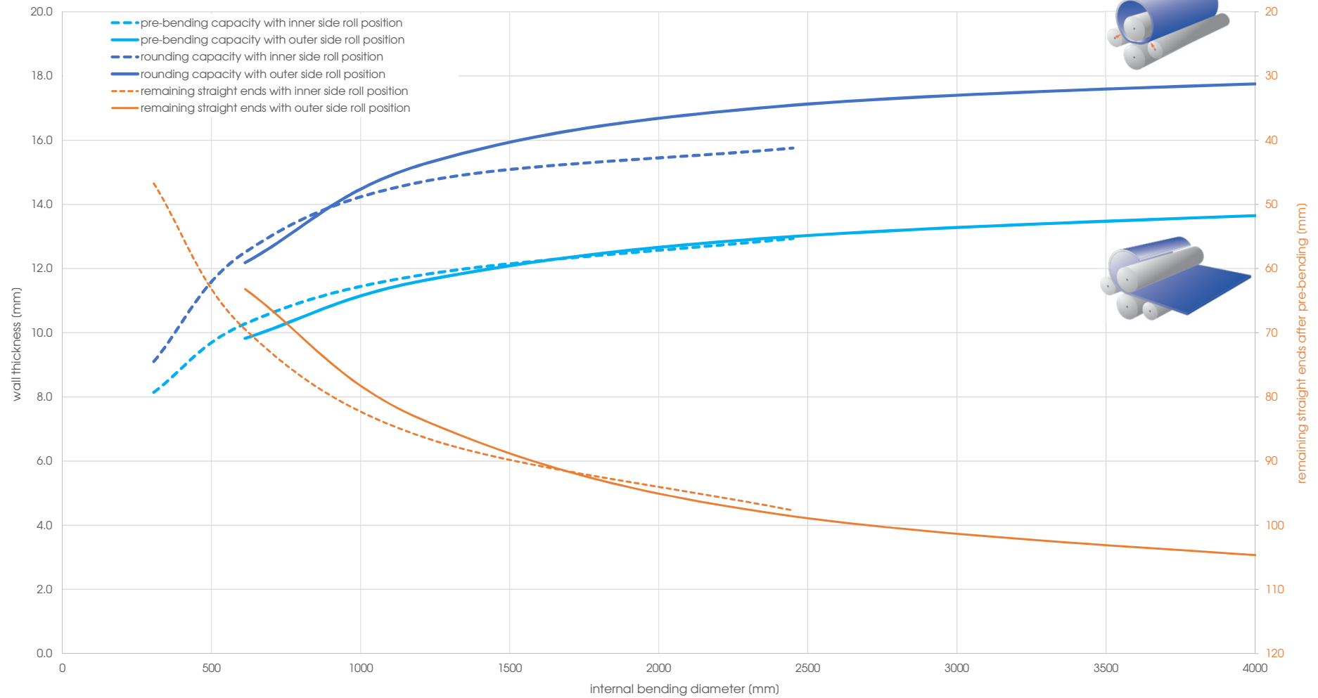
Capacity graph EVO 21031 - Yield point 360 N/mm 2 (calculated plate width 2'000 mm)
