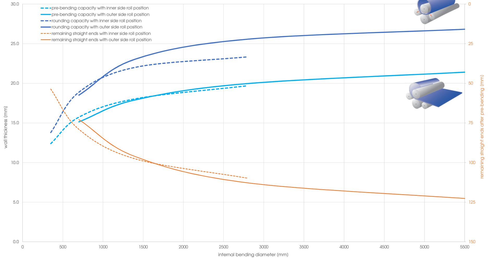
Capacity graph EVO 21049 - Yield point 260 N/mm 2 (calculated plate width 2'000 mm)
