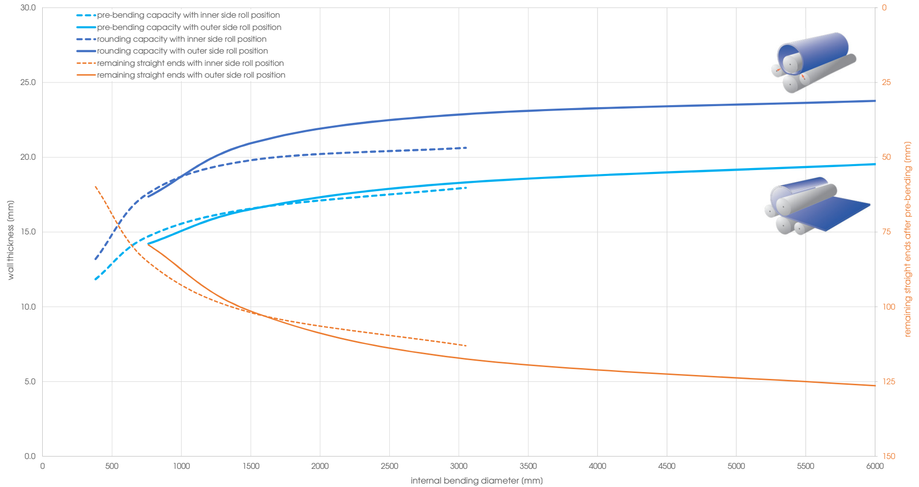
Capacity graph EVO 26049 - Yield point 260 N/mm 2 (calculated plate width 2'500 mm)
