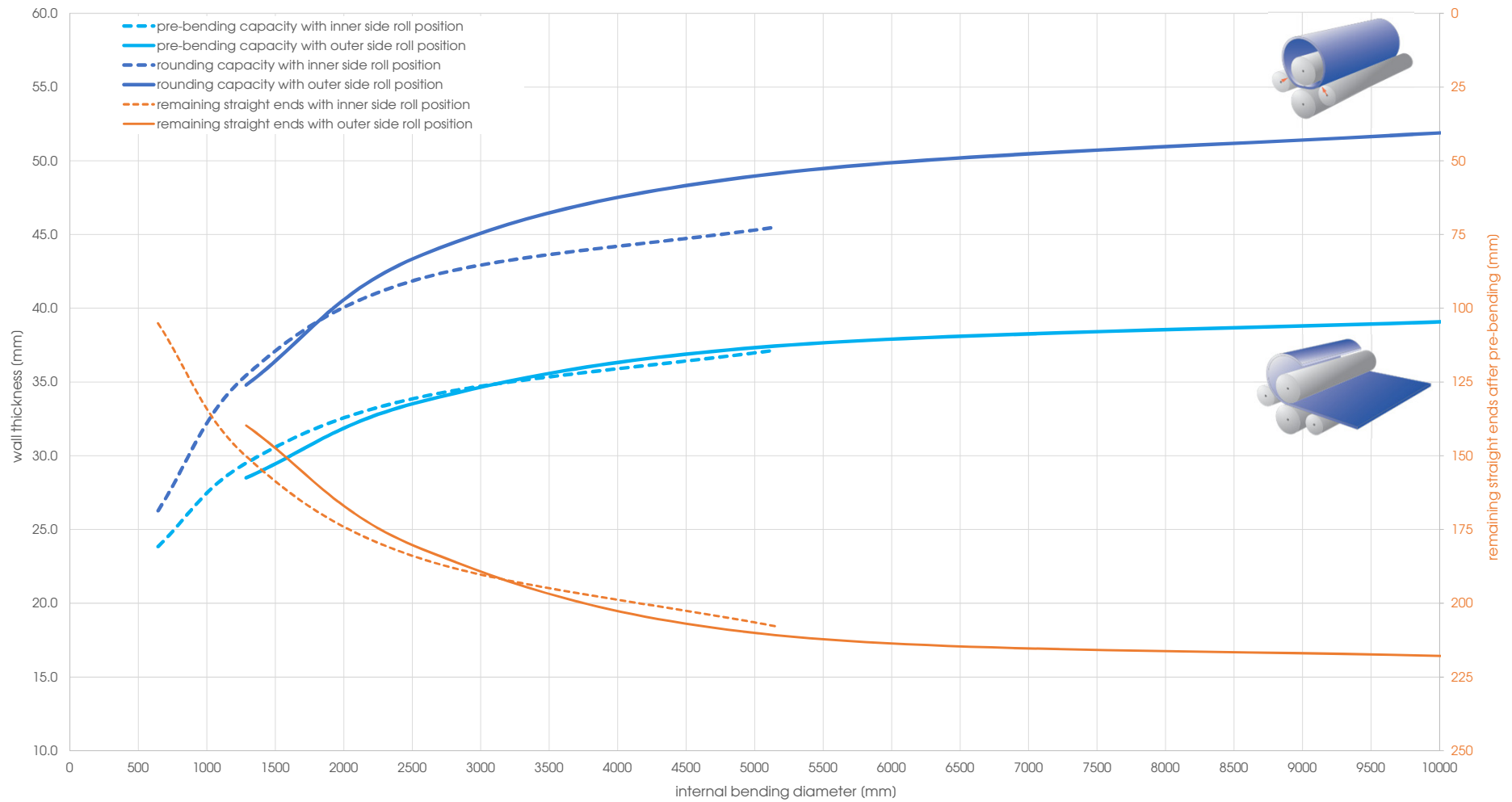
Capacity graph EVO 26283 - Yield point 690 N/mm 2 (calculated plate width 2'500 mm)
