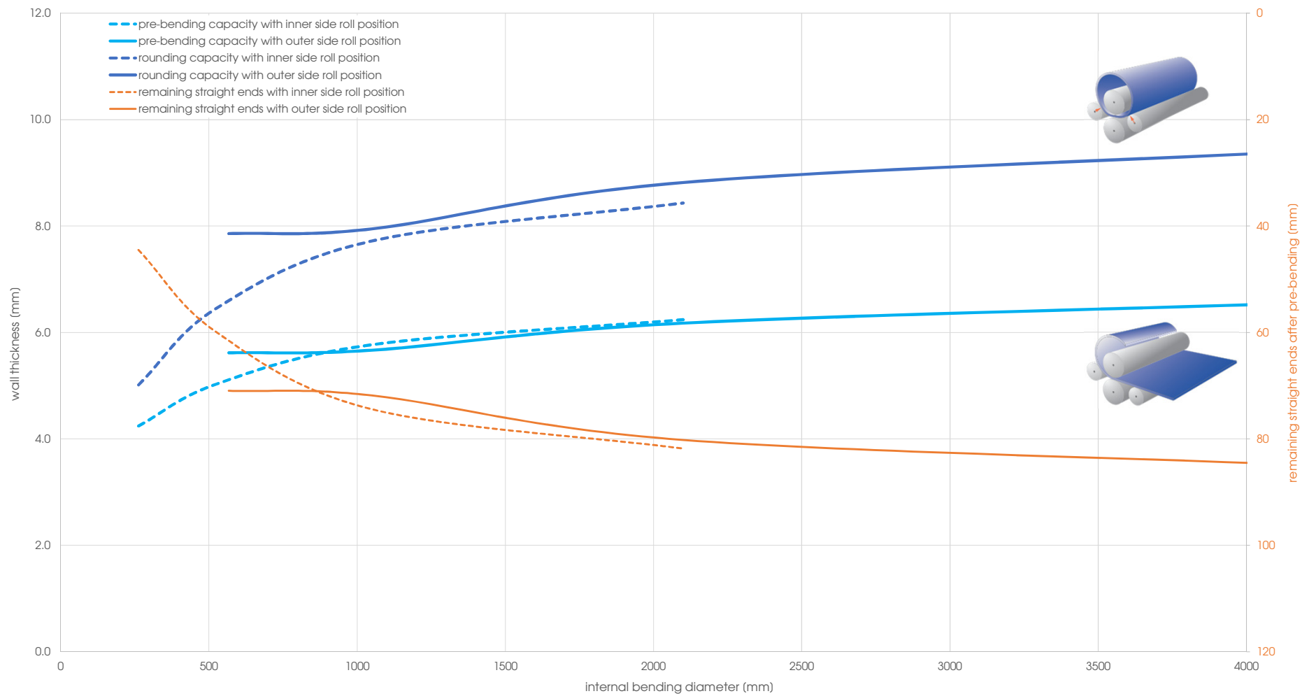
Capacity graph EVO 21015 - Yield point 690 N/mm 2 (calculated plate width 2'000 mm)
