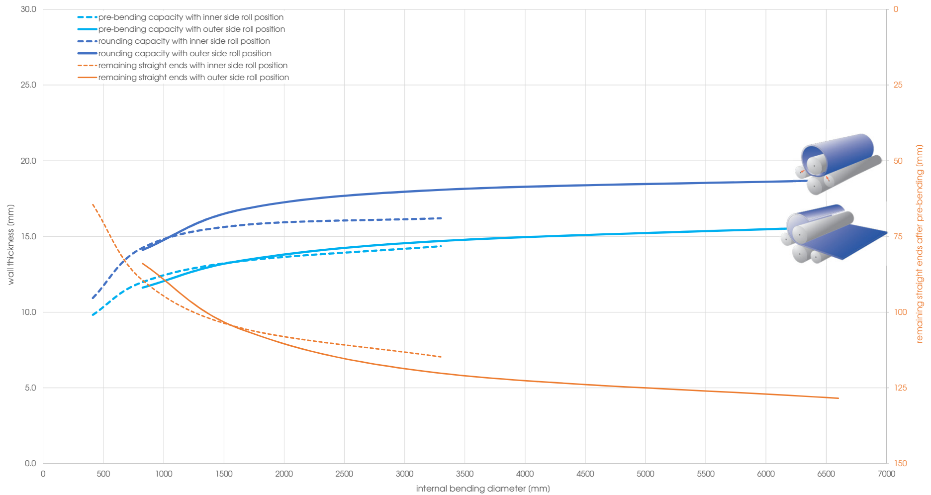
Capacity graph EVO 31049 - Yield point 360 N/mm 2 (calculated plate width 3'000 mm)
