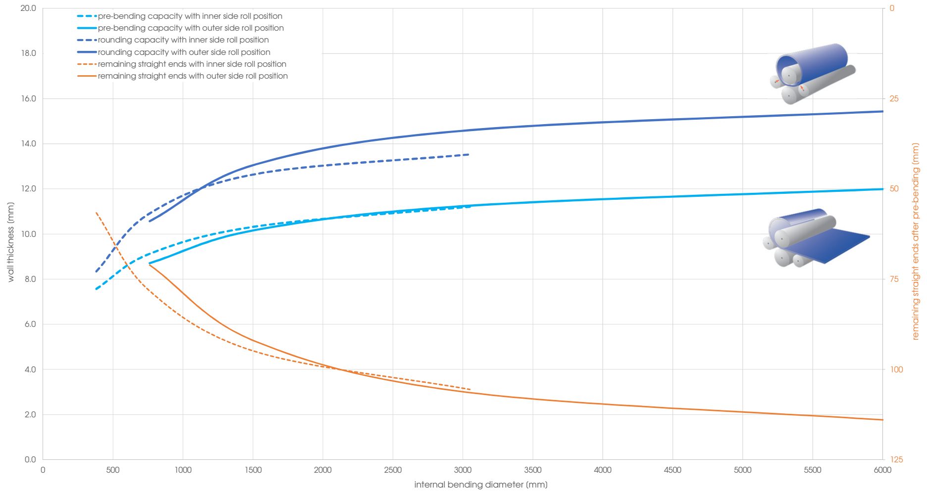
Capacity graph EVO 26049 - Yield point 690 N/mm 2 (calculated plate width 2'500 mm)
