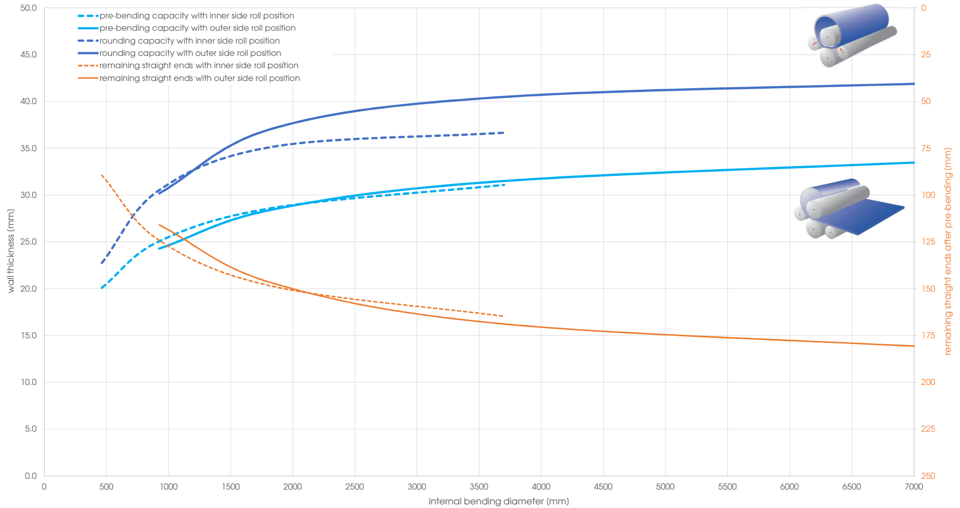
Capacity graph EVO 26102 - Yield point 260 N/mm 2 (calculated plate width 2'500 mm)
