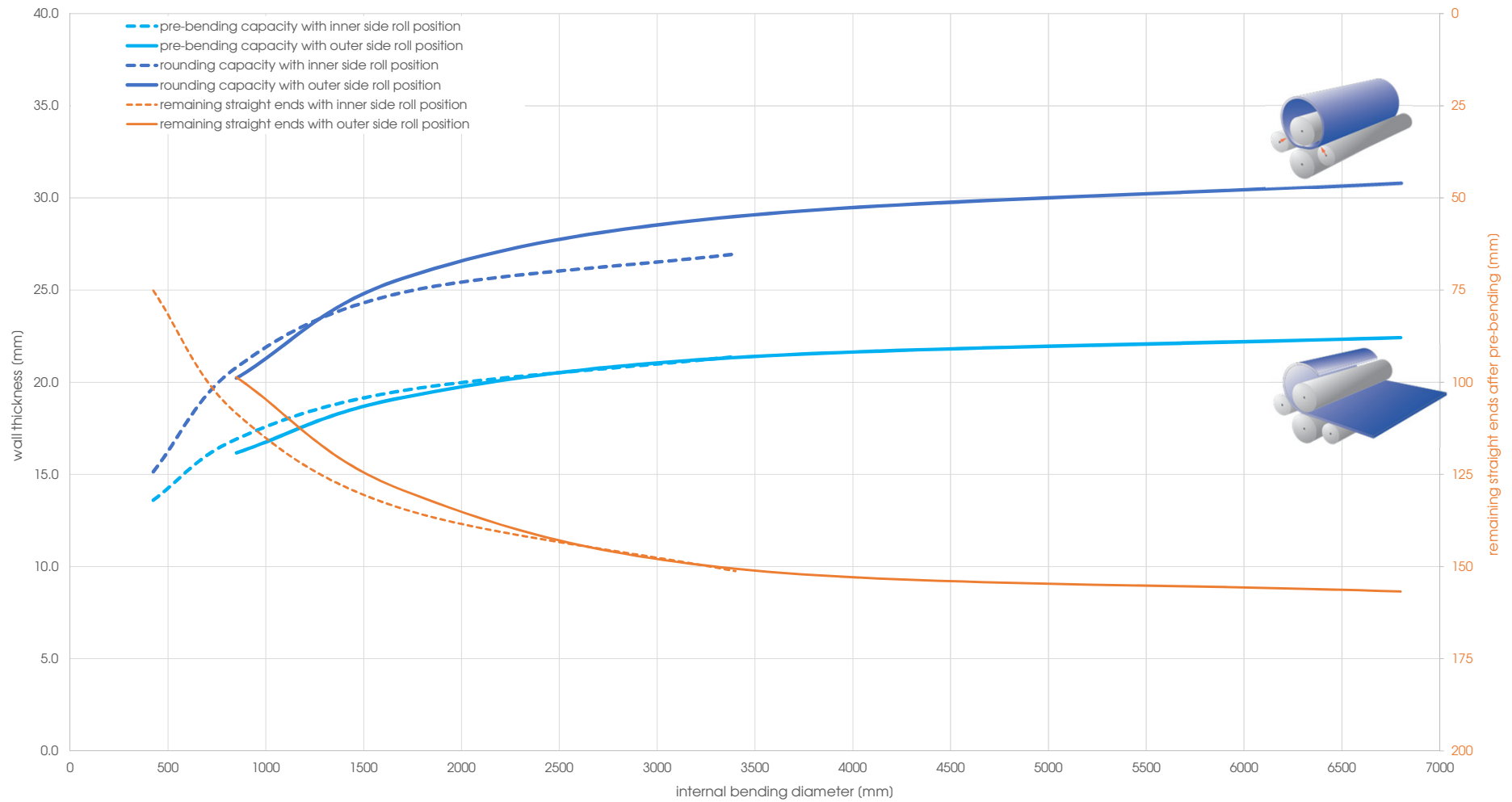
Capacity graph EVO 21102 - Yield point 690 N/mm 2 (calculated plate width 2'000 mm)
