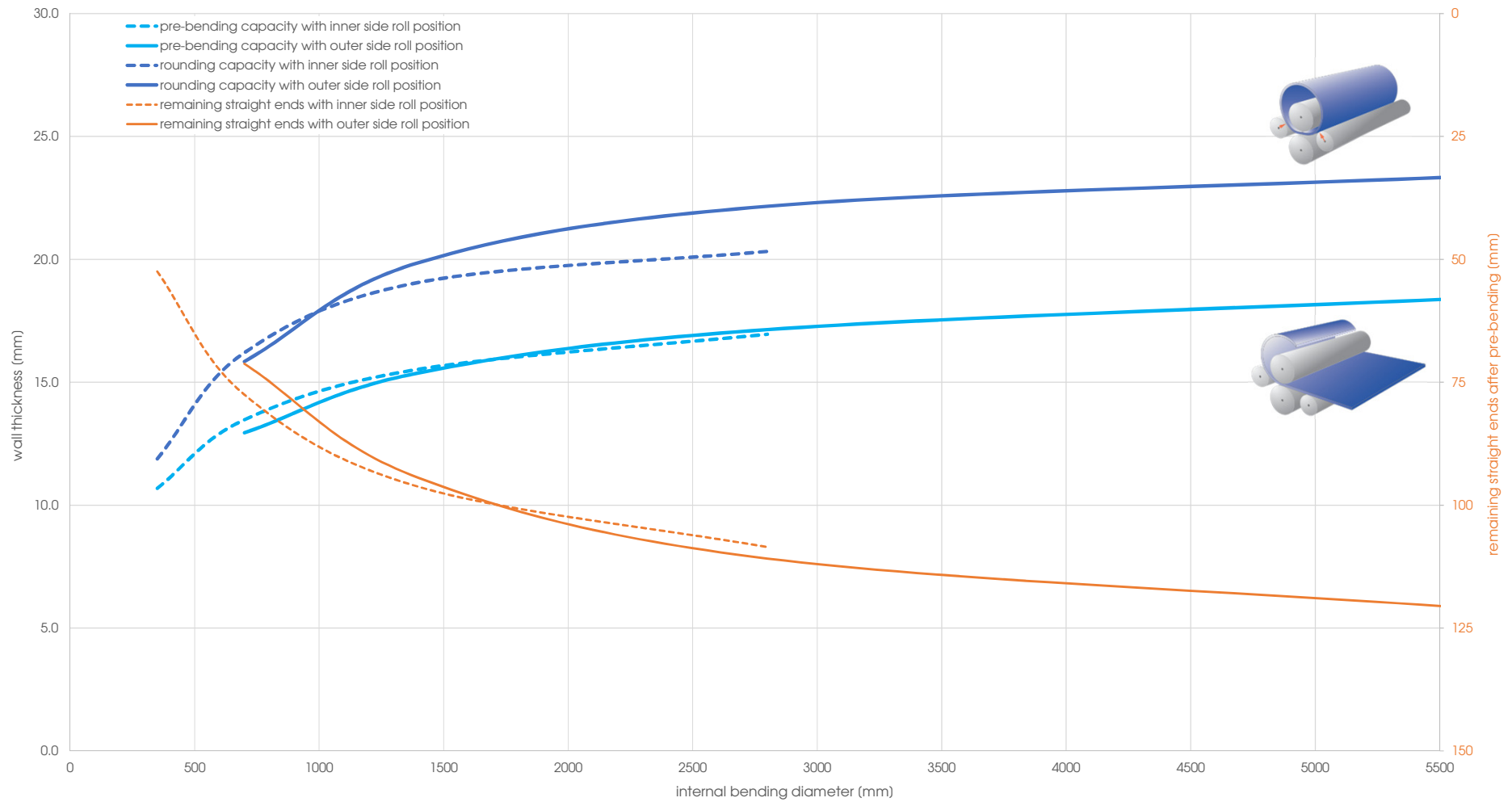
Capacity graph EVO 21049 - Yield point 360 N/mm 2 (calculated plate width 2'000 mm)
