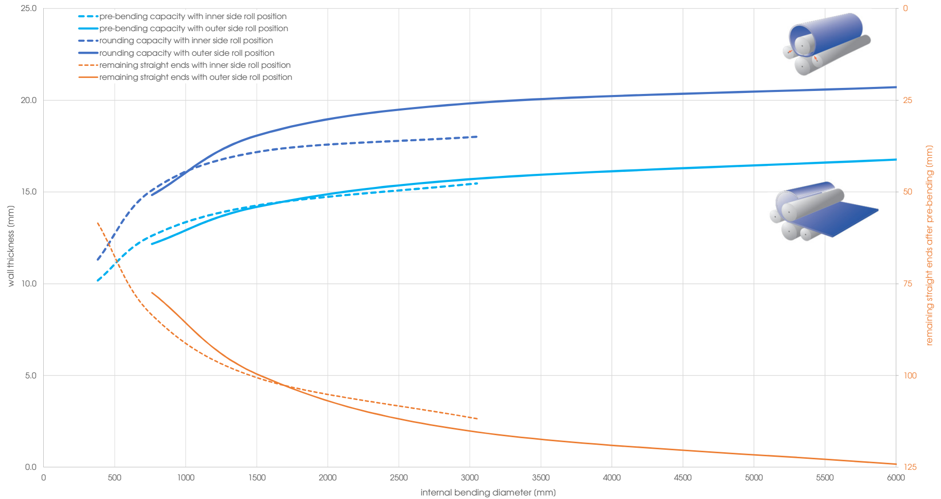
Capacity graph EVO 26049 - Yield point 360 N/mm 2 (calculated plate width 2'500 mm)
