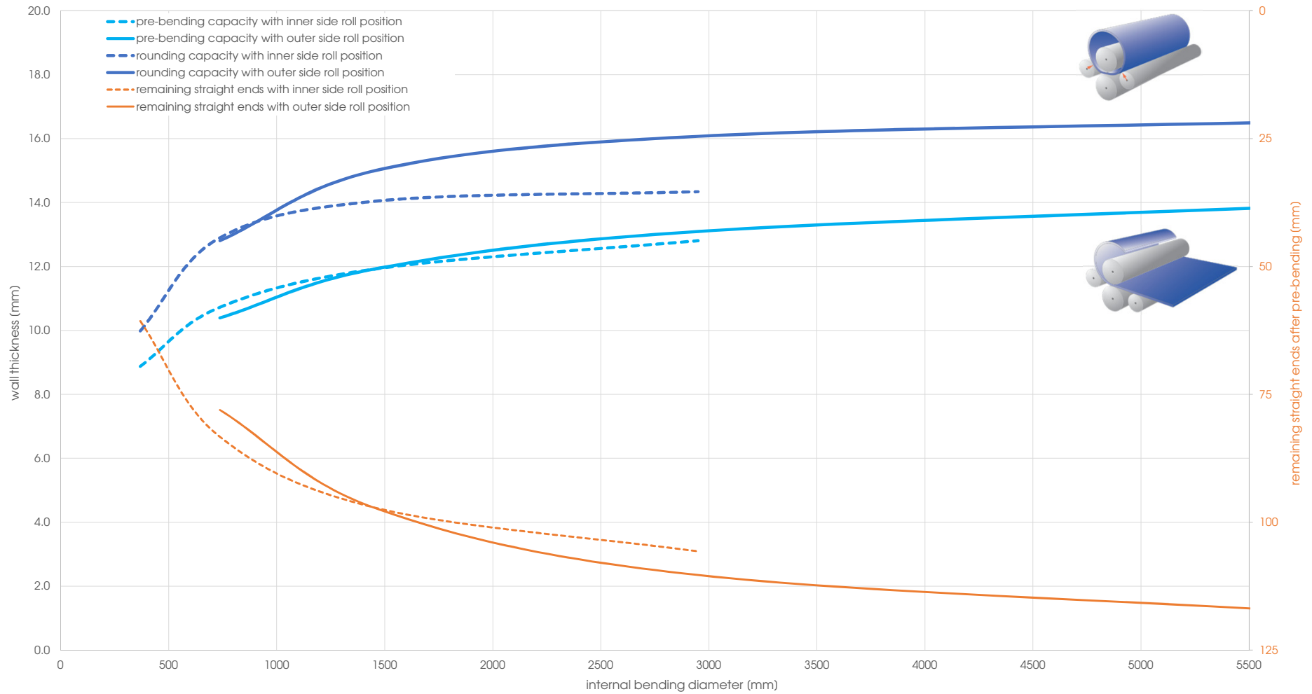
Capacity graph EVO 31031 - Yield point 260 N/mm 2 (calculated plate width 3'000 mm)
