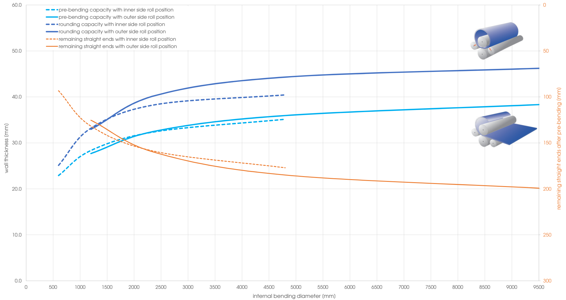
Capacity graph EVO 31196 - Yield point 360 N/mm 2 (calculated plate width 3'000 mm)
