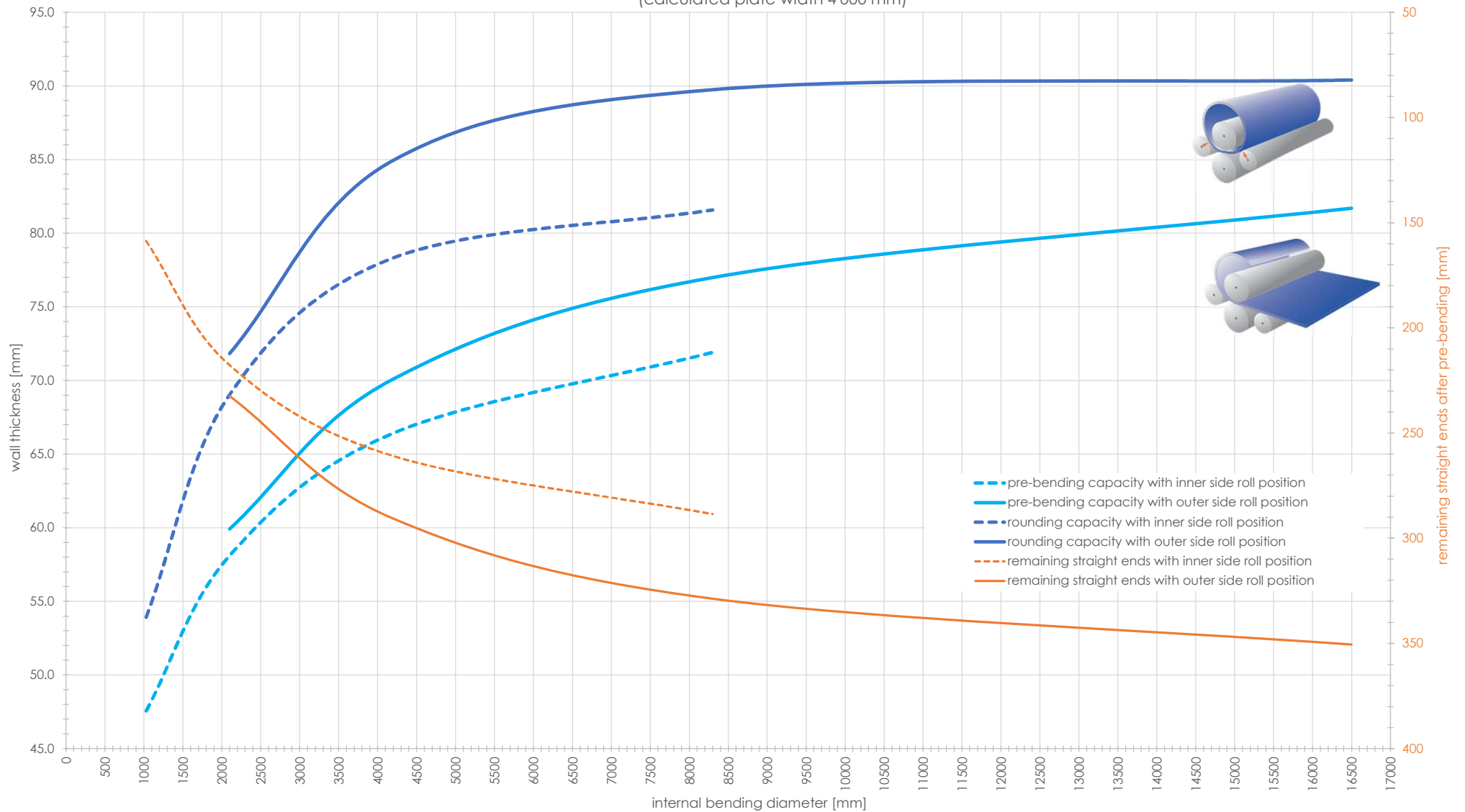
Capacity graph EVO 41680 - Yield point 360 N/mm 2 (calculated plate width 4'000 mm)
