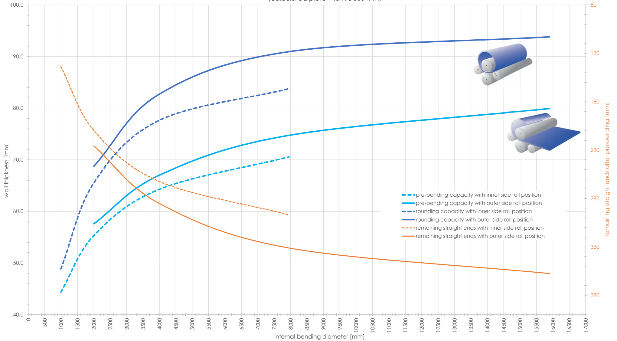
Capacity graph EVO 31871 - Yield point 690 N/mm 2 (calculated plate width 3'000 mm)
