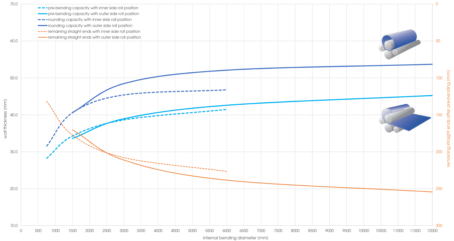
Capacity graph EVO 41283 - Yield point 360 N/mm 2 (calculated plate width 4'000 mm)
