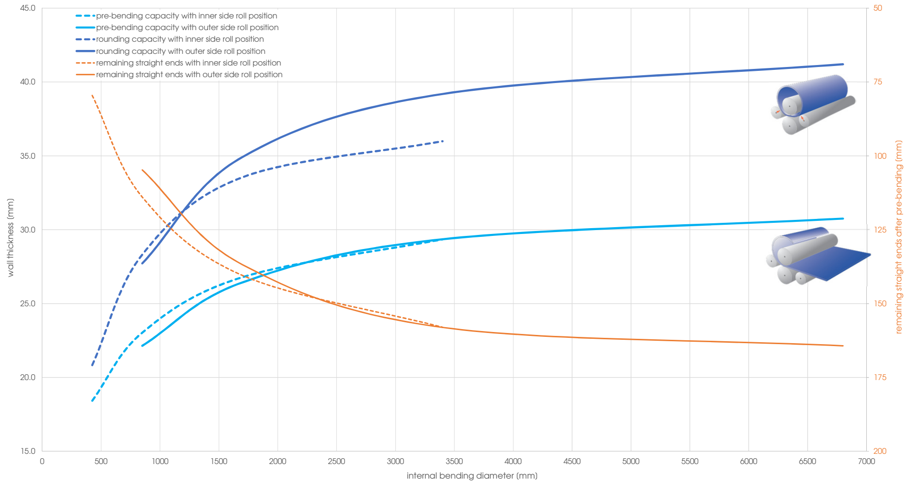
Capacity graph EVO 21102 - Yield point 360 N/mm 2 (calculated plate width 2'000 mm)
