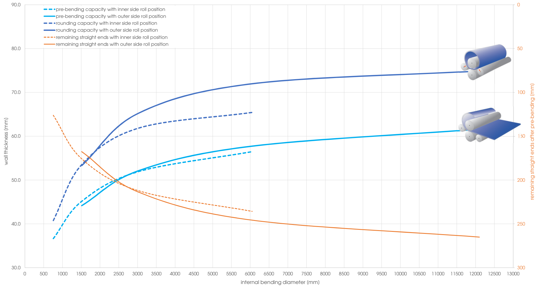
Capacity graph EVO 31385 - Yield point 360 N/mm 2 (calculated plate width 3'000 mm)
