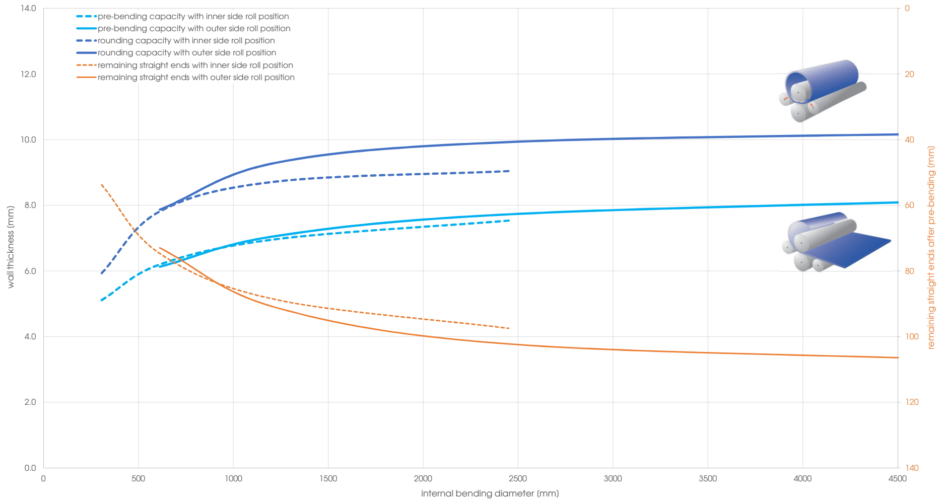
Capacity graph EVO 31015 - Yield point 360 N/mm 2 (calculated plate width 3'000 mm)
