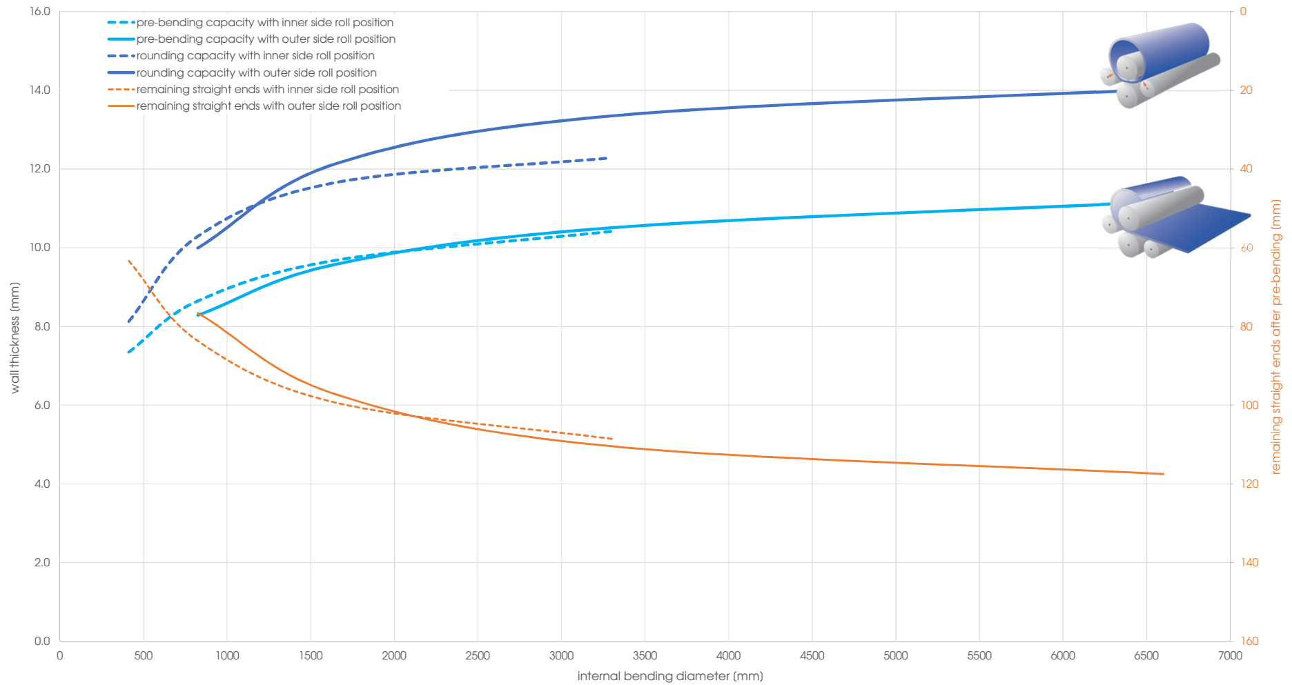
Capacity graph EVO 31049 - Yield point 690 N/mm 2 (calculated plate width 3'000 mm)
