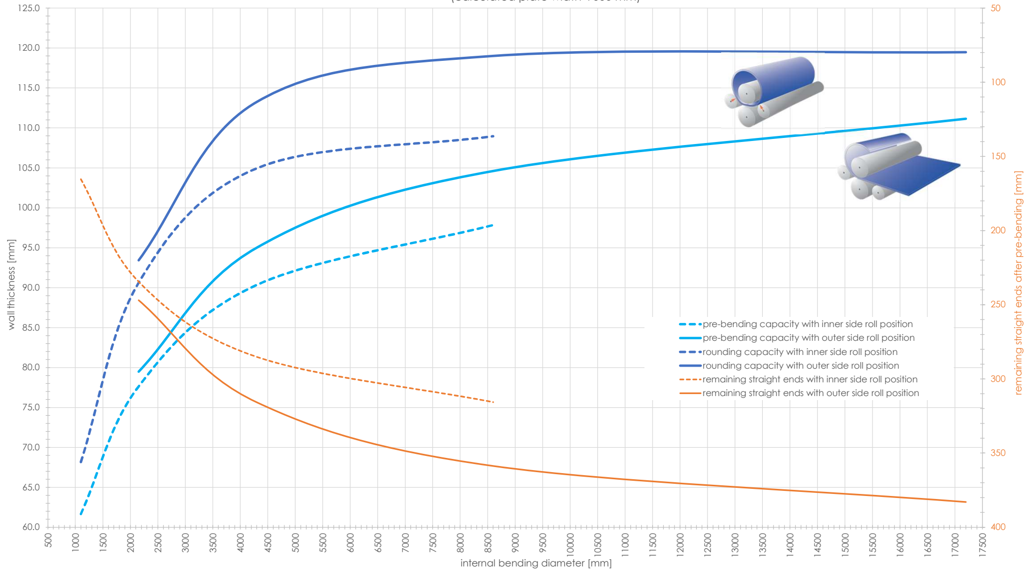
Capacity graph EVO 41871 - Yield point 260 N/mm 2 (calculated plate width 4'000 mm)
