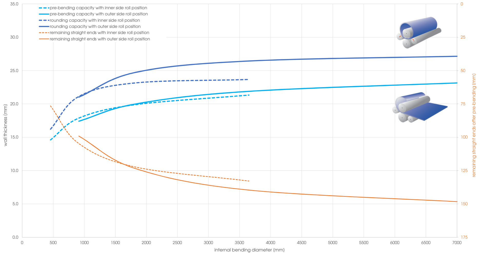
Capacity graph EVO 31071 - Yield point 260 N/mm 2 (calculated plate width 3'000 mm)
