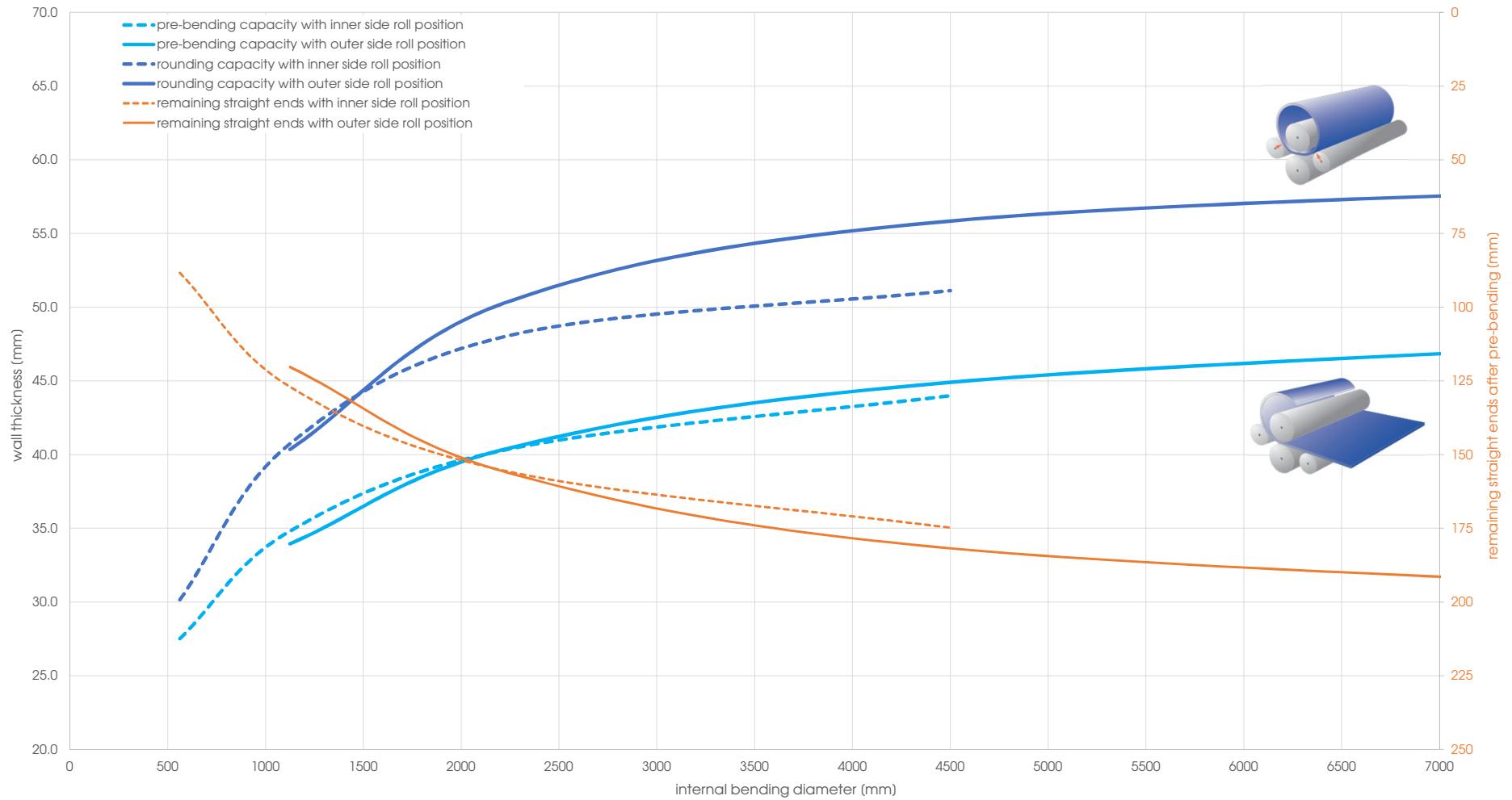
Capacity graph EVO 26196 - Yield point 260 N/mm 2 (calculated plate width 2'500 mm)
