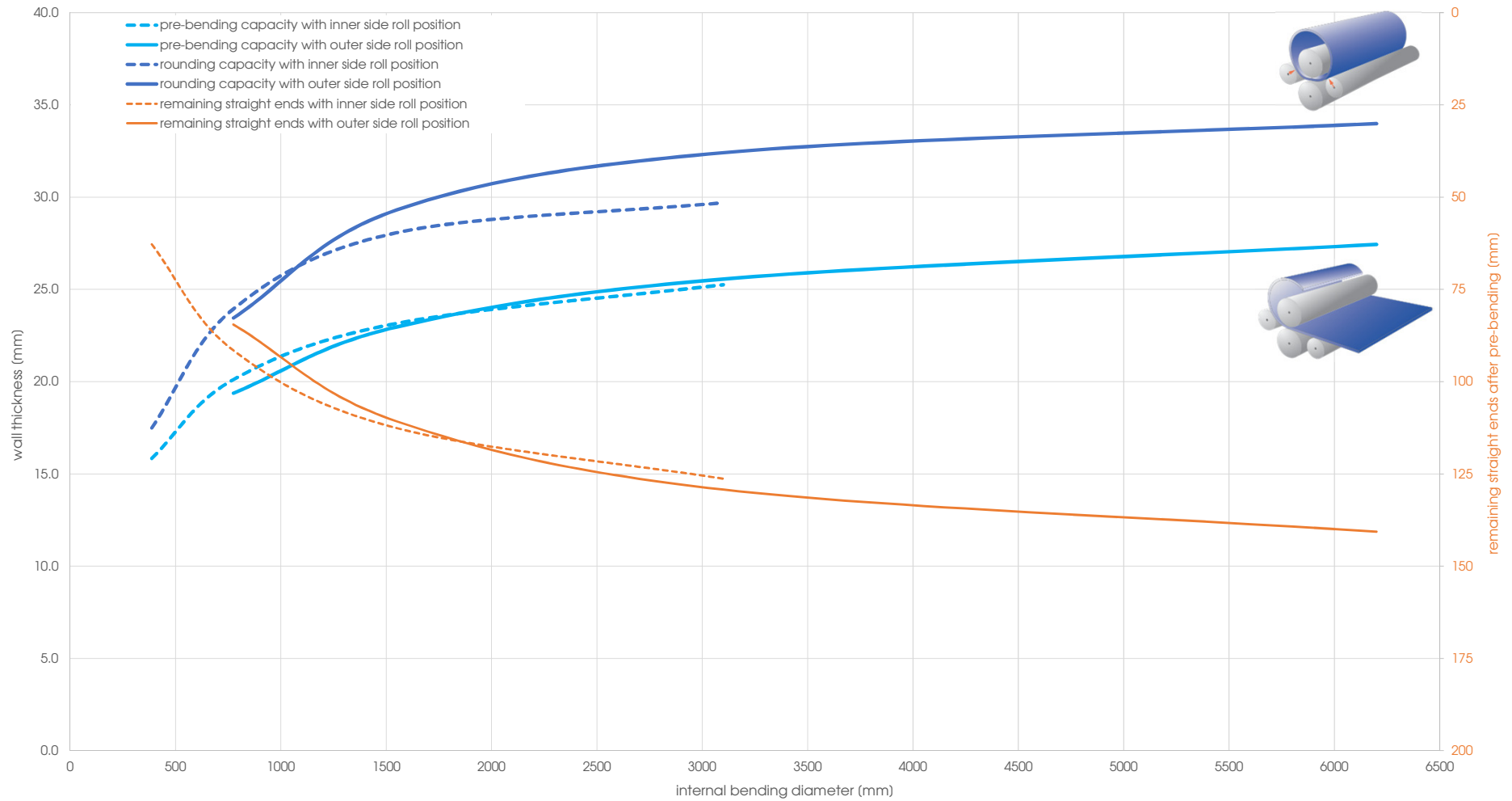
Capacity graph EVO 21071 - Yield point 260 N/mm 2 (calculated plate width 2'000 mm)
