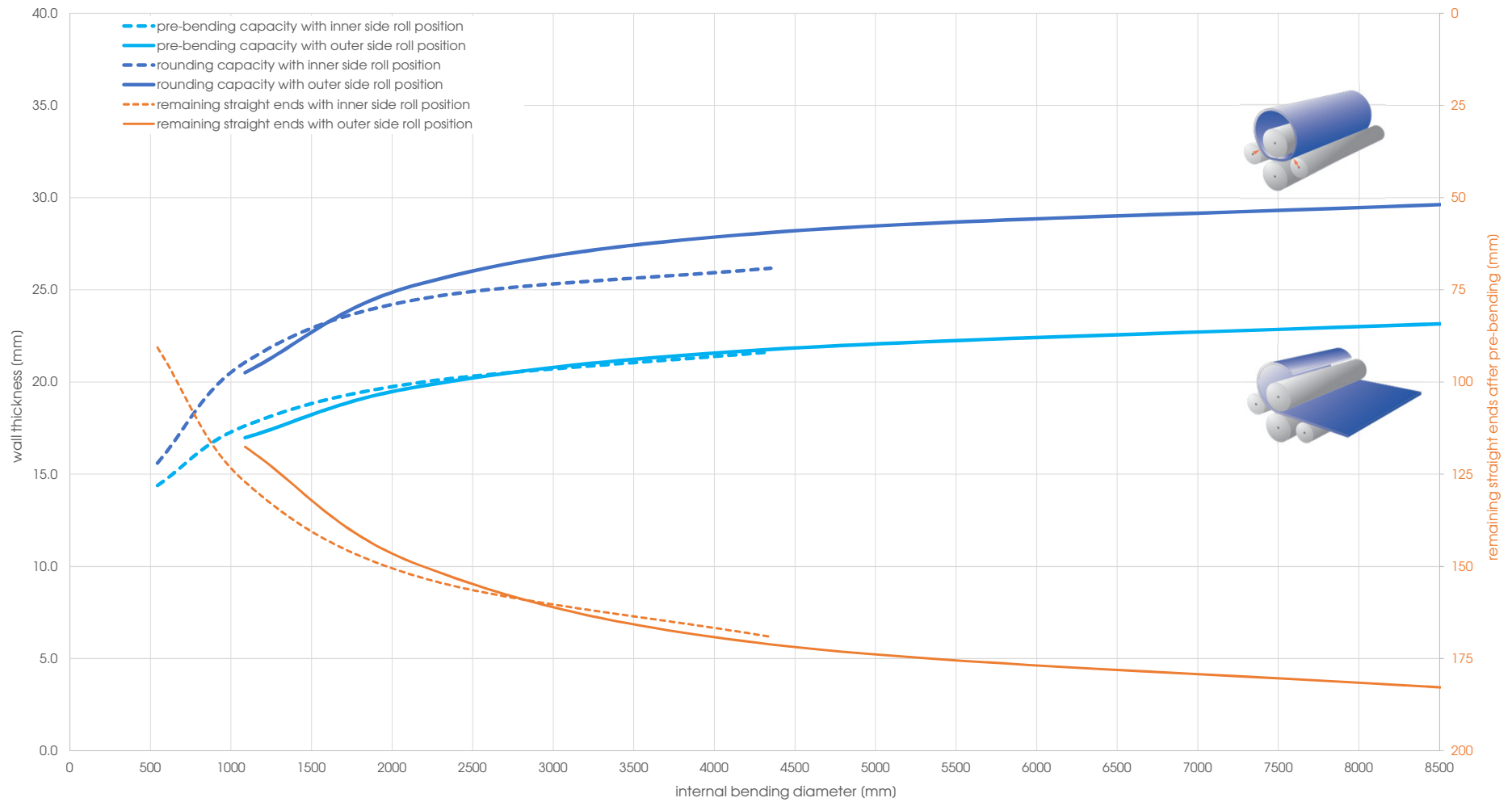
Capacity graph EVO 31139 - Yield point 690 N/mm 2 (calculated plate width 3'000 mm)
