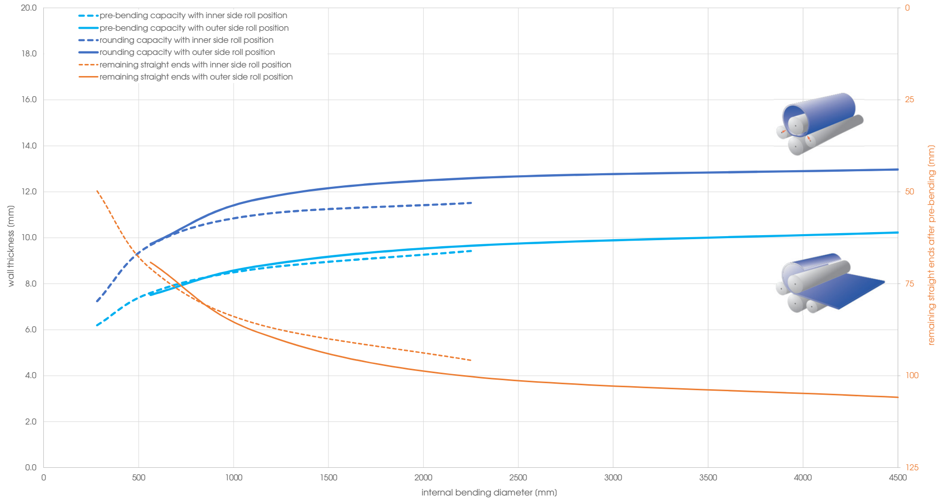
Capacity graph EVO 26015 - Yield point 260 N/mm 2 (calculated plate width 2'500 mm)
