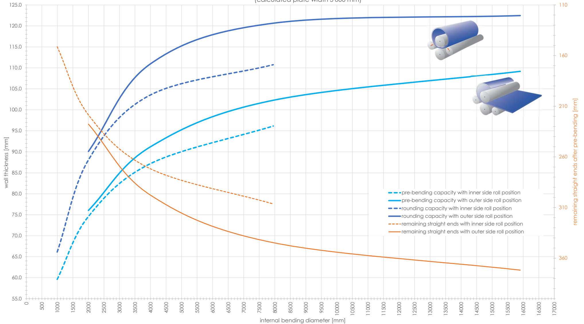
Capacity graph EVO 31871 - Yield point 360 N/mm 2 (calculated plate width 3'000 mm)
