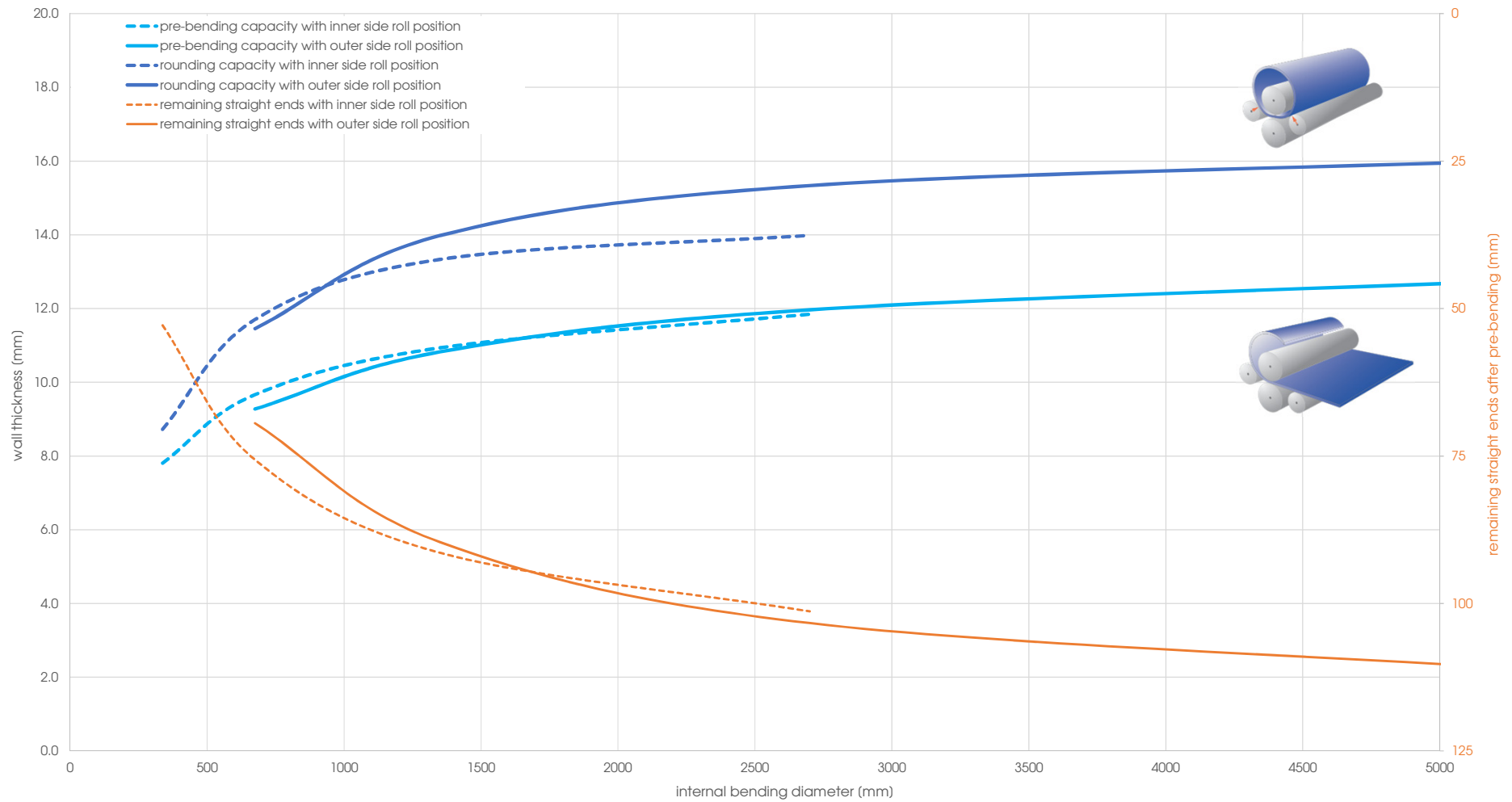
Capacity graph EVO 26031 - Yield point 360 N/mm 2 (calculated plate width 2'500 mm)
