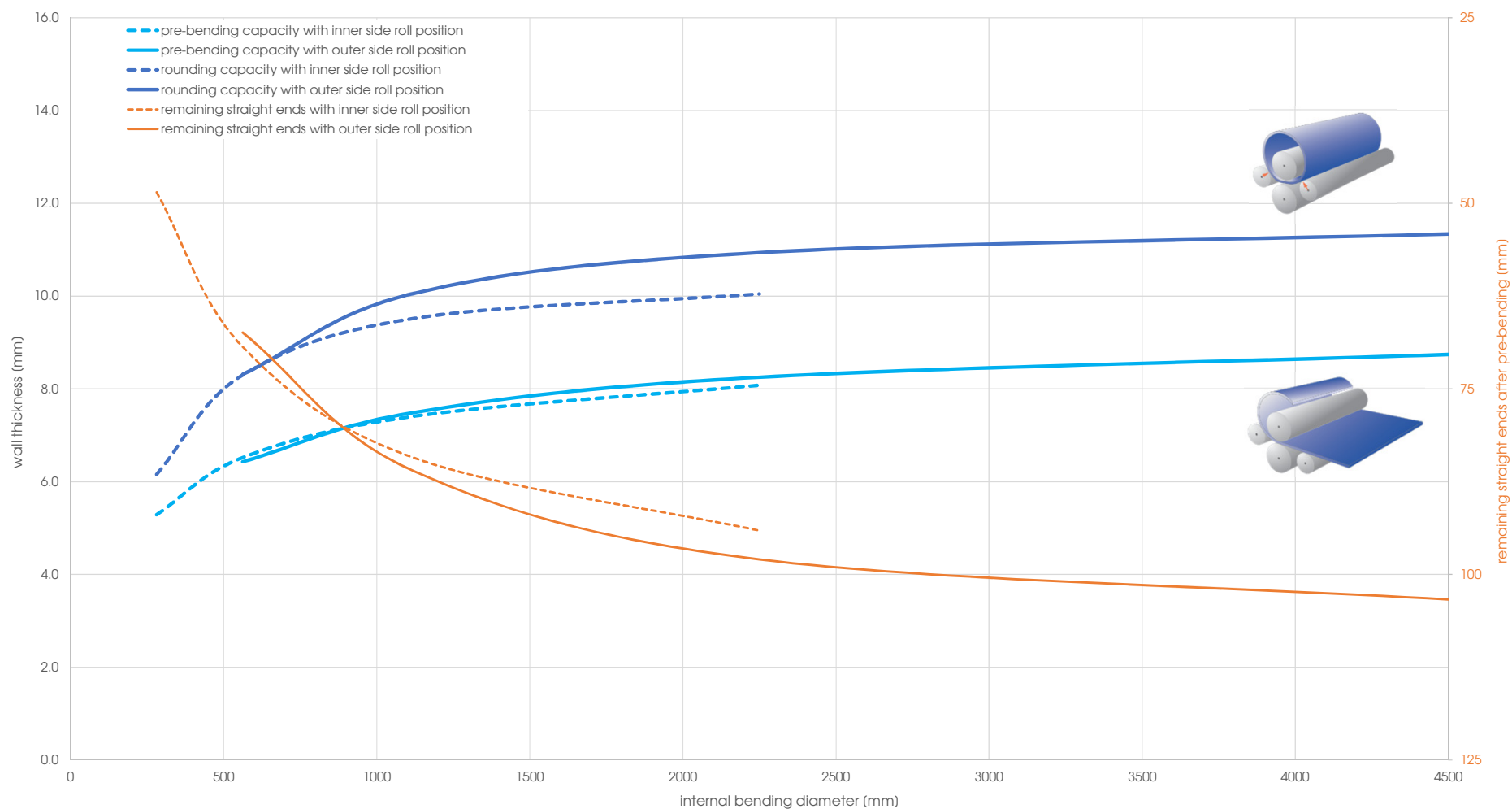
Capacity graph EVO 26015 - Yield point 360 N/mm 2 (calculated plate width 2'500 mm)
