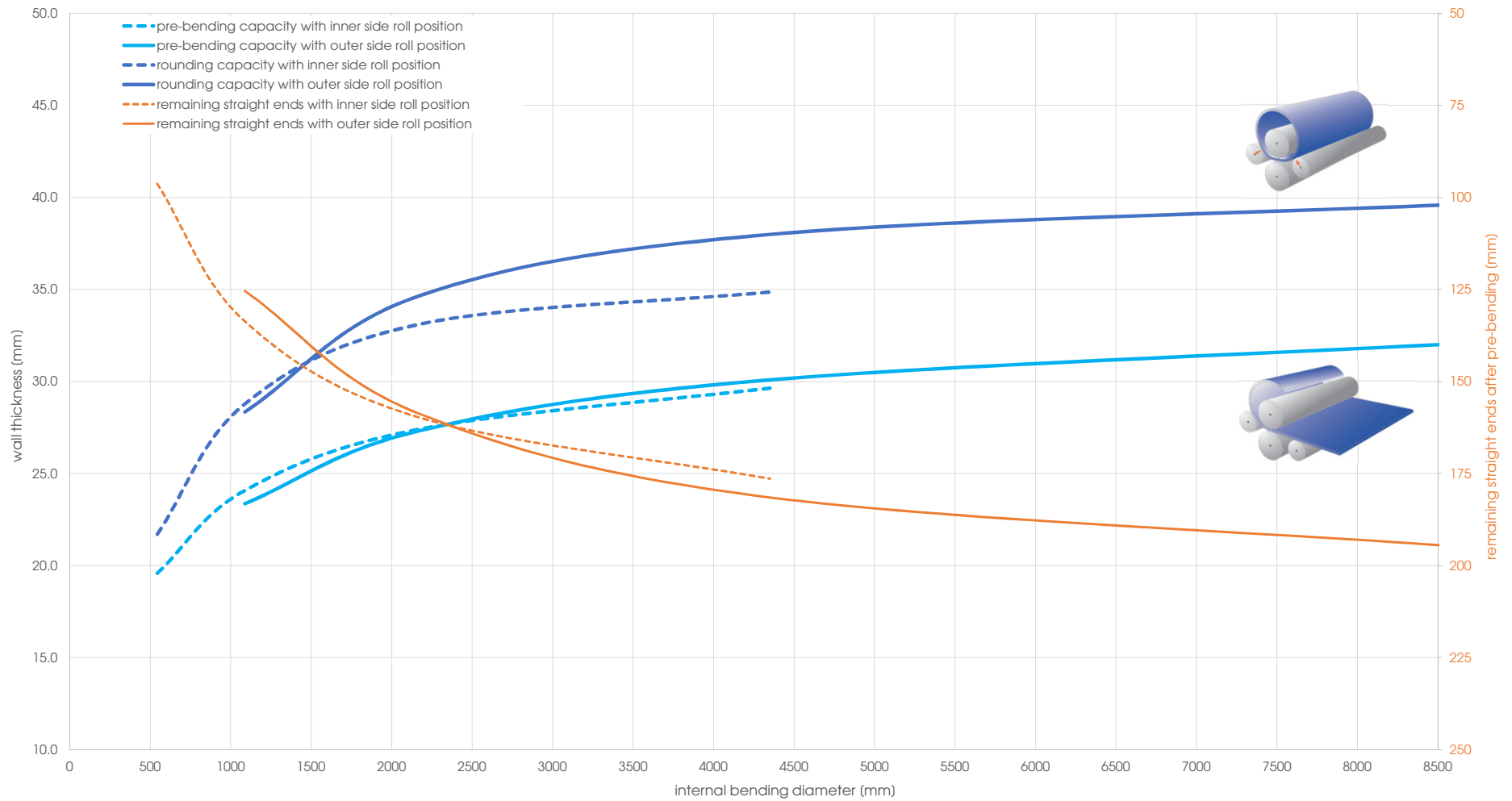
Capacity graph EVO 31139 - Yield point 360 N/mm 2 (calculated plate width 3'000 mm)
