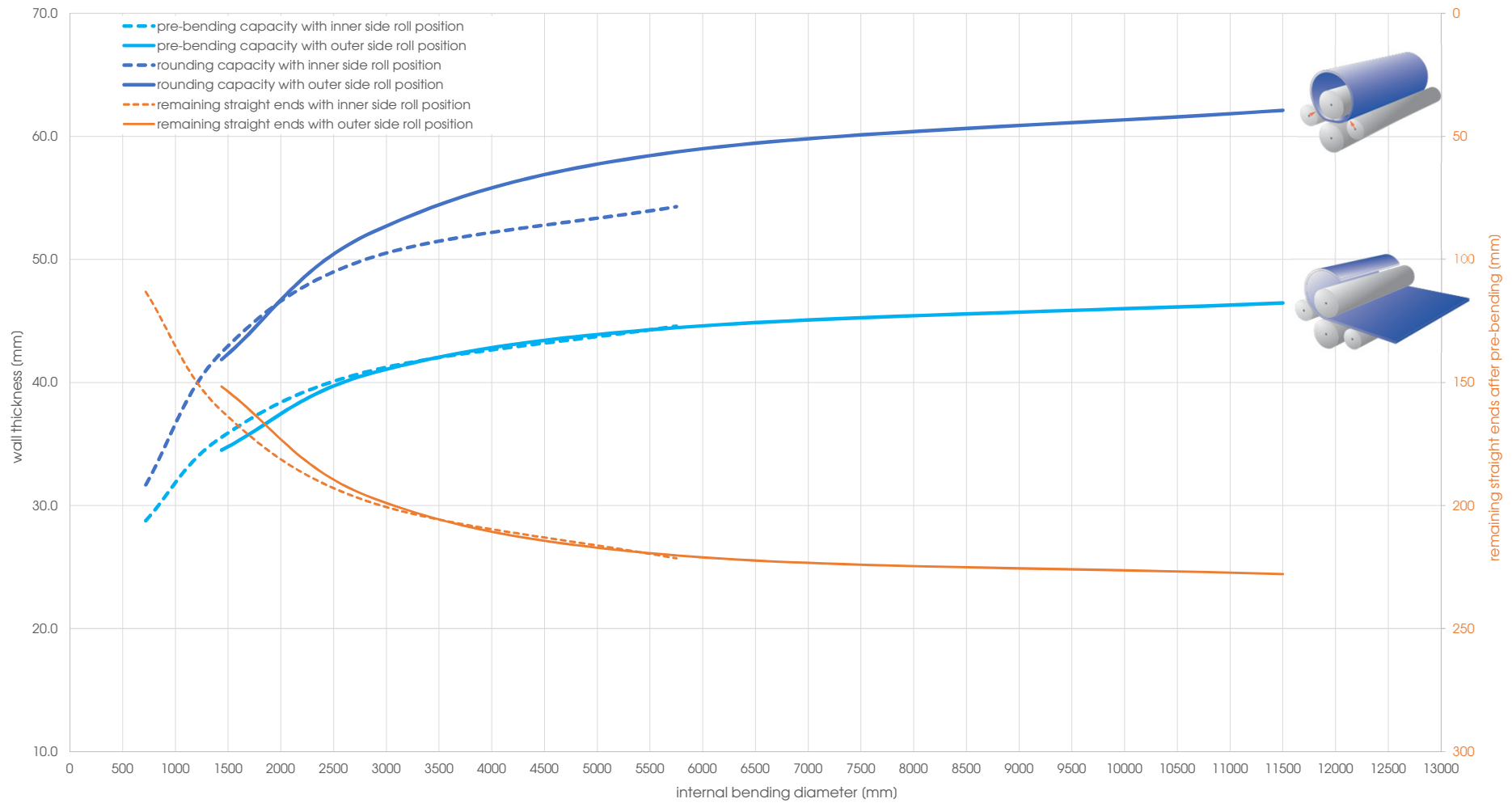
Capacity graph EVO 26385 - Yield point 690 N/mm 2 (calculated plate width 2'500 mm)
