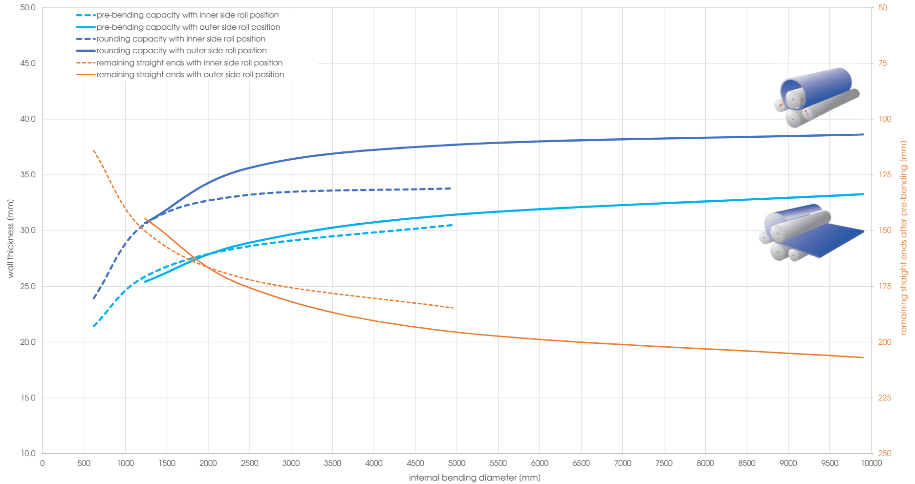
Capacity graph EVO 41139 - Yield point 260 N/mm 2 (calculated plate width 4'000 mm)
