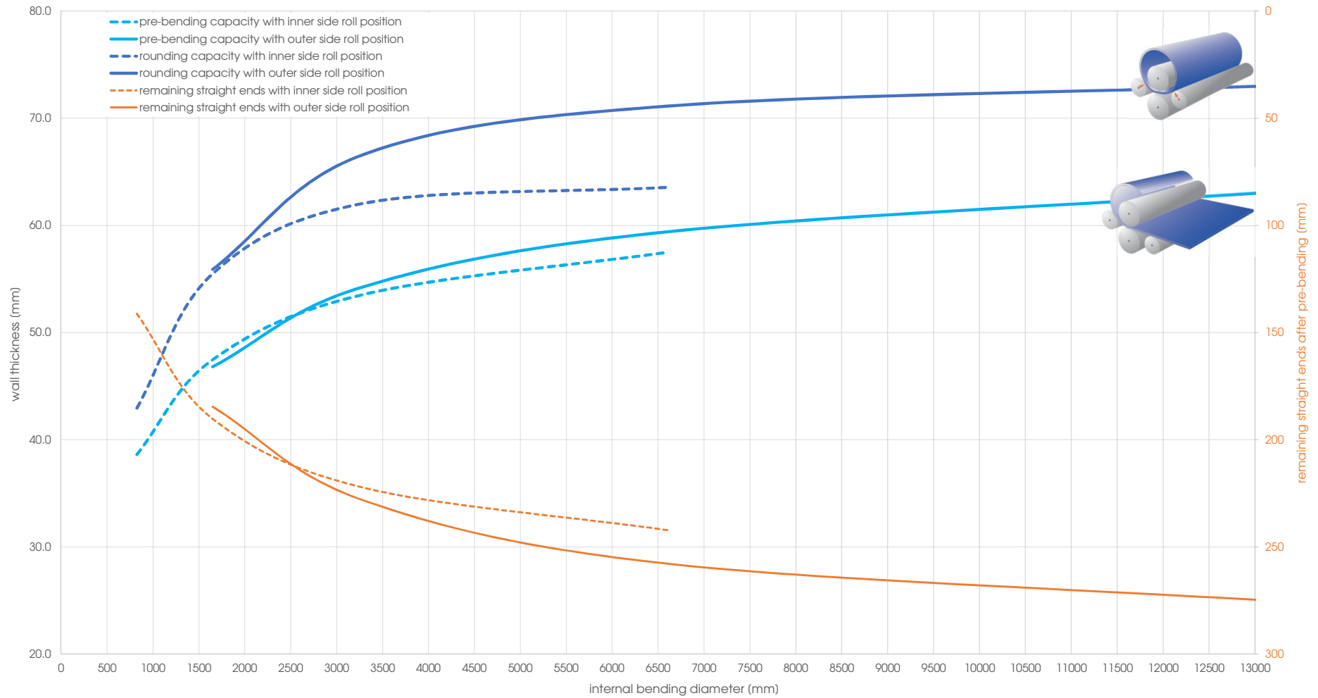
Capacity graph EVO 41385 - Yield point 260 N/mm 2 (calculated plate width 4'000 mm)
