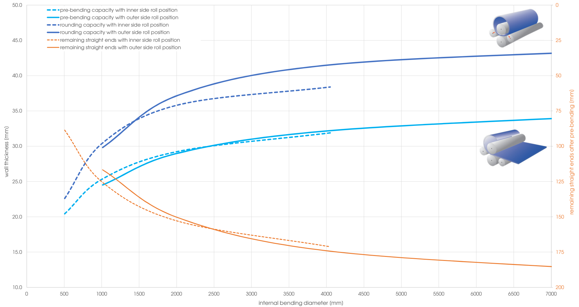
Capacity graph EVO 26139 - Yield point 360 N/mm 2 (calculated plate width 2'500 mm)
