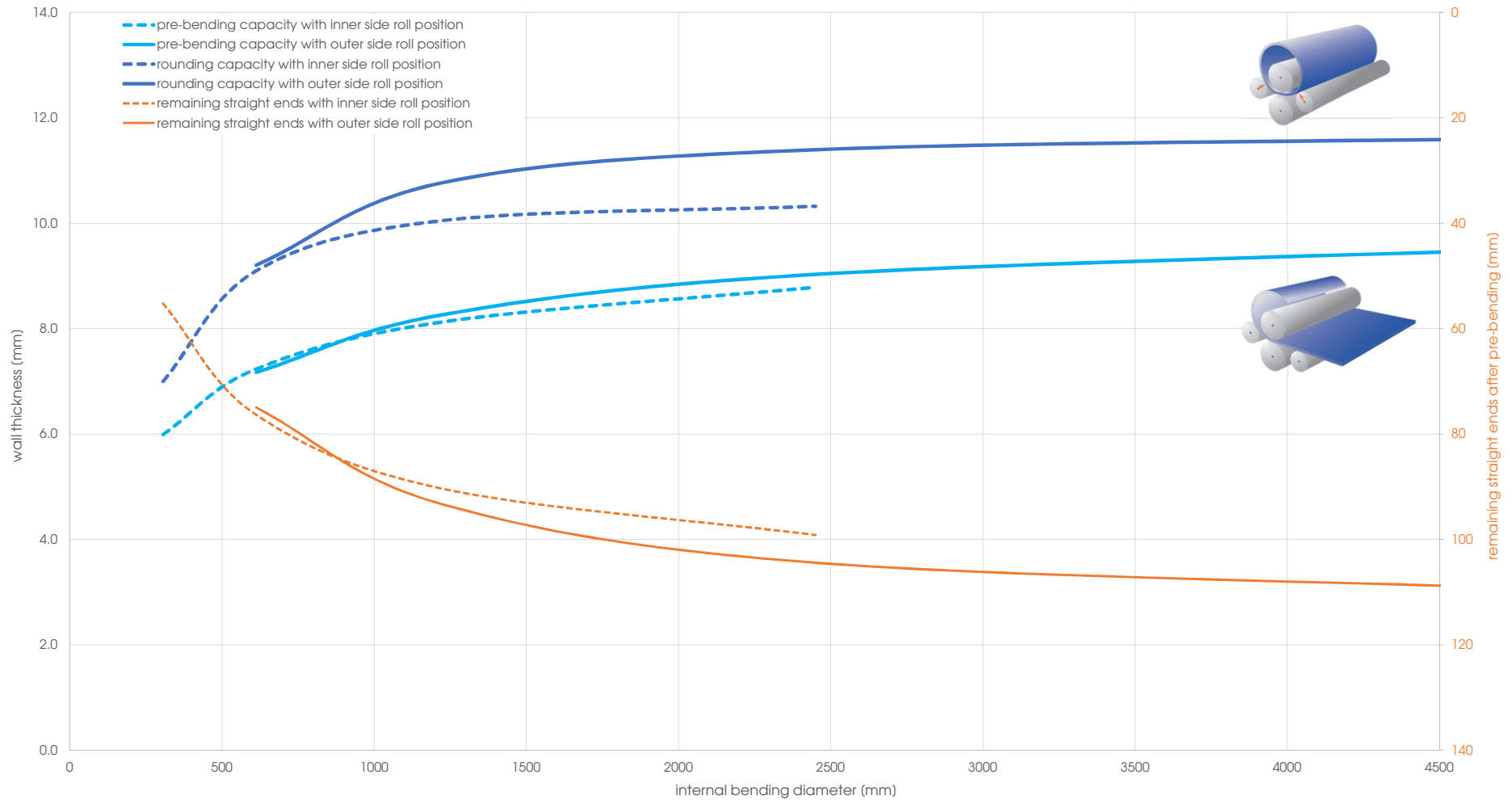
Capacity graph EVO 31015 - Yield point 260 N/mm 2 (calculated plate width 3'000 mm)
