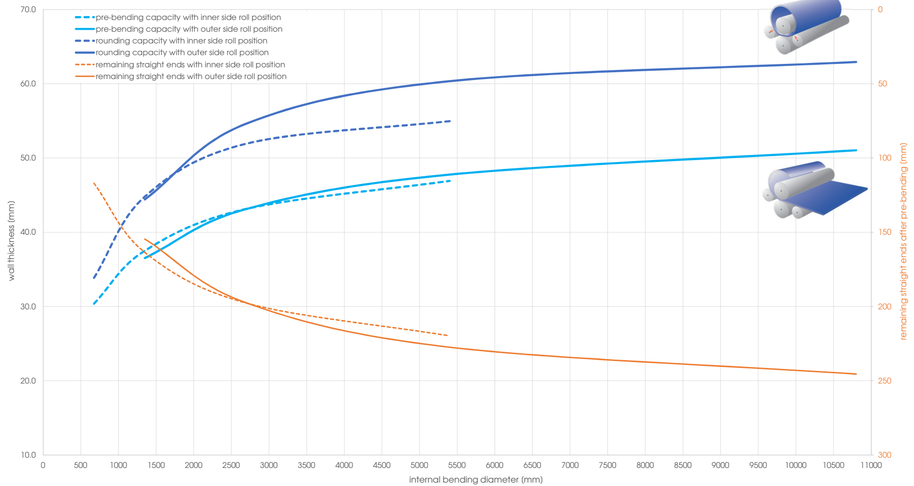
Capacity graph EVO 31283 - Yield point 360 N/mm 2 (calculated plate width 3'000 mm)
