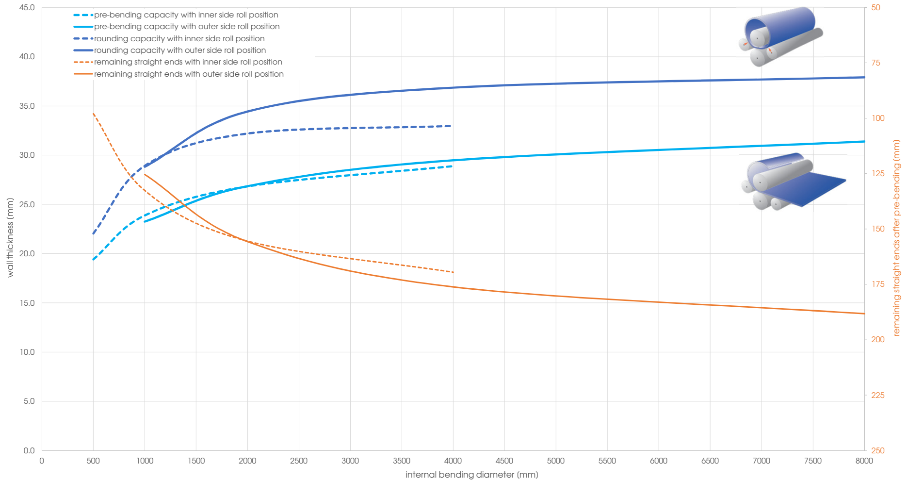
Capacity graph EVO 31102 - Yield point 260 N/mm 2 (calculated plate width 3'000 mm)
