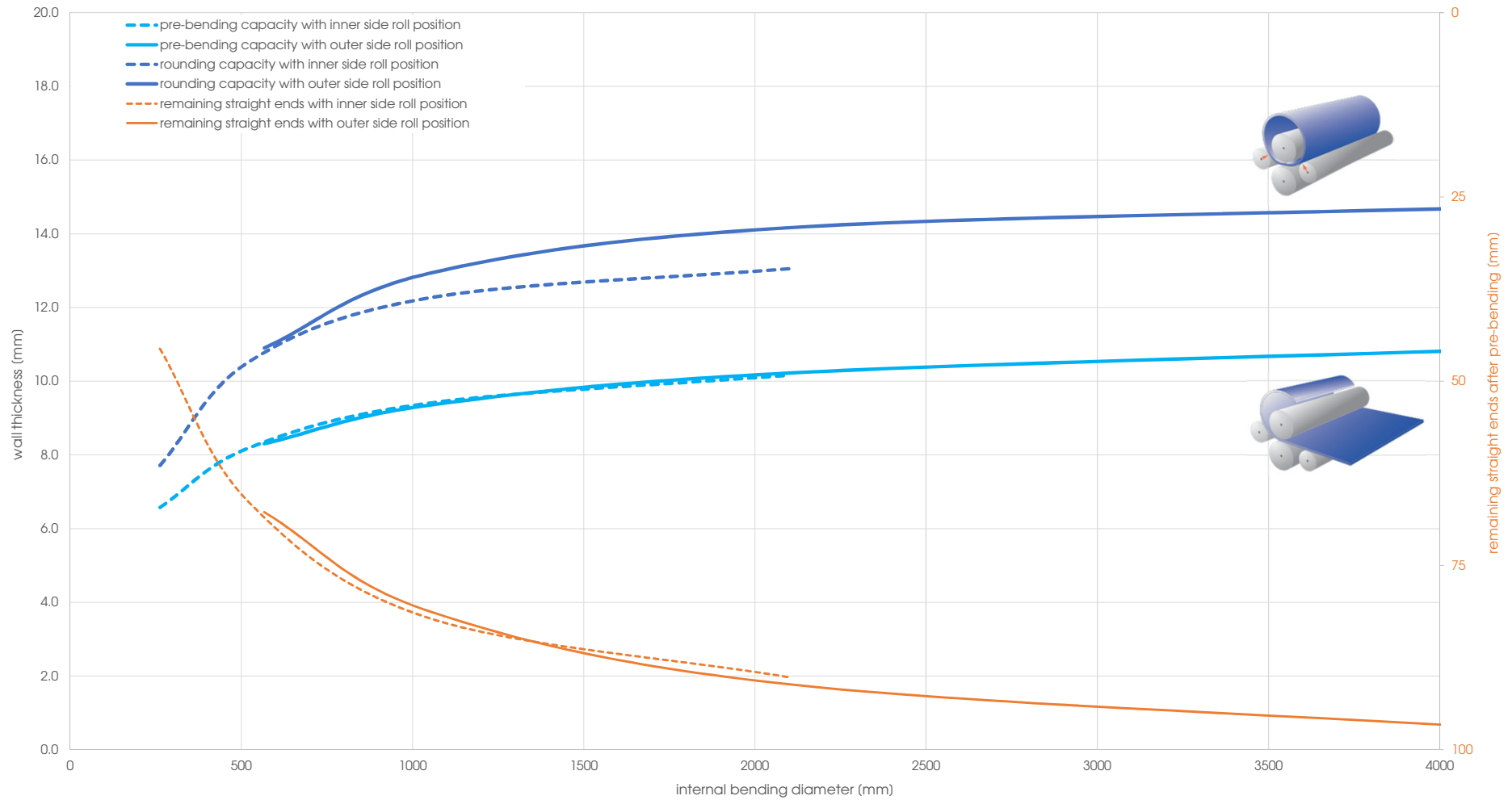
Capacity graph EVO 21015 - Yield point 260 N/mm 2 (calculated plate width 2'000 mm)
