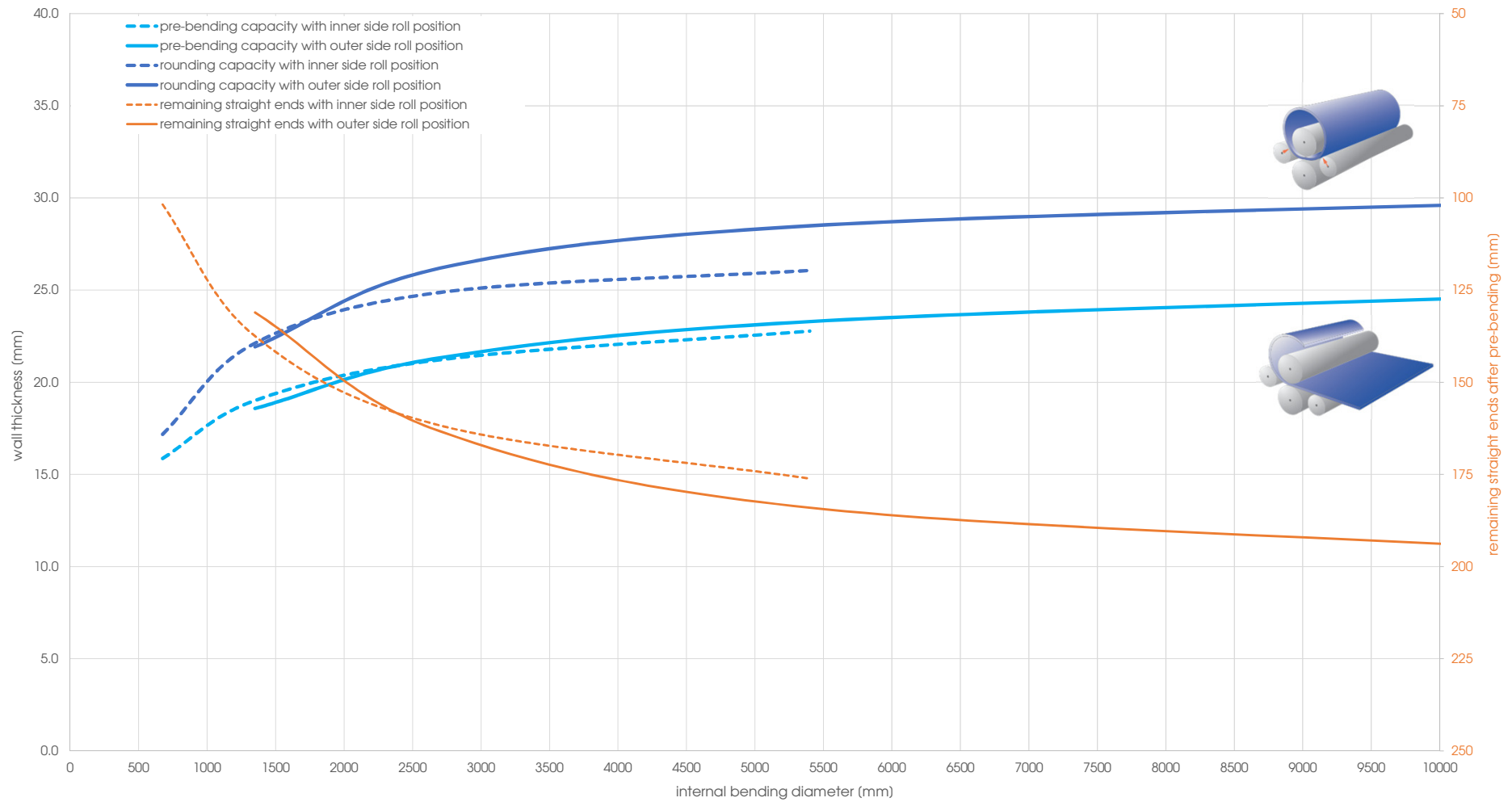
Capacity graph EVO 41196 - Yield point 690 N/mm 2 (calculated plate width 4'000 mm)
