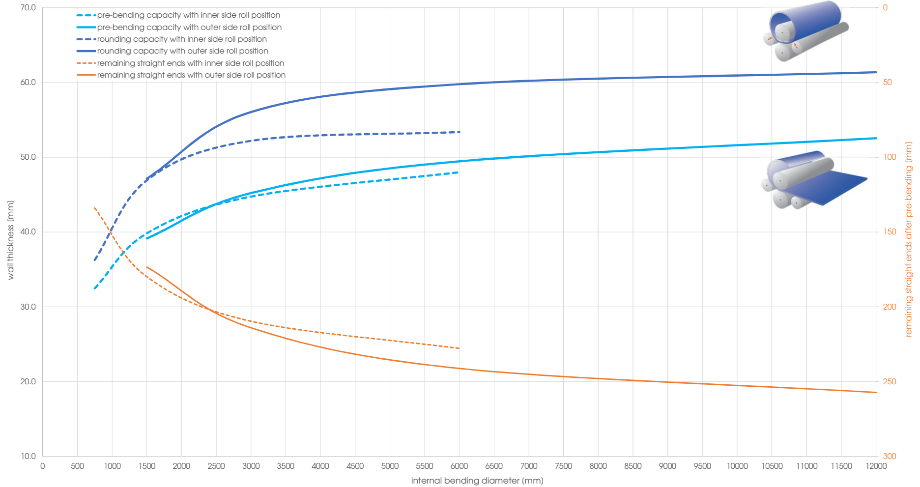
Capacity graph EVO 41283 - Yield point 260 N/mm 2 (calculated plate width 4'000 mm)
