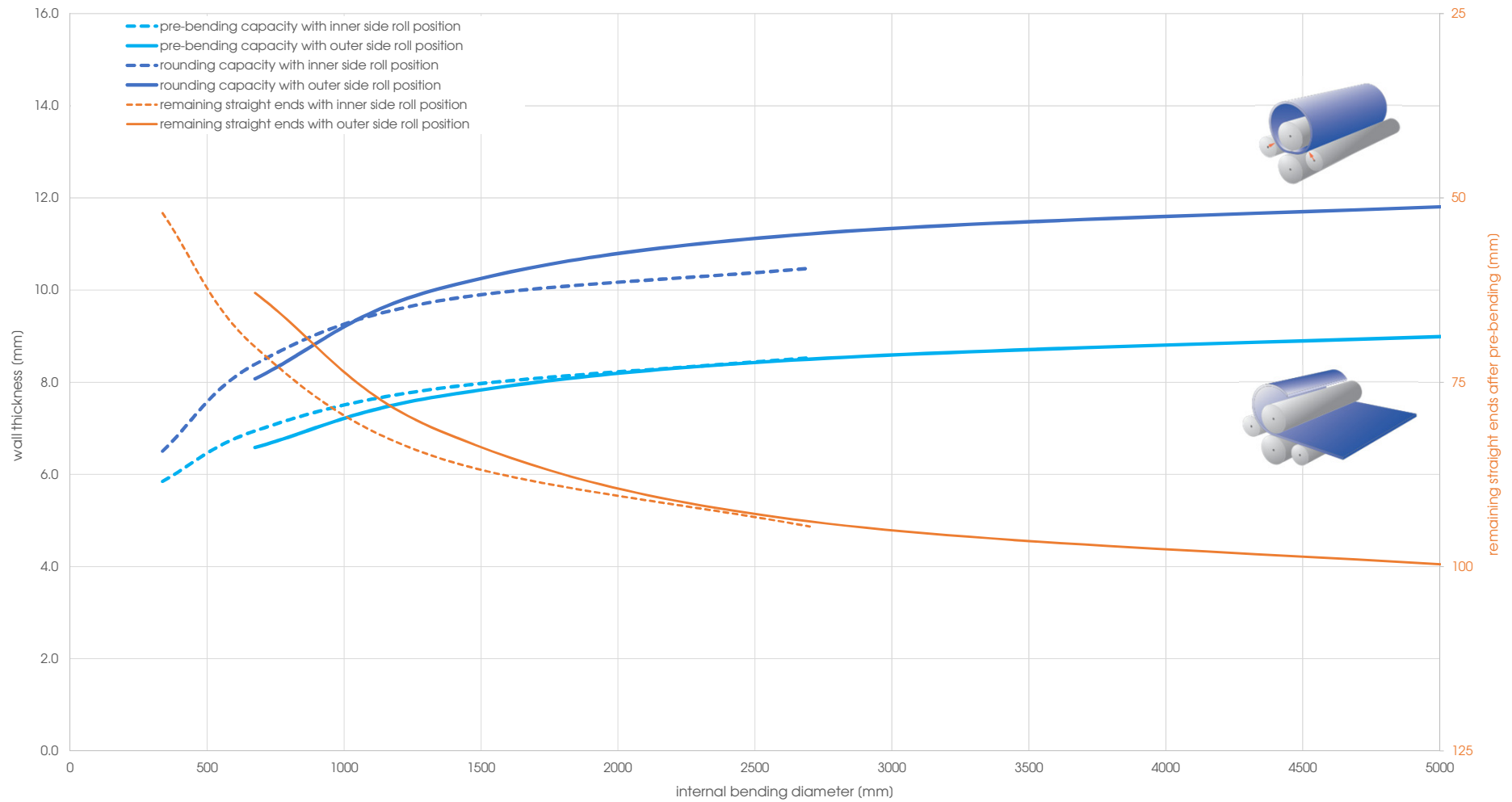
Capacity graph EVO 26031 - Yield point 690 N/mm 2 (calculated plate width 2'500 mm)
