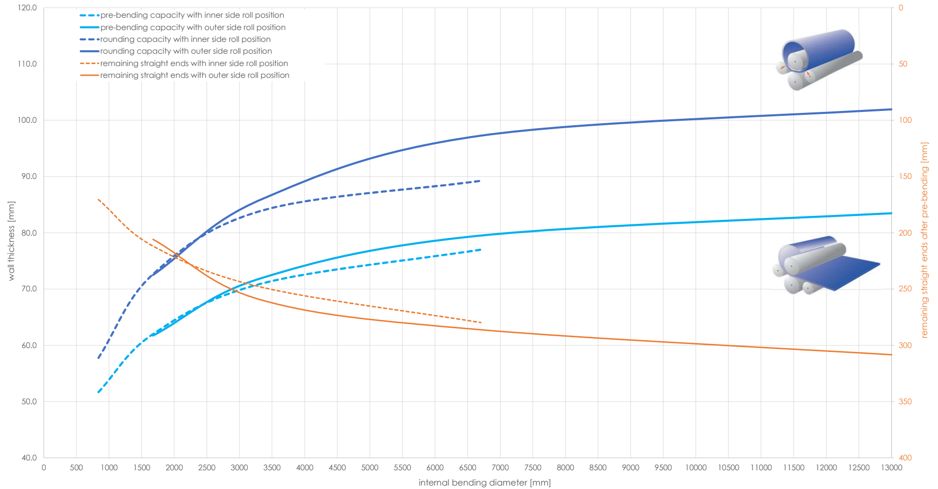
Capacity graph EVO 31513 - Yield point 260 N/mm 2 (calculated plate width 3'000 mm)
