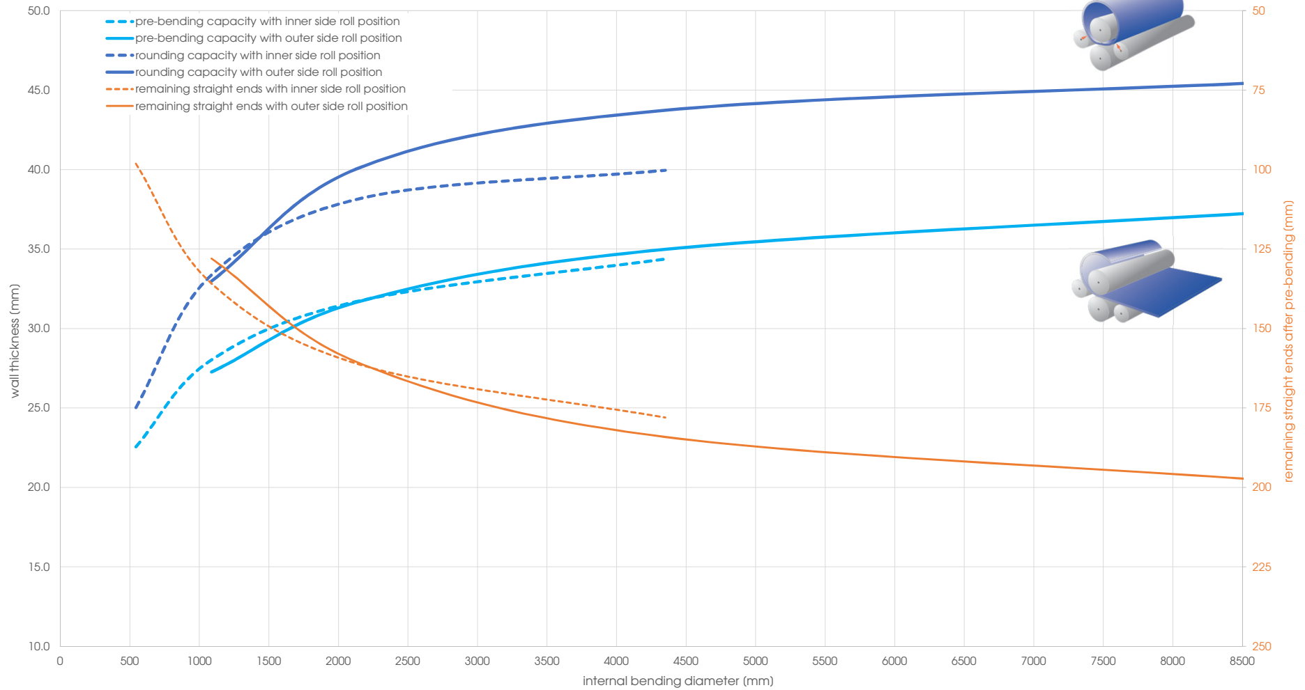
Capacity graph EVO 31139 - Yield point 260 N/mm 2 (calculated plate width 3'000 mm)
