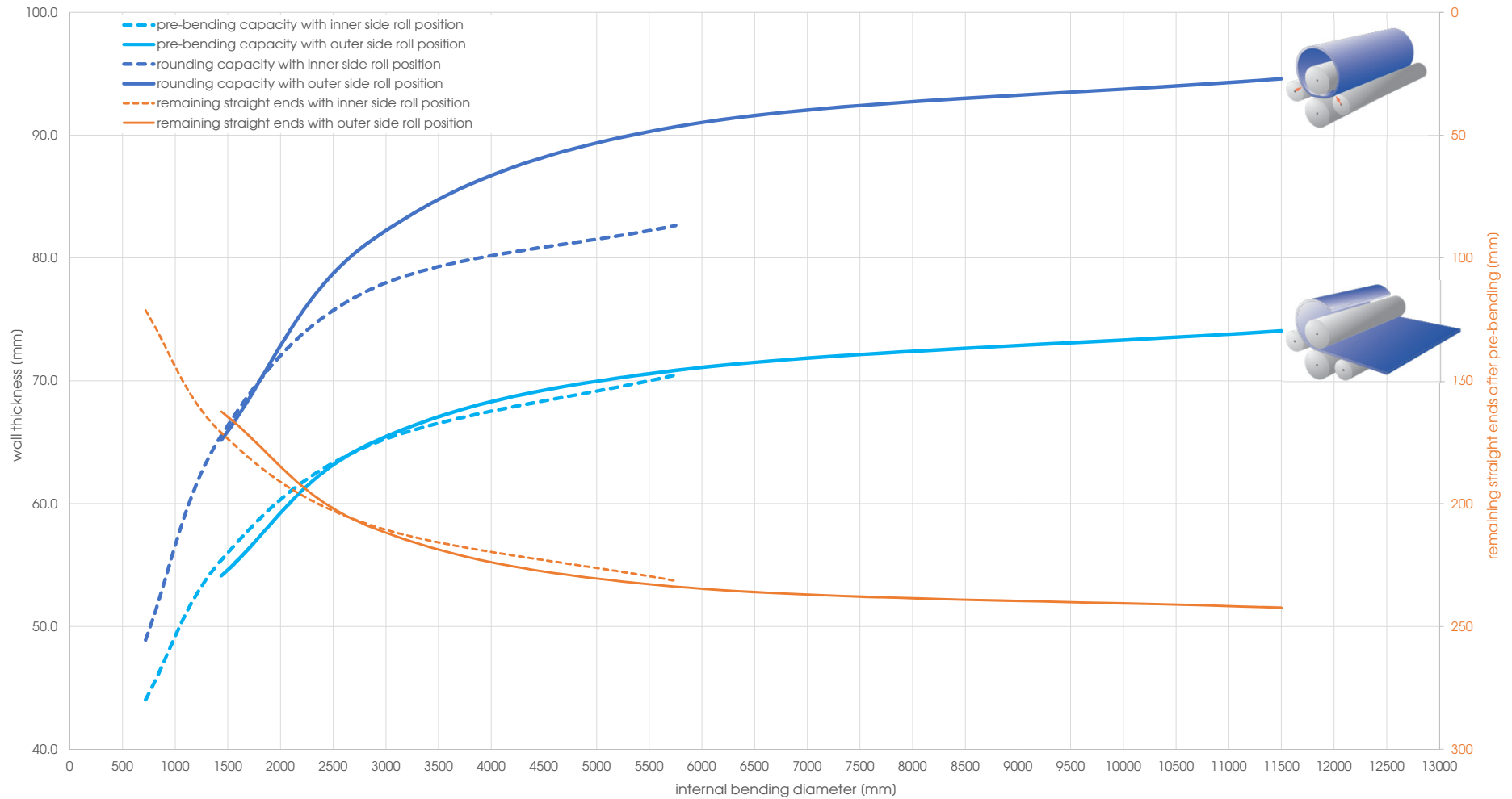
Capacity graph EVO 26385 - Yield point 260 N/mm 2 (calculated plate width 2'500 mm)
