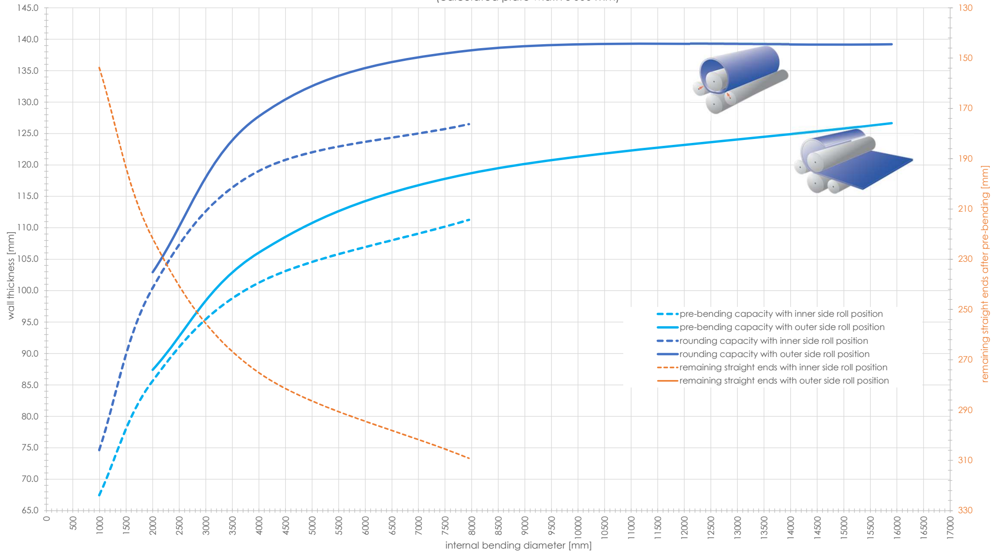
Capacity graph EVO 31871 - Yield point 260 N/mm 2 (calculated plate width 3'000 mm)
