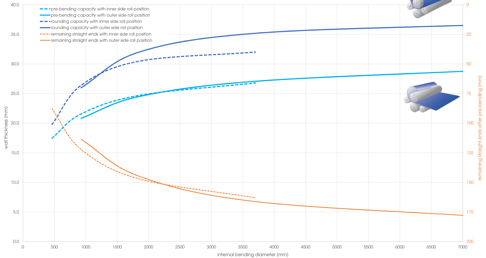
Capacity graph EVO 26102 - Yield point 360 N/mm 2 (calculated plate width 2'500 mm)
