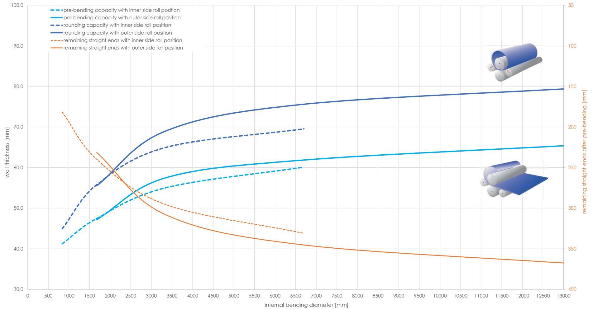
Capacity graph EVO 31513 - Yield point 450 N/mm 2 (calculated plate width 3'000 mm)
