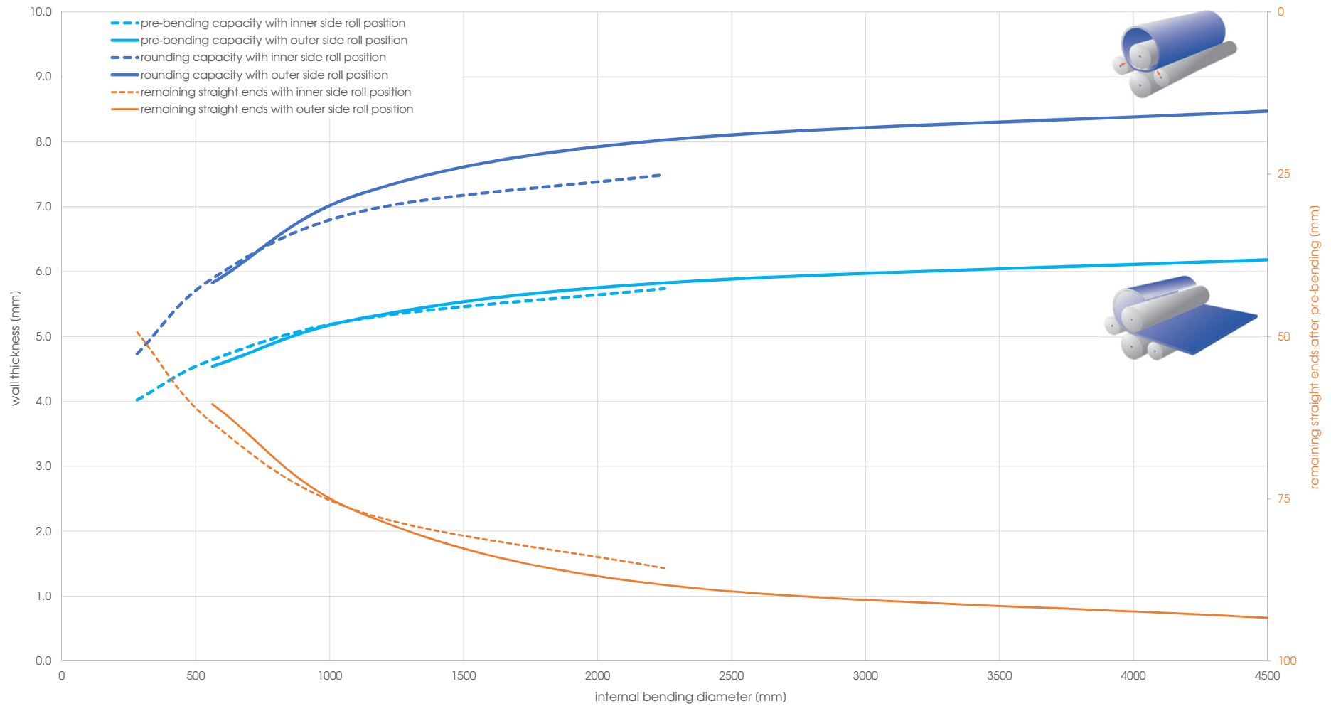
Capacity graph EVO 26015 - Yield point 690 N/mm 2 (calculated plate width 2'500 mm)
