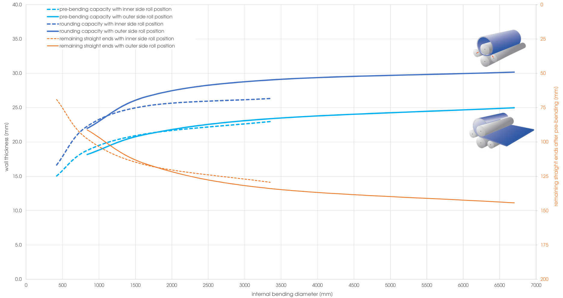
Capacity graph EVO 26071 - Yield point 260 N/mm 2 (calculated plate width 2'500 mm)
