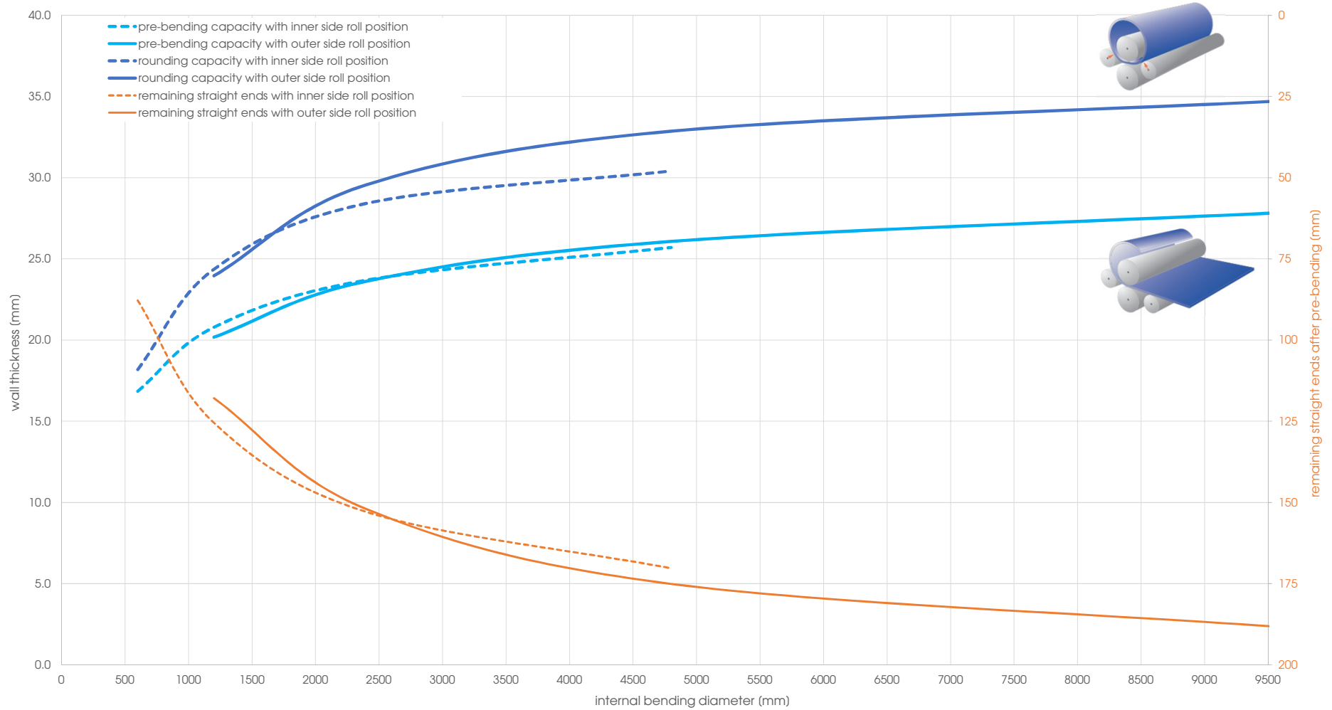
Capacity graph EVO 31196 - Yield point 690 N/mm 2 (calculated plate width 3'000 mm)
