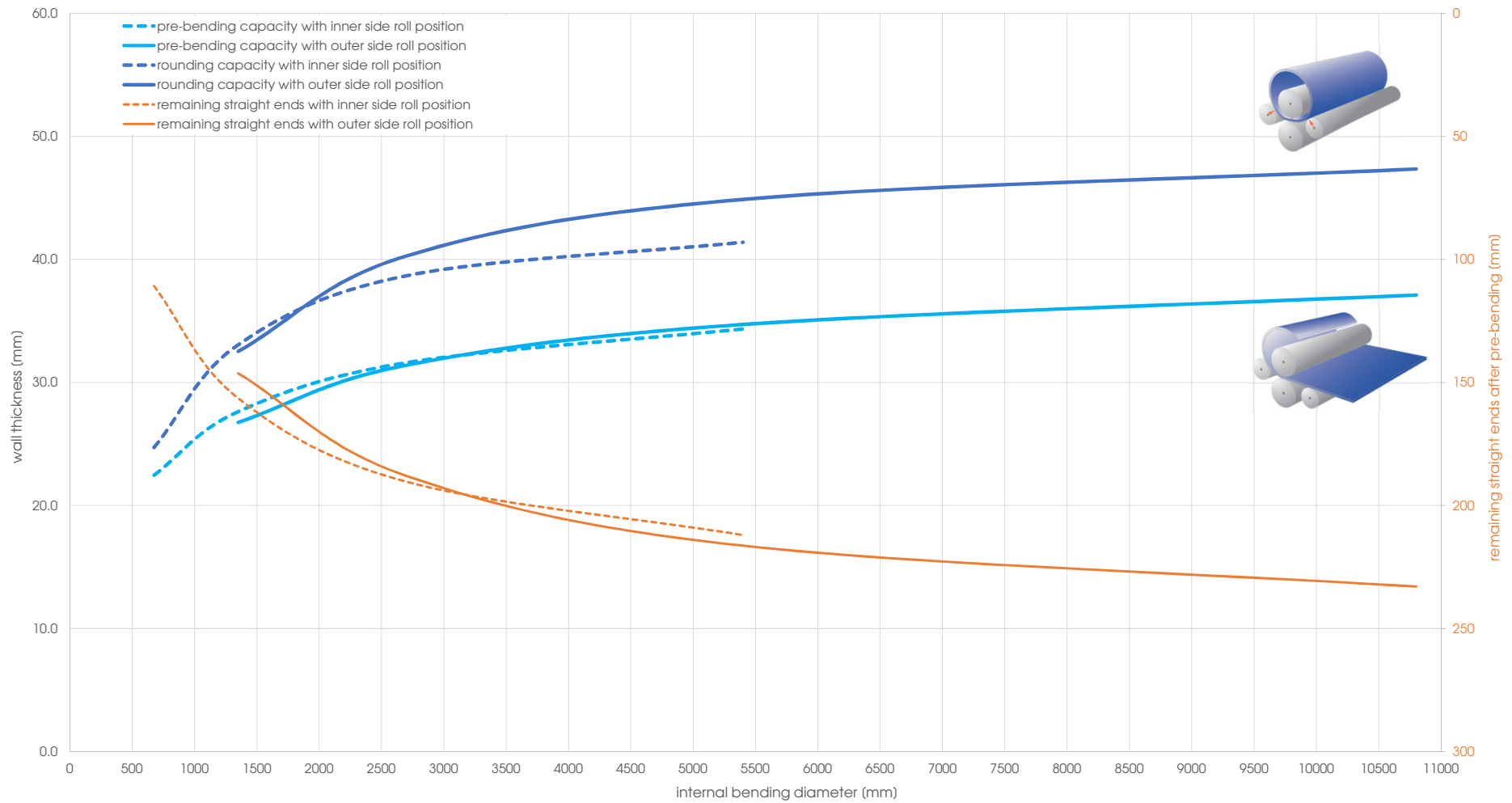
Capacity graph EVO 31283 - Yield point 690 N/mm 2 (calculated plate width 3'000 mm)
