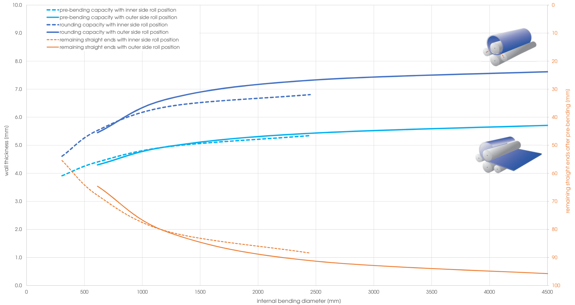
Capacity graph EVO 31015 - Yield point 690 N/mm 2 (calculated plate width 3'000 mm)
