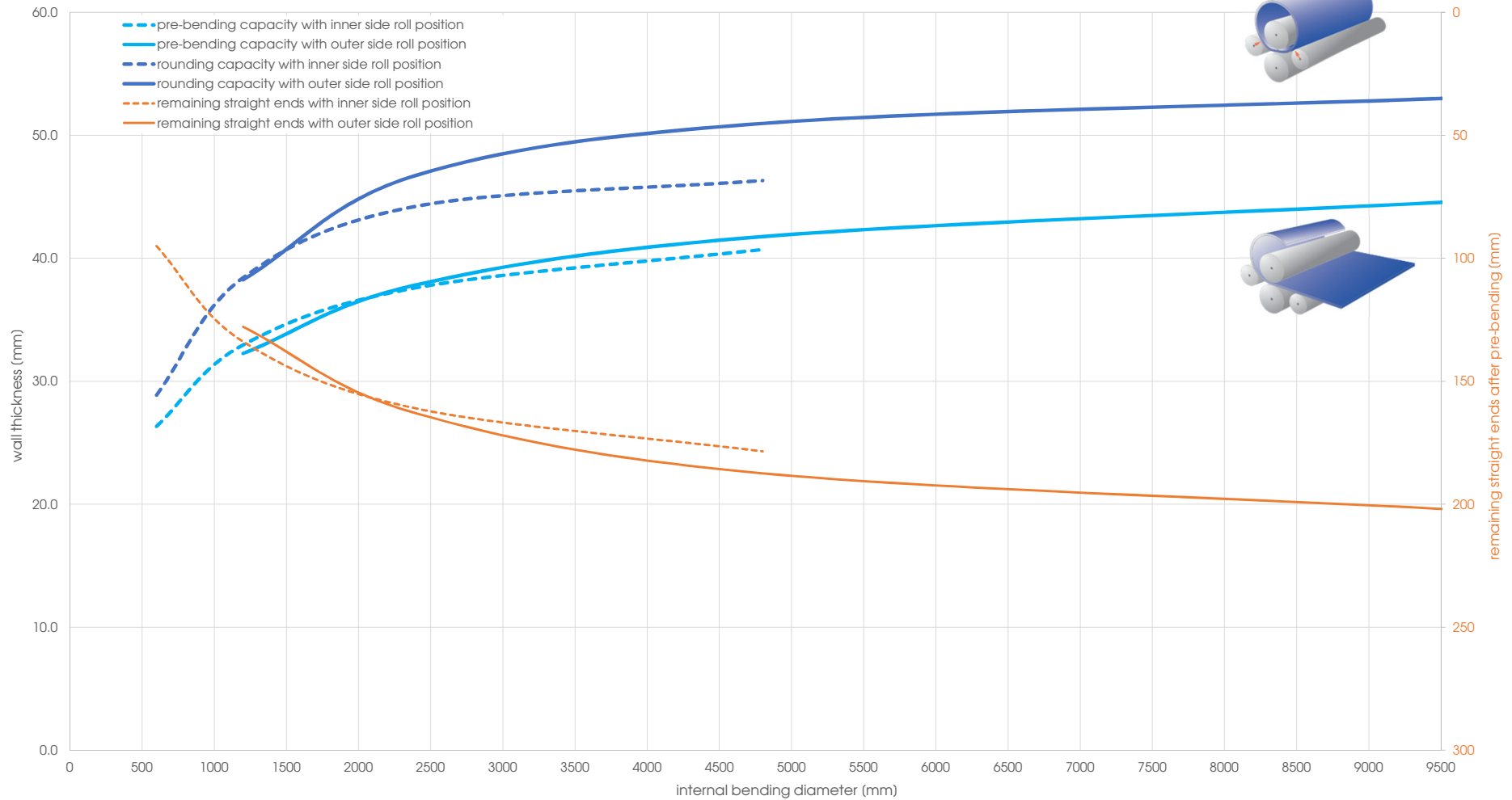
Capacity graph EVO 31196 - Yield point 260 N/mm 2 (calculated plate width 3'000 mm)
