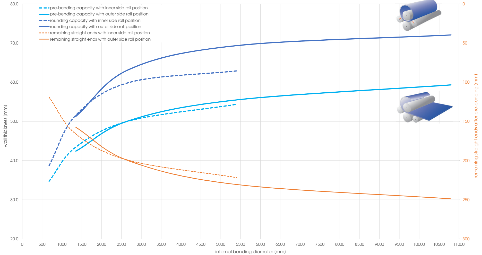
Capacity graph EVO 31283 - Yield point 260 N/mm 2 (calculated plate width 3'000 mm)
