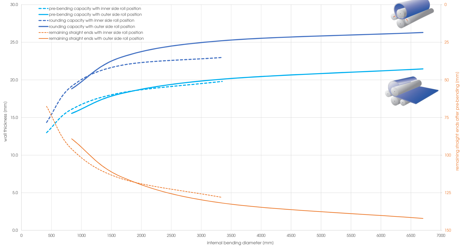
Capacity graph EVO 26071 - Yield point 360 N/mm 2 (calculated plate width 2'500 mm)
