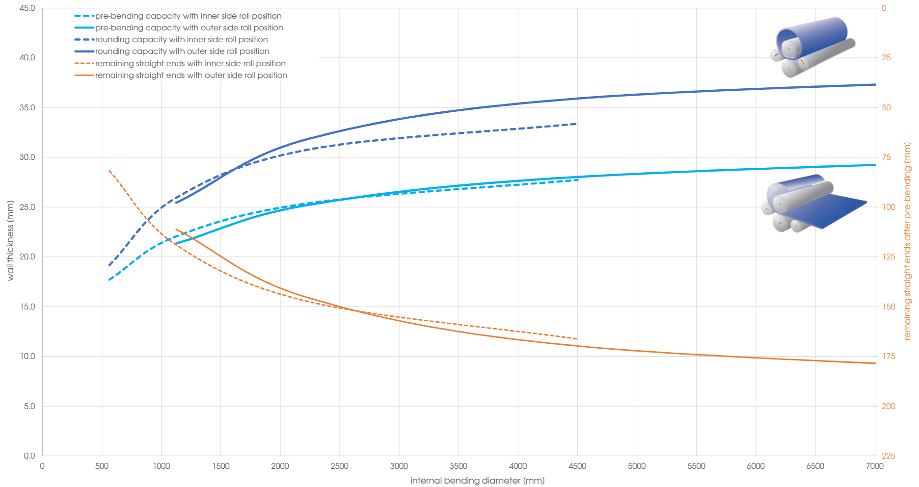
Capacity graph EVO 26196 - Yield point 690 N/mm 2 (calculated plate width 2'500 mm)
