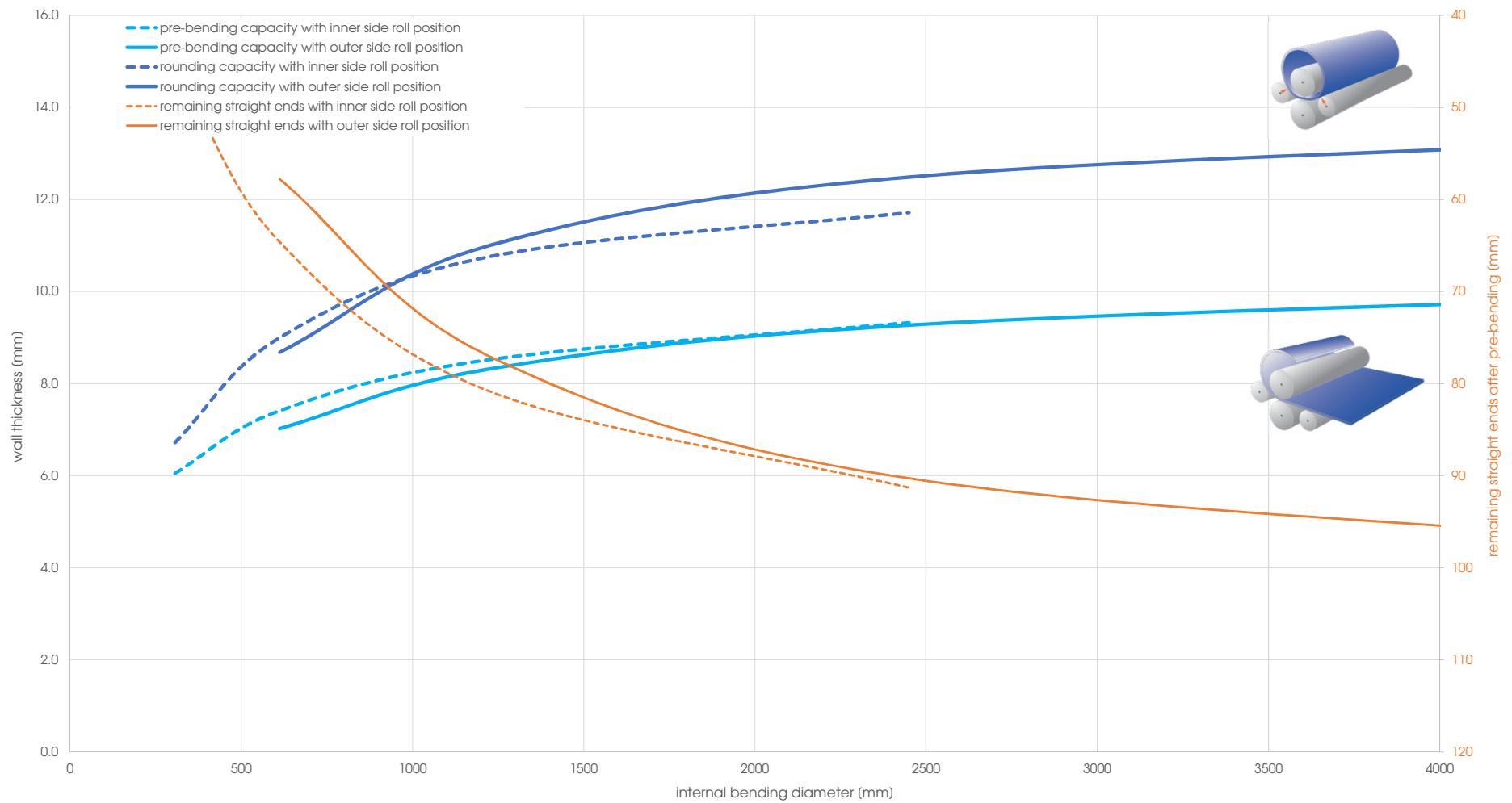
Capacity graph EVO 21031 - Yield point 690 N/mm 2 (calculated plate width 2'000 mm)
