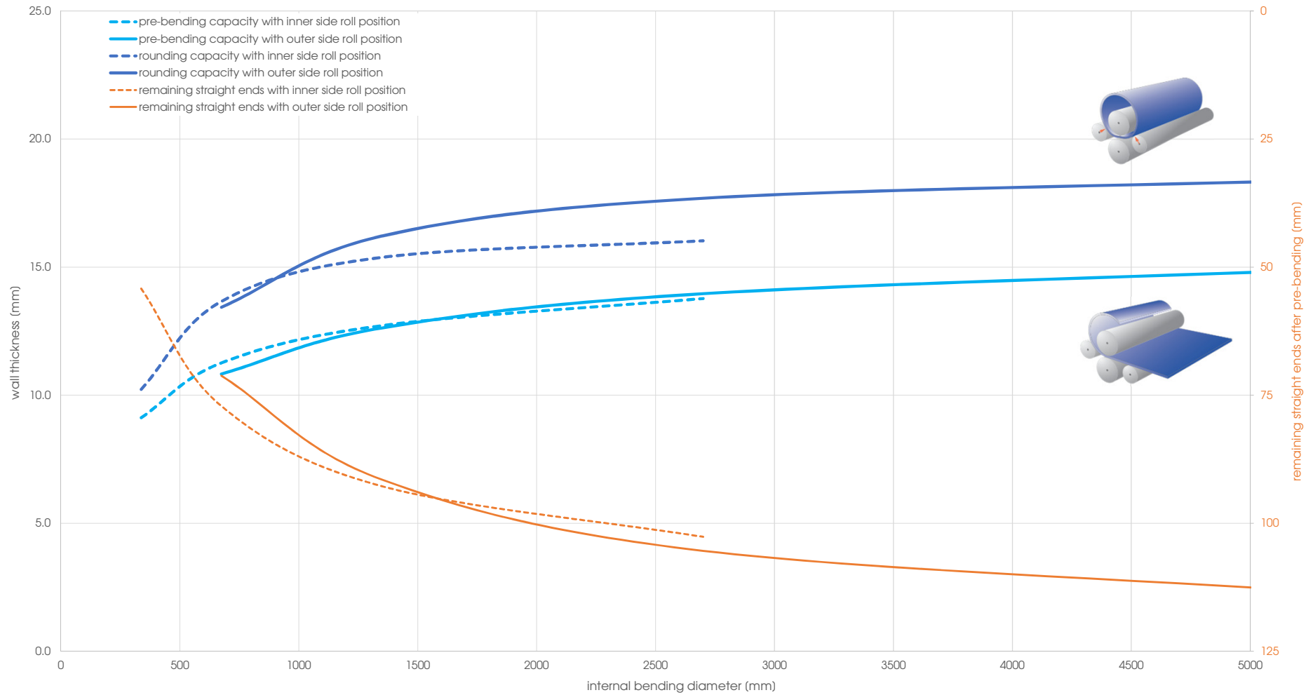
Capacity graph EVO 26031 - Yield point 260 N/mm 2 (calculated plate width 2'500 mm)
