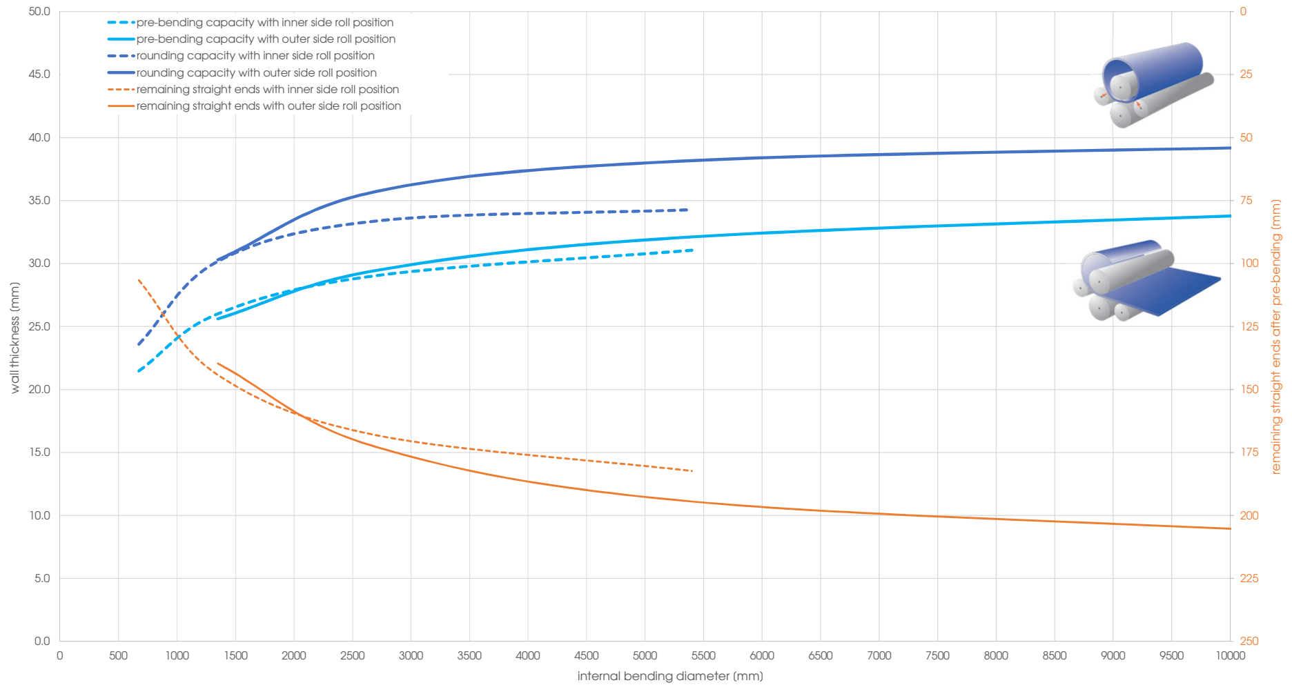
Capacity graph EVO 41196 - Yield point 360 N/mm 2 (calculated plate width 4'000 mm)
