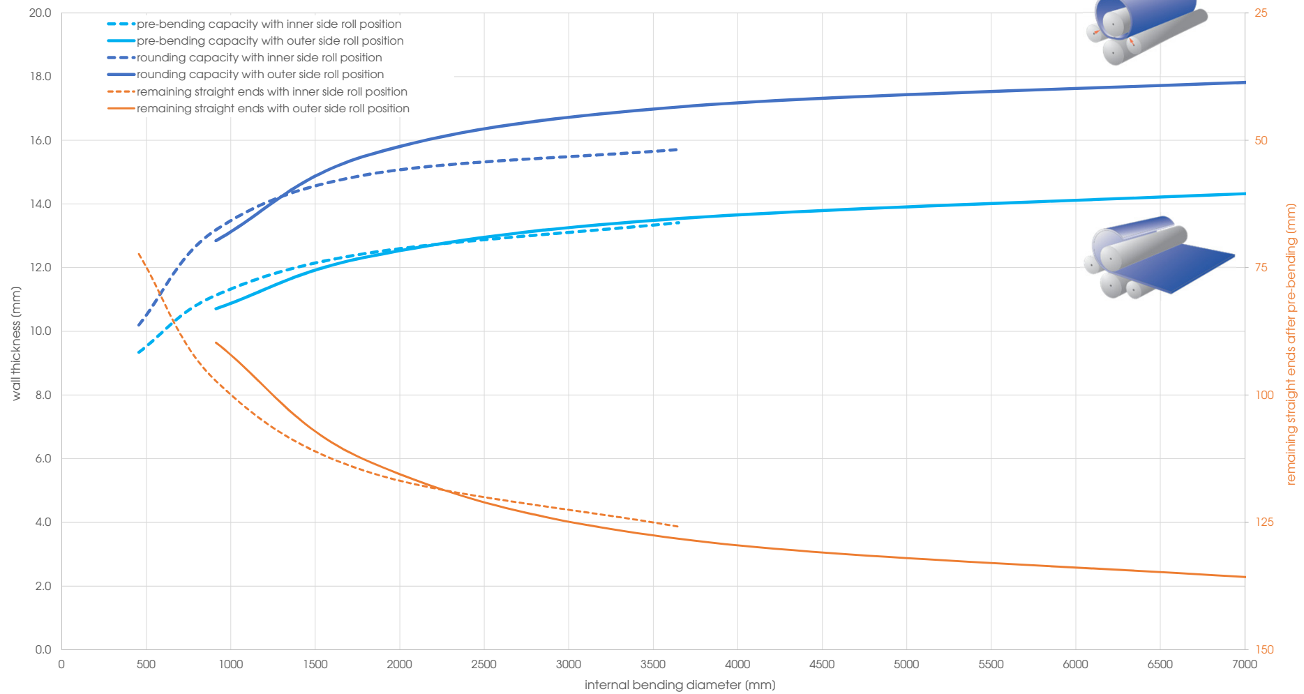
Capacity graph EVO 31071 - Yield point 690 N/mm 2 (calculated plate width 3'000 mm)
